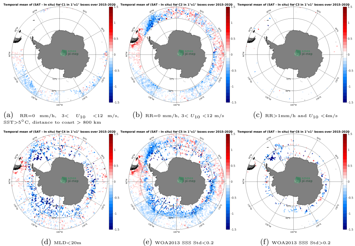
Figure 12: Temporal mean gridded over spatial boxes of size 1^{\circ}\times 1^{\circ} of \Delta\text{SSS} (SMAP SSS L3 v4 - Monthly (RSS) - Argo) for 6 different subdatasets corresponding to: \text{RR}=0 mm/h, 3 < U_{10} < 12 m/s, \text{SST}>5^{\circ}\text{C} , distance to coast > 800 km (a), \text{RR}=0 mm/h, 3 < U_{10} < 12 m/s (b), \text{RR}>1\text{mm/h} and U_{10} < 4\text{m/s} (c), \text{MLD}<20\text{m} (d), \text{WOA2013 SSS Std}<0.2 (e), \text{WOA2013 SSS Std}>0.2 (f).
