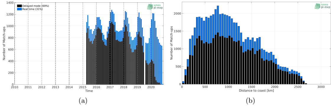
Figure 1: Number of match-ups between Argo and SMAP SSS L3 v4 - Monthly (RSS) SSS as a function of time (a) and as function of the distance to coast (b) over the Southern Ocean Pi-MEP region and for the full satellite product period.
