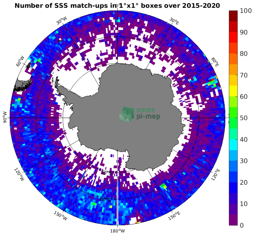
Figure 4: Number of SSS match-ups between Argo SSS and the SMAP SSS L3 v4 - Monthly (RSS) SSS product for the Southern Ocean Pi-MEP region over 1^\circ \times 1^\circ boxes and for the full satellite product period.
