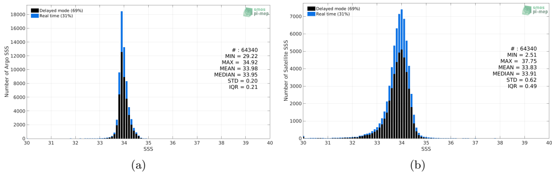
Figure 2: Histograms of SSS from Argo (a) and SMAP SSS L3 v4 - Monthly (RSS) (b) considering all match-up pairs per bins of 0.1 over the Southern Ocean Pi-MEP region and for the full satellite product period.
