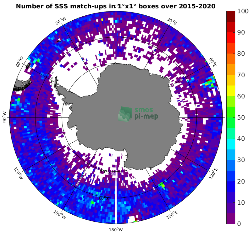
Figure 4: Number of SSS match-ups between Argo SSS and the SMAP-L3-RSS-V4-MONTHLY SSS product for the Southern Ocean Pi-MEP region over 1°x1° boxes and for the full satellite product period.
