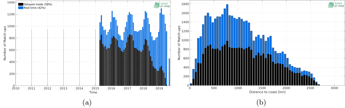
Figure 1: Number of match-ups between Argo and SMAP-L3-RSS-V4-MONTHLY SSS as a function of time (a) and as function of the distance to coast (b) over the Southern Ocean Pi-MEP region and for the full satellite product period.
