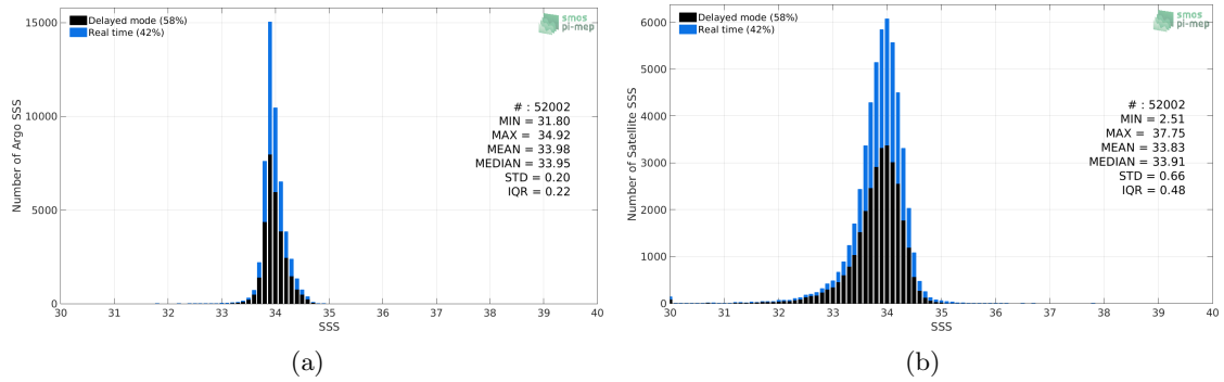
Figure 2: Histograms of SSS from Argo (a) and SMAP-L3-RSS-V4-MONTHLY (b) considering all match-up pairs per bins of 0.1 over the Southern Ocean Pi-MEP region and for the full satellite product period.
