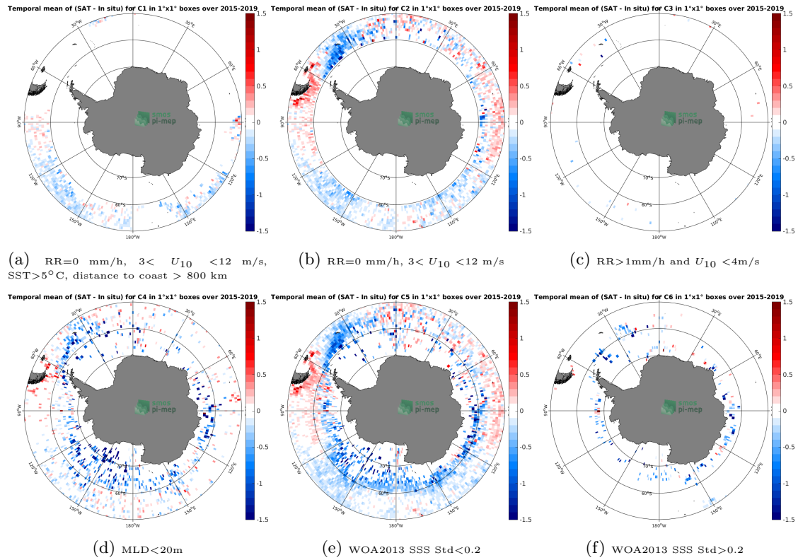
Figure 12: Temporal mean gridded over spatial boxes of size 1^\circ \times 1^\circ of \Delta SSS (SMAP-L3-RSS-V4-MONTHLY - Argo) for 6 different subdatasets corresponding to:RR=0 mm/h, 3 < U_{10} < 12 m/s, SST > 5^\circ C, distance to coast > 800 km (a), RR=0 mm/h, 3 < U_{10} < 12 m/s (b), RR > 1 mm/h and U_{10} < 4 m/s (c),MLD < 20 m (d),WOA2013 SSS Std < 0.2 (e),WOA2013 SSS Std > 0.2 (f).
