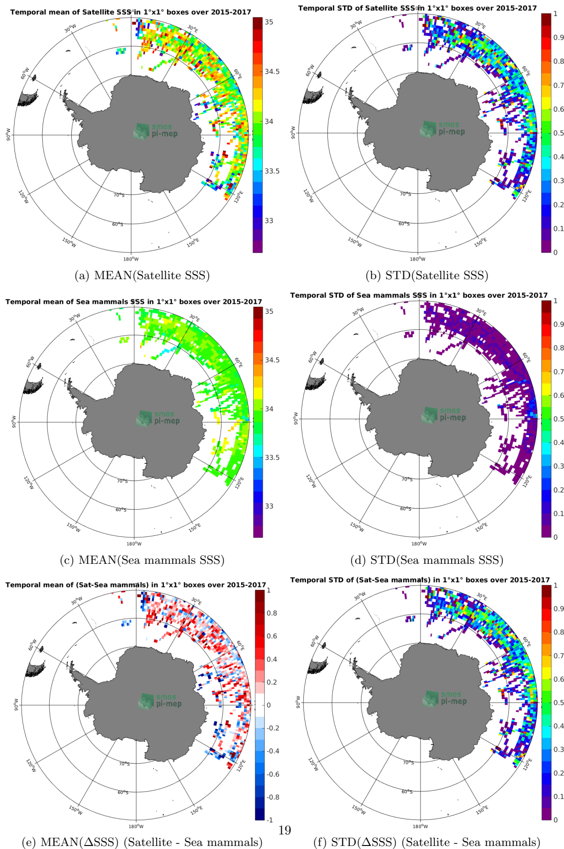
Figure 6: Temporal mean (left) and STD (right) of SSS from SMAP-L3-RSS-V3-8DAY-RUNNING-70KM (top), Sea mammals (middle), and of \Delta SSS (Satellite - Sea mammals). Only match-up pairs are used to generate these maps.
