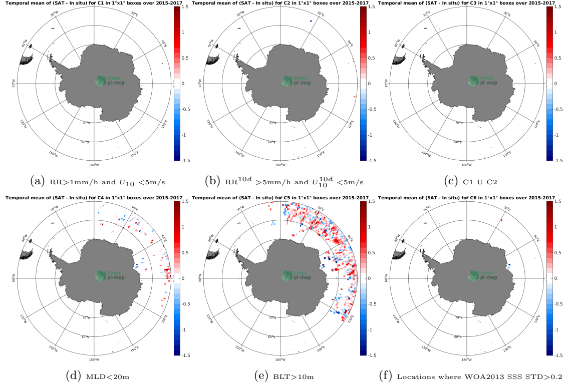
Figure 12: Temporal mean gridded over spatial boxes of size 1^\circ \times 1^\circ of \Delta\text{SSS} (SMAP-L3-RSS-V3-8DAY-RUNNING-70KM - Sea mammals) for 6 different subdatasets corresponding to: \text{RR} > 1\text{mm/h} and U_{10} < 5\text{m/s} (a), \text{RR}^{10d} > 5\text{mm/h} and U_{10}^{10d} < 5\text{m/s} (b), C1 U C2 (c), \text{MLD} < 20\text{m} (d), \text{BLT} > 10\text{m} (e), Locations where WOA2013 SSS STD > 0.2 (f).
