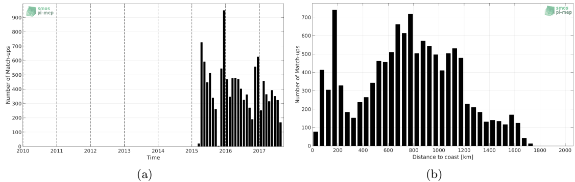
Figure 1: Number of match-ups between Sea mammals and SMAP-L3-RSS-V3-8DAY-RUNNING-70KM SSS as a function of time (a) and as function of the distance to coast (b) over the Southern Ocean Pi-MEP region and for the full satellite product period.
