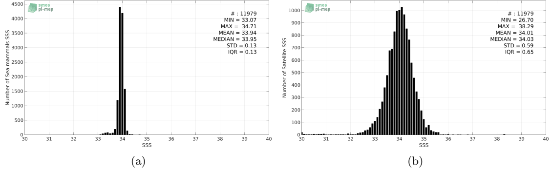
Figure 2: Histograms of SSS from Sea mammals (a) and SMAP-L3-RSS-V3-8DAY-RUNNING-70KM (b) considering all match-up pairs per bins of 0.1 over the Southern Ocean Pi-MEP region and for the full satellite product period.
