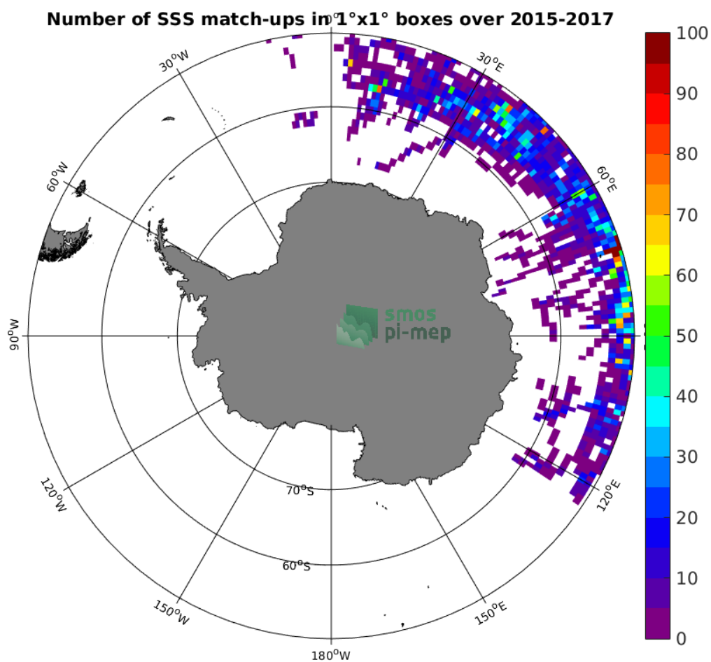
Figure 4: Number of SSS match-ups between Sea mammals SSS and the SMAP-L3-RSS-V3-8DAY-RUNNING-70KM SSS product for the Southern Ocean Pi-MEP region over 1^\circ \times 1^\circ boxes and for the full satellite product period.
