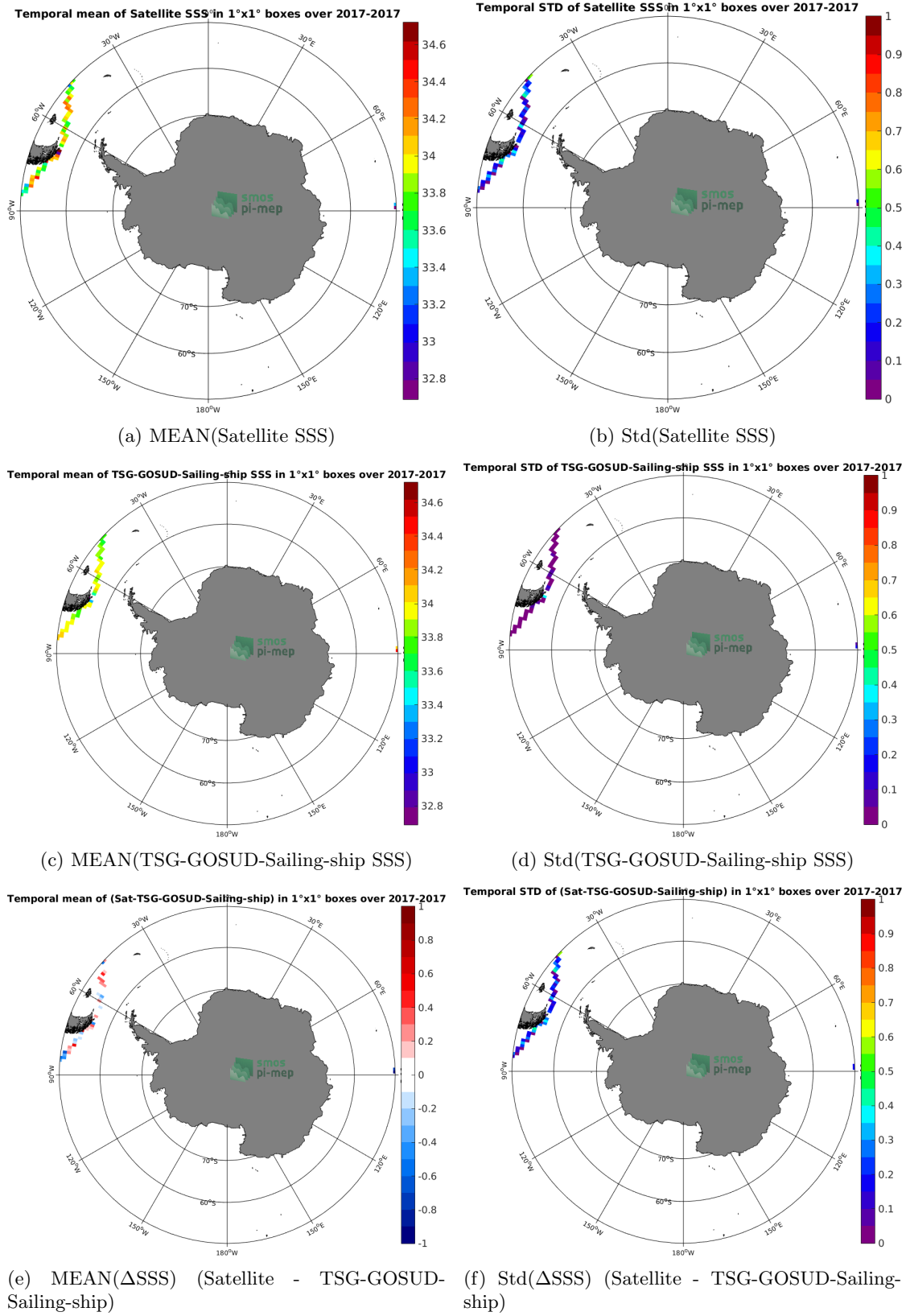
Figure 6: Temporal mean (left) and Std (right) of SSS from SMAP-L3-RSS-V3-8DAY-RUNNING-40KM (top), TSG-GOSUD-Sailing-ship (middle), and of \Delta SSS (Satellite - TSG-GOSUD-Sailing-ship). Only match-up pairs are used to generate these maps.
