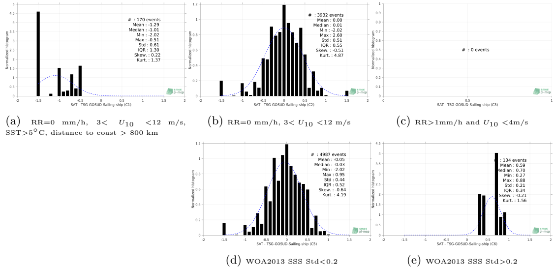
Figure 13: Normalized histogram of \Delta SSS (SMAP-L3-RSS-V3-8DAY-RUNNING-40KM - TSG-GOSUD-Sailing-ship) for 5 different subdatasets corresponding to: RR=0 mm/h, 3 < U_{10} < 12 m/s, SST>5°C, distance to coast > 800 km (a), RR=0 mm/h, 3 < U_{10} < 12 m/s (b), RR>1mm/h and U_{10} < 4 m/s (c), WOA2013 SSS Std<0.2 (d), WOA2013 SSS Std>0.2 (e).
