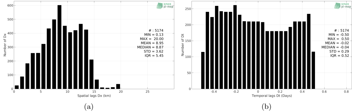
Figure 5: Histograms of the spatial (a) and temporal (b) lags between the time of the TSG-GOSUD-Sailing-ship measurements and the date of the corresponding SMAP-L3-RSS-V3-8DAY-RUNNING-40KM SSS product.
