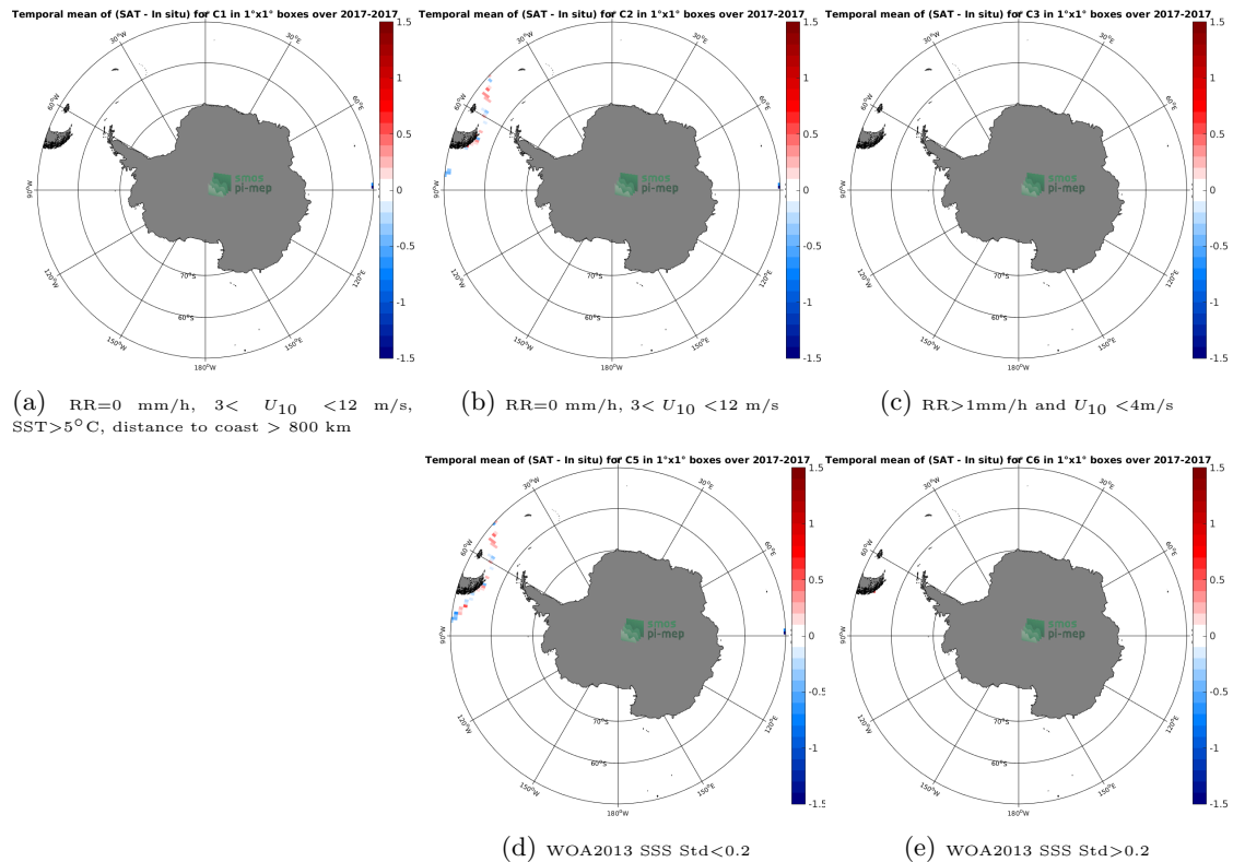
Figure 12: Temporal mean gridded over spatial boxes of size 1^\circ \times 1^\circ of \Delta SSS (SMAP-L3-RSS-V3-8DAY-RUNNING-40KM - TSG-GOSUD-Sailing-ship) for 5 different subdatasets corresponding to:RR=0 mm/h, 3 < U_{10} < 12 m/s, SST >5^\circ C, distance to coast > 800 km (a), RR=0 mm/h, 3 < U_{10} < 12 m/s (b), RR >1 mm/h and U_{10} < 4 m/s (c), WOA2013 SSS Std <0.2 (d), WOA2013 SSS Std >0.2 (e).
