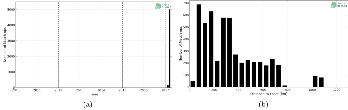
Figure 1: Number of match-ups between TSG-GOSUD-Sailing-ship and SMAP-L3-RSS-V3-8DAY-RUNNING-40KM SSS as a function of time (a) and as function of the distance to coast (b) over the Southern Ocean Pi-MEP region and for the full satellite product period.
