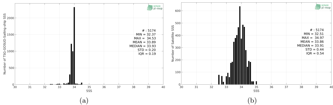
Figure 2: Histograms of SSS from TSG-GOSUD-Sailing-ship (a) and SMAP-L3-RSS-V3-8DAY-RUNNING-40KM (b) considering all match-up pairs per bins of 0.1 over the Southern Ocean Pi-MEP region and for the full satellite product period.
