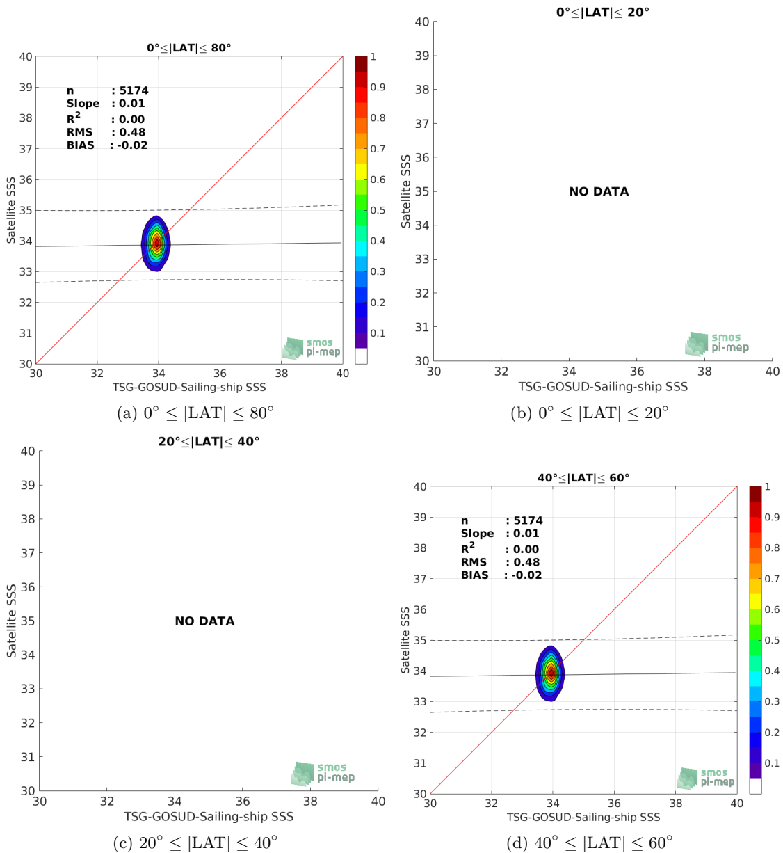
Figure 9: Contour maps of the concentration of SMAP-L3-RSS-V3-8DAY-RUNNING-40KM SSS (y-axis) versus TSG-GOSUD-Sailing-ship SSS (x-axis) at match-up pairs for different latitude bands. For each plot, the red line shows x=y . The black thin and dashed lines indicate a linear fit through the data cloud and the \pm 95\% confidence levels, respectively. The number match-up pairs n , the slope and R^2 coefficient of the linear fit, the root mean square (RMS) and the mean bias between satellite and in situ data are indicated for each latitude band in each plots.
