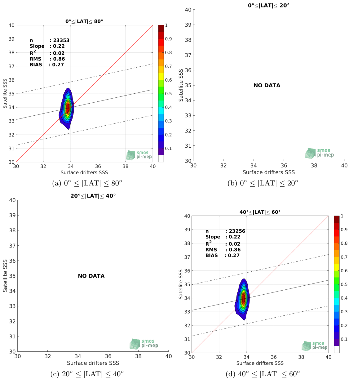
Figure 8: Contour maps of the concentration of SMAP-L3-RSS-V3-8DAY-RUNNING-40KM SSS (y-axis) versus Surface drifters SSS (x-axis) at match-up pairs for different latitude bands. For each plot, the red line shows x=y . The black thin and dashed lines indicate a linear fit through the data cloud and the \pm 95\% confidence levels, respectively. The number match-up pairs n , the slope and R^2 coefficient of the linear fit, the root mean square (RMS) and the mean bias between satellite and in situ data are indicated for each latitude band in each plots.
