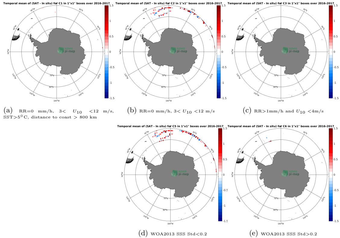
Figure 11: Temporal mean gridded over spatial boxes of size 1^\circ \times 1^\circ of \Delta SSS (SMAP-L3-RSS-V3-8DAY-RUNNING-40KM - Surface drifters) for 5 different subdatasets corresponding to:RR=0 mm/h, 3 < U_{10} < 12 m/s, SST >5^\circ C, distance to coast > 800 km (a), RR=0 mm/h, 3 < U_{10} < 12 m/s (b), RR >1 mm/h and U_{10} < 4 m/s (c), WOA2013 SSS Std <0.2 (d), WOA2013 SSS Std >0.2 (e).
