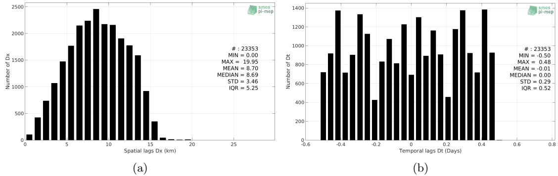
Figure 4: Histograms of the spatial (a) and temporal (b) lags between the time of the Surface drifters measurements and the date of the corresponding SMAP-L3-RSS-V3-8DAY-RUNNING-40KM SSS product.
