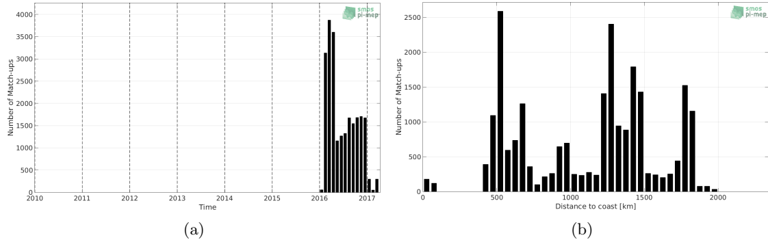
Figure 1: Number of match-ups between Surface drifters and SMAP-L3-RSS-V3-8DAY-RUNNING-40KM SSS as a function of time (a) and as function of the distance to coast (b) over the Southern Ocean Pi-MEP region and for the full satellite product period.
