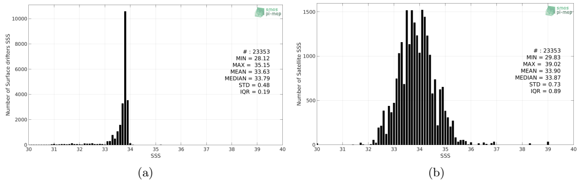
Figure 2: Histograms of SSS from Surface drifters (a) and SMAP-L3-RSS-V3-8DAY-RUNNING-40KM (b) considering all match-up pairs per bins of 0.1 over the Southern Ocean Pi-MEP region and for the full satellite product period.
