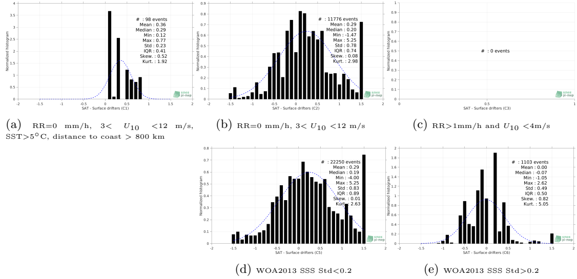
Figure 12: Normalized histogram of \Delta SSS (SMAP-L3-RSS-V3-8DAY-RUNNING-40KM - Surface drifters) for 5 different subdatasets corresponding to: RR=0 mm/h, 3 < U_{10} < 12 m/s, SST>5°C, distance to coast > 800 km (a), RR=0 mm/h, 3 < U_{10} < 12 m/s (b), RR>1mm/h and U_{10} < 4 m/s (c), WOA2013 SSS Std<0.2 (d), WOA2013 SSS Std>0.2 (e).
