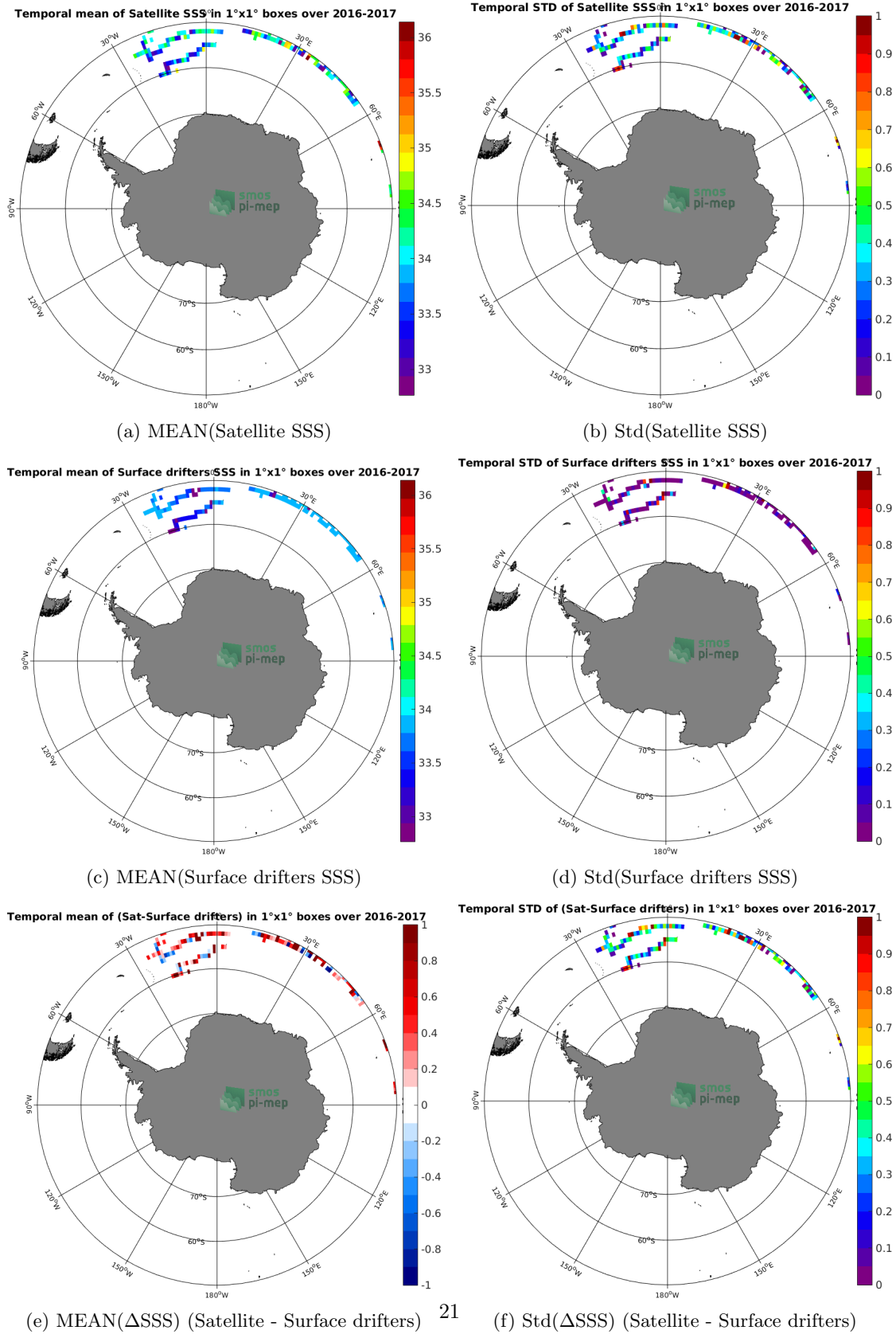
Figure 5: Temporal mean (left) and Std (right) of SSS from SMAP-L3-RSS-V3-8DAY-RUNNING-40KM (top), Surface drifters (middle), and of \Delta SSS (Satellite - Surface drifters). Only match-up pairs are used to generate these maps.
