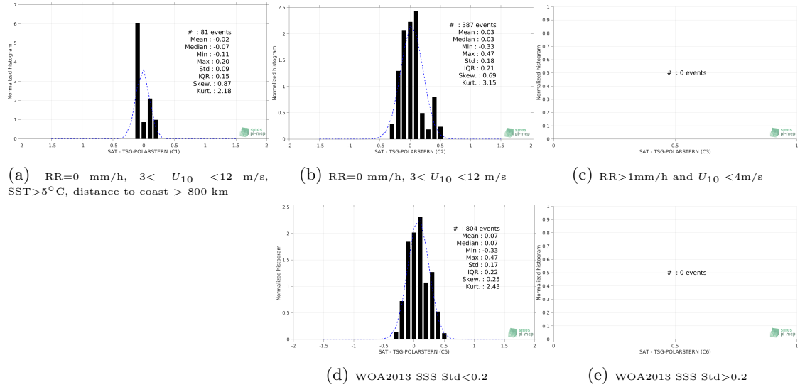
Figure 13: Normalized histogram of \Delta\text{SSS} (SMAP-L3-RSS-V3-MONTHLY-70KM - TSG-POLARSTERN) for 5 different subdatasets corresponding to: RR=0 mm/h, 3 < U_{10} < 12 m/s, SST >5^{\circ}\text{C} , distance to coast > 800 km (a), RR=0 mm/h, 3 < U_{10} < 12 m/s (b), RR >1\text{mm/h} and U_{10} < 4\text{m/s} (c), WOA2013 SSS Std <0.2 (d), WOA2013 SSS Std >0.2 (e).
