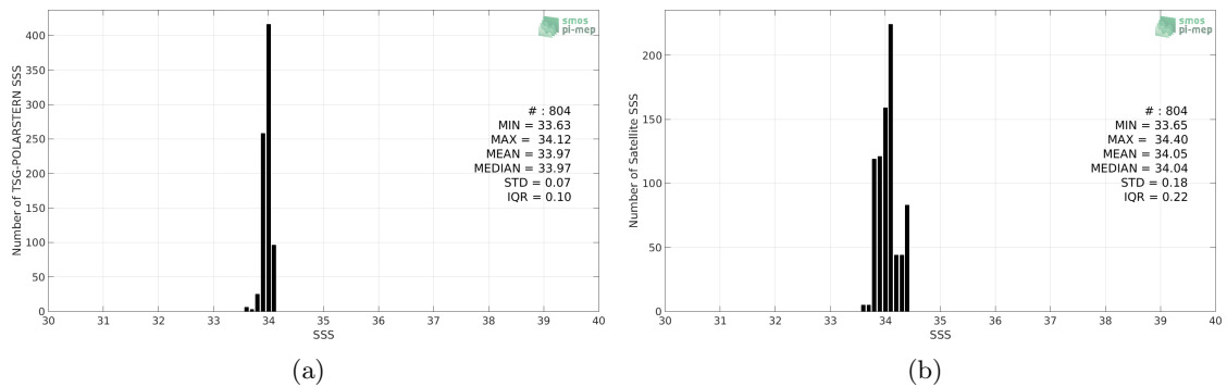
Figure 2: Histograms of SSS from TSG-POLARSTERN (a) and SMAP-L3-RSS-V3-MONTHLY-70KM (b) considering all match-up pairs per bins of 0.1 over the Southern Ocean Pi-MEP region and for the full satellite product period.
