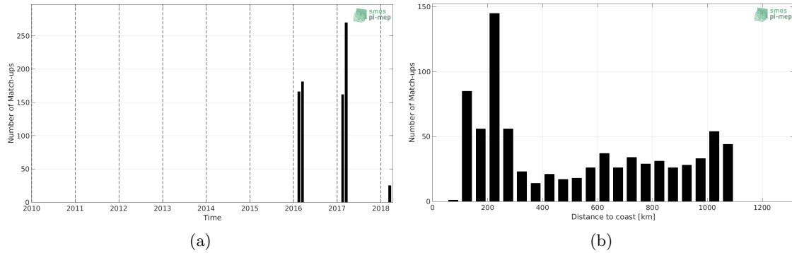
Figure 1: Number of match-ups between TSG-POLARSTERN and SMAP-L3-RSS-V3-MONTHLY-70KM SSS as a function of time (a) and as function of the distance to coast (b) over the Southern Ocean Pi-MEP region and for the full satellite product period.
