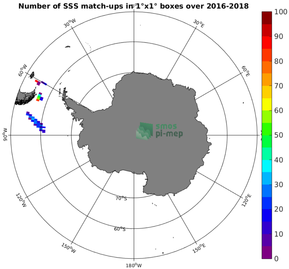
Figure 4: Number of SSS match-ups between TSG-POLARSTERN SSS and the SMAP-L3-RSS-V3-MONTHLY-70KM SSS product for the Southern Ocean Pi-MEP region over 1°x1° boxes and for the full satellite product period.
