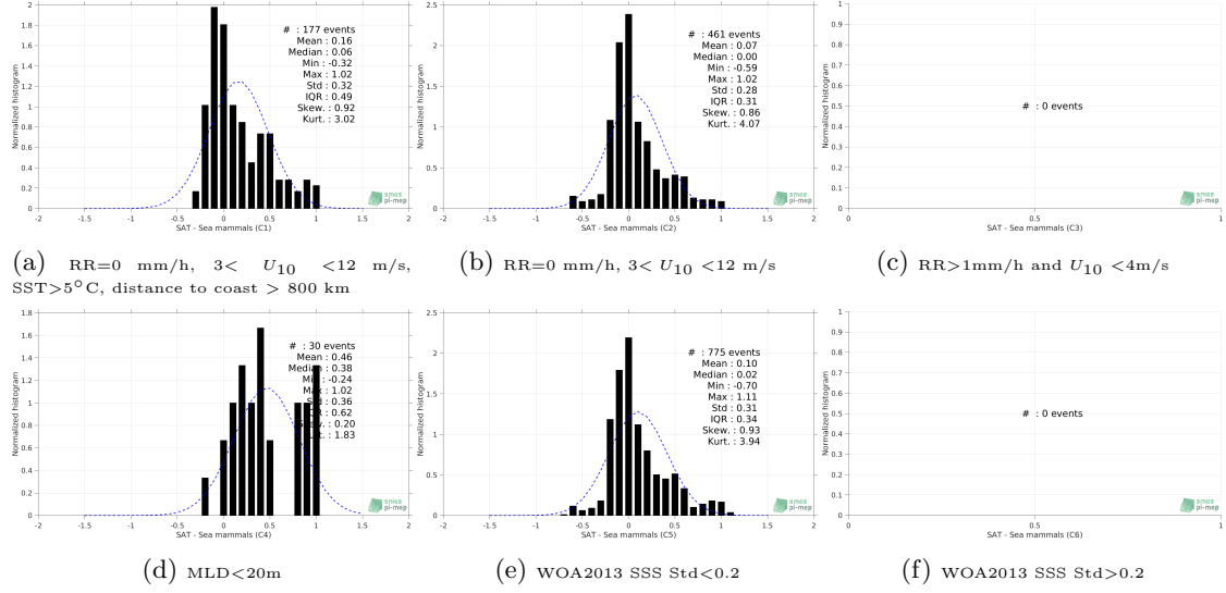
Figure 13: Normalized histogram of \Delta\text{SSS} (SMAP-L3-RSS-V3-MONTHLY-70KM - Sea mammals) for 6 different subdatasets corresponding to: RR=0 mm/h, 3 < U_{10} < 12 m/s, SST > 5^\circ\text{C} , distance to coast > 800 km (a), RR=0 mm/h, 3 < U_{10} < 12 m/s (b), RR > 1\text{mm/h} and U_{10} < 4\text{m/s} (c), MLD < 20\text{m} (d), WOA2013 SSS Std < 0.2 (e), WOA2013 SSS Std > 0.2 (f).
