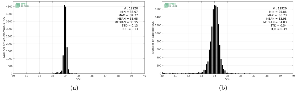
Figure 2: Histograms of SSS from Sea mammals (a) and SMAP-L3-RSS-V3-MONTHLY-70KM (b) considering all match-up pairs per bins of 0.1 over the Southern Ocean Pi-MEP region and for the full satellite product period.
