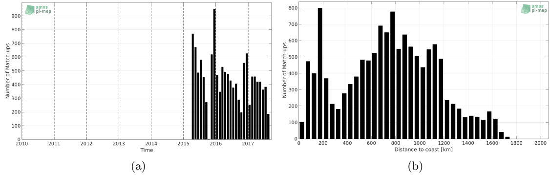
Figure 1: Number of match-ups between Sea mammals and SMAP-L3-RSS-V3-MONTHLY-70KM SSS as a function of time (a) and as function of the distance to coast (b) over the Southern Ocean Pi-MEP region and for the full satellite product period.
