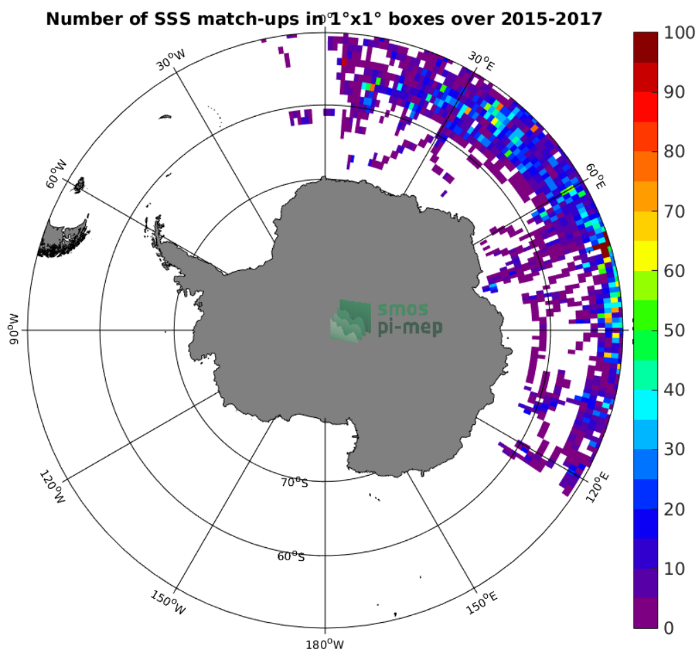
Figure 4: Number of SSS match-ups between Sea mammals SSS and the SMAP-L3-RSS-V3-MONTHLY-70KM SSS product for the Southern Ocean Pi-MEP region over 1^\circ \times 1^\circ boxes and for the full satellite product period.
