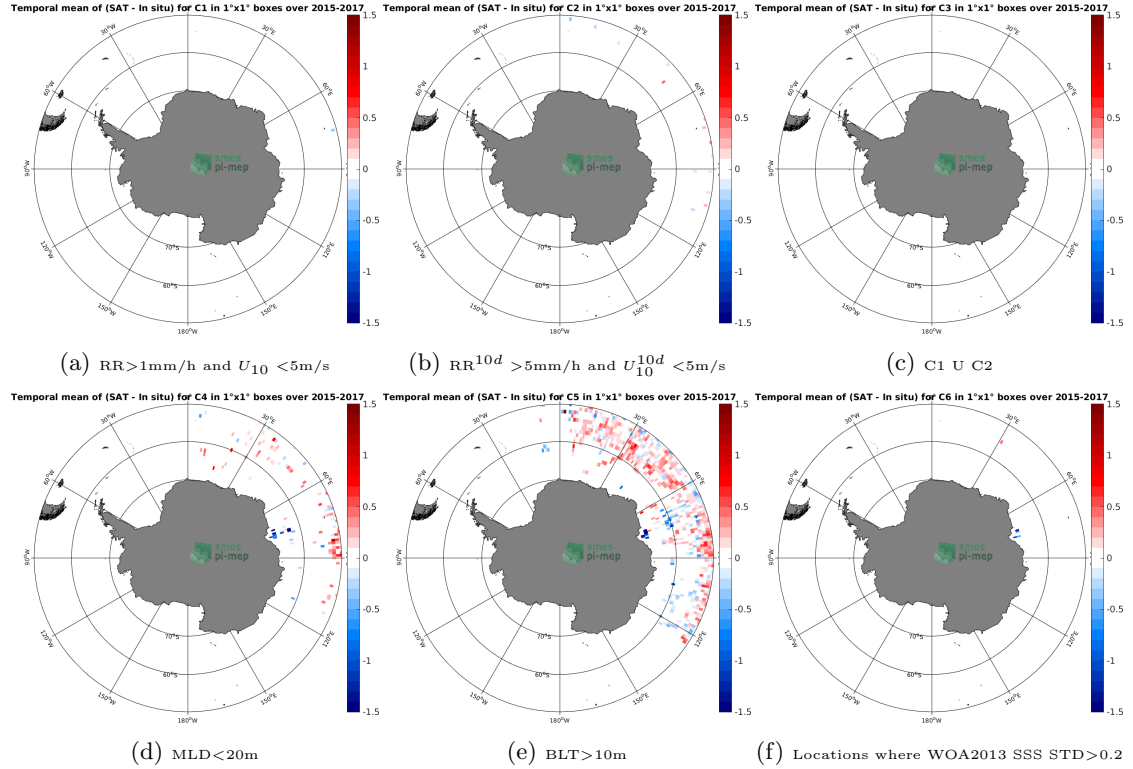
Figure 12: Temporal mean gridded over spatial boxes of size 1^\circ \times 1^\circ of \Delta\text{SSS} (SMAP-L3-RSS-V3-MONTHLY-70KM - Sea mammals) for 6 different subdatasets corresponding to: \text{RR} > 1\text{mm/h} and U_{10} < 5\text{m/s} (a), \text{RR}^{10d} > 5\text{mm/h} and U_{10}^{10d} < 5\text{m/s} (b), C1 U C2 (c), \text{MLD} < 20\text{m} (d), \text{BLT} > 10\text{m} (e), Locations where WOA2013 SSS STD > 0.2 (f).
