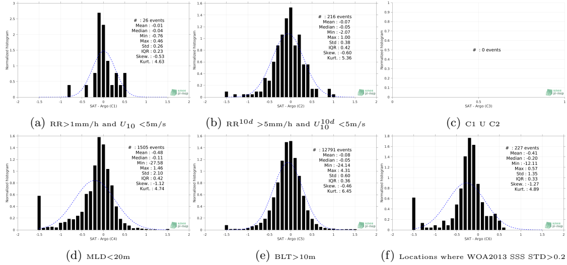
Figure 13: Normalized histogram of \Delta SSS (SMAP-L3-RSS-V3-MONTHLY-70KM - Argo) for 6 different subdatasets corresponding to: RR > 1mm/h and U_{10} < 5 m/s (a), RR 10d > 5mm/h and U_{10}^{10d} < 5 m/s (b), C1 U C2 (c), MLD < 20m (d), BLT > 10m (e), Locations where WOA2013 SSS STD > 0.2 (f).
