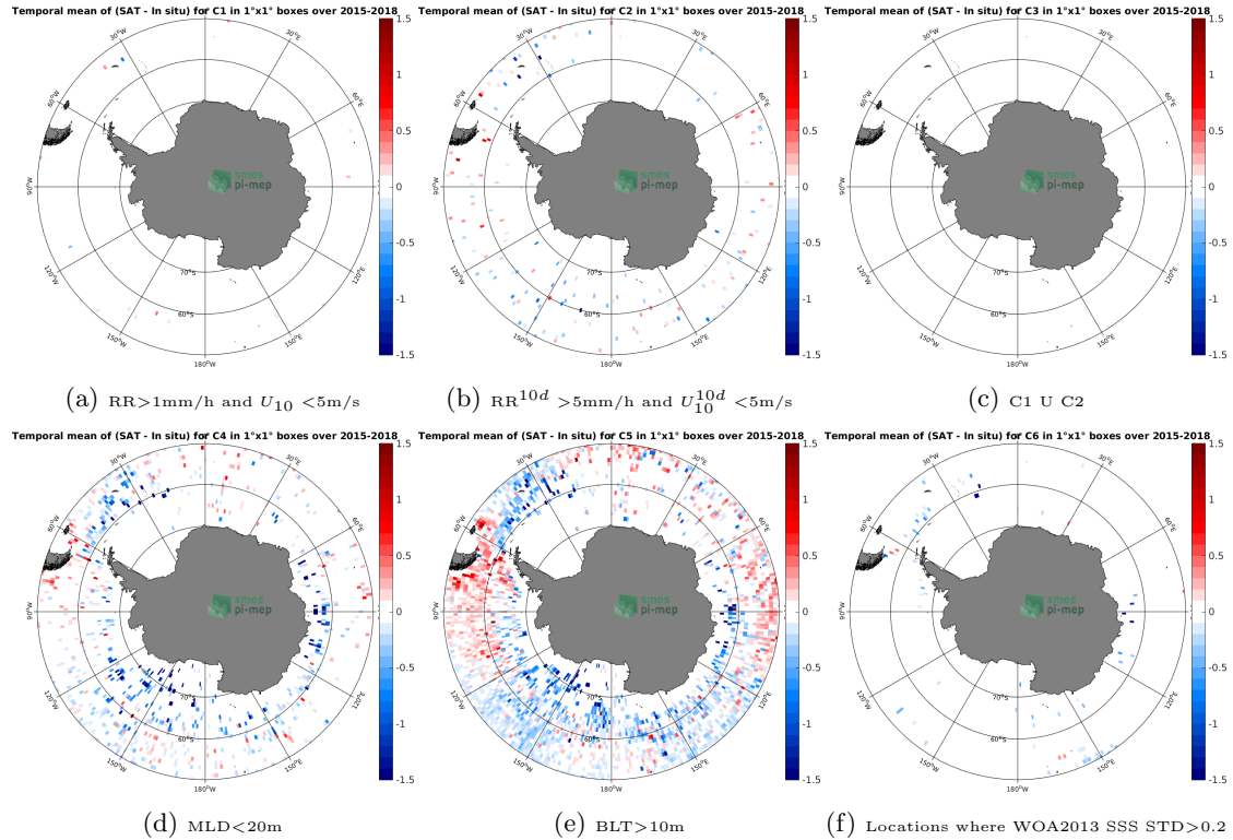
Figure 12: Temporal mean gridded over spatial boxes of size 1^\circ \times 1^\circ of \Delta\text{SSS} (SMAP-L3-RSS-V3-MONTHLY-70KM - Argo) for 6 different subdatasets corresponding to:RR > 1mm/h and U_{10} < 5\text{m/s} (a), \text{RR}^{10d} > 5\text{mm/h} and U_{10}^{10d} < 5\text{m/s} (b), C1 U C2 (c),MLD < 20m (d),BLT > 10m (e),Locations where WOA2013 SSS STD > 0.2 (f).
