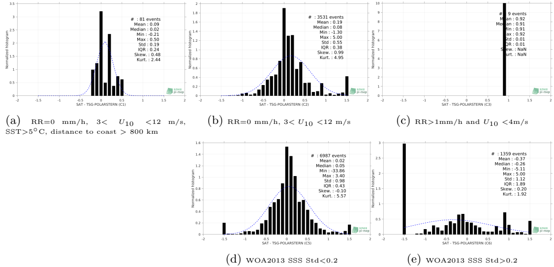
Figure 13: Normalized histogram of \Delta SSS (SMAP-L3-RSS-V3-MONTHLY-0.25DEG-40KM - TSG-POLARSTERN) for 5 different subdatasets corresponding to: RR=0 mm/h, 3 < U_{10} < 12 m/s, SST>5°C, distance to coast > 800 km (a), RR=0 mm/h, 3 < U_{10} < 12 m/s (b), RR>1mm/h and U_{10} < 4 m/s (c), WOA2013 SSS Std<0.2 (d), WOA2013 SSS Std>0.2 (e).
