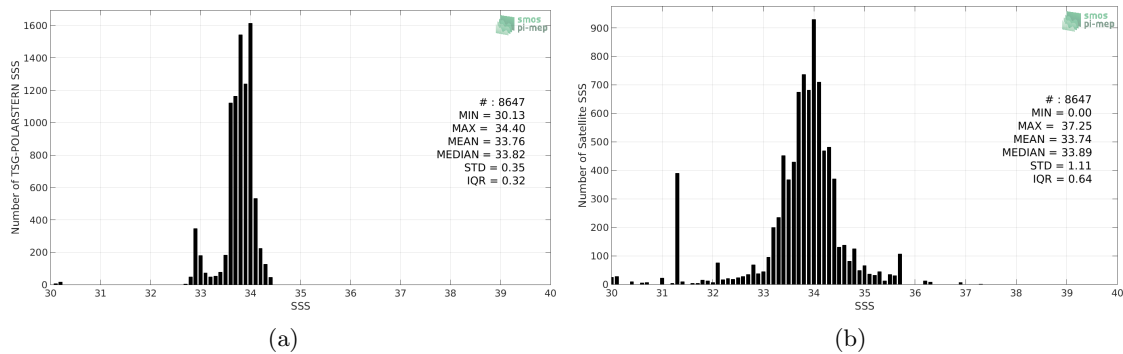
Figure 2: Histograms of SSS from TSG-POLARSTERN (a) and SMAP-L3-RSS-V3-MONTHLY-0.25DEG-40KM (b) considering all match-up pairs per bins of 0.1 over the Southern Ocean Pi-MEP region and for the full satellite product period.
