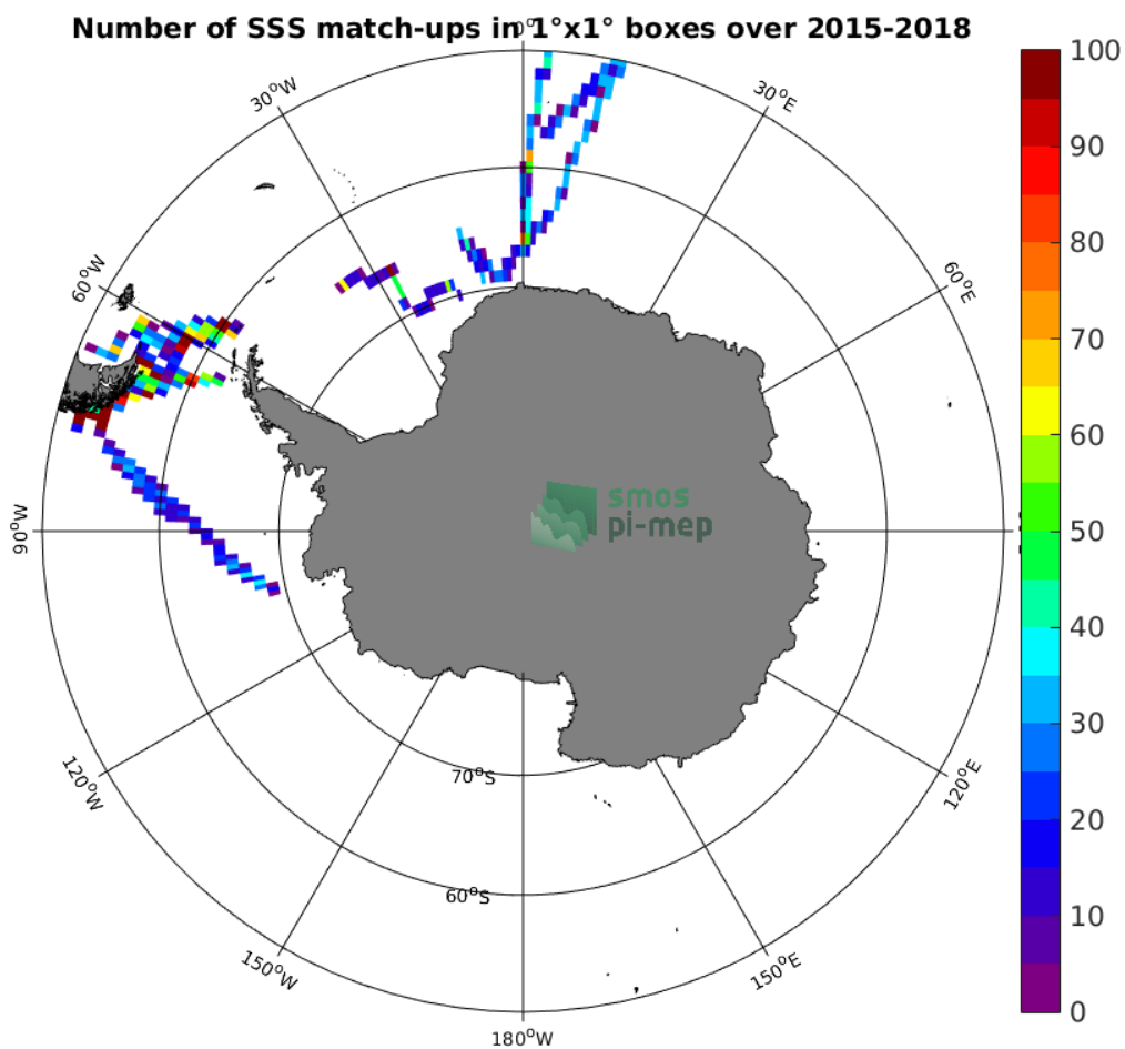
Figure 4: Number of SSS match-ups between TSG-POLARSTERN SSS and the SMAP-L3-RSS-V3-MONTHLY-0.25DEG-40KM SSS product for the Southern Ocean Pi-MEP region over 1^\circ \times 1^\circ boxes and for the full satellite product period.
