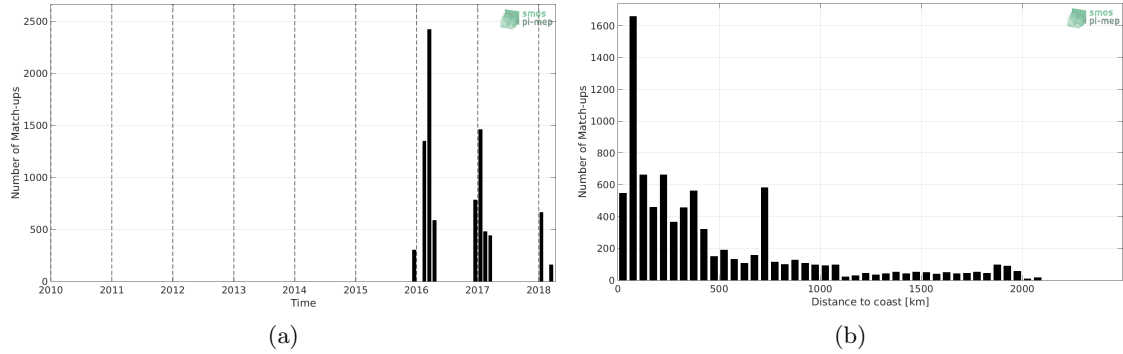
Figure 1: Number of match-ups between TSG-POLARSTERN and SMAP-L3-RSS-V3-MONTHLY-0.25DEG-40KM SSS as a function of time (a) and as function of the distance to coast (b) over the Southern Ocean Pi-MEP region and for the full satellite product period.
