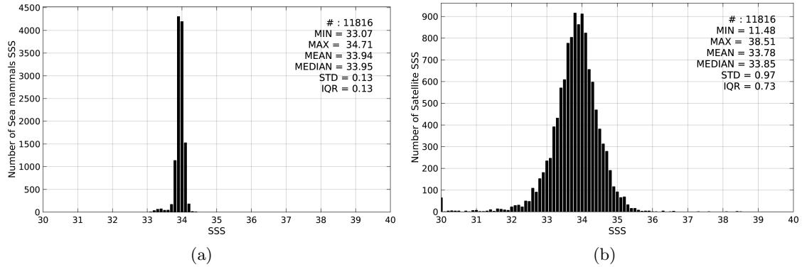
Figure 2: Histograms of SSS from Sea mammals (a) and SMAP-L3-RSS-V2-8DAY-RUNNING-70KM (b) considering all match-up pairs per bins of 0.1 over the Southern Ocean Pi-MEP region and for the full satellite product period.
