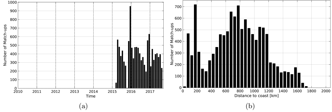
Figure 1: Number of match-ups between Sea mammals and SMAP-L3-RSS-V2-8DAY-RUNNING-70KM SSS as a function of time (a) and as function of the distance to coast (b) over the Southern Ocean Pi-MEP region and for the full satellite product period.
