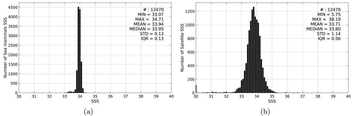
Figure 2: Histograms of SSS from Sea mammals (a) and SMAP-L3-RSS-V2-MONTHLY-0.25DEG-40KM (b) considering all match-up pairs per bins of 0.1 over the Southern Ocean Pi-MEP region and for the full satellite product period.
