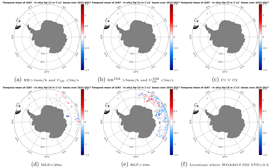
Figure 12: Temporally mean gridded over spatial boxes of size 1^\circ \times 1^\circ of \Delta SSS (SMAP-L3-RSS-V2-MONTHLY-0.25DEG-40KM - Sea mammals) for 6 different subdatasets corresponding to: RR > 1\text{mm/h} and U_{10} < 5\text{m/s} (a), RR^{10d} > 5\text{mm/h} and U_{10}^{10d} < 5\text{m/s} (b), C1 U C2 (c), MLD < 20\text{m} (d), BLT > 10\text{m} (e), Locations where WOA2013 SSS STD > 0.2 (f).
