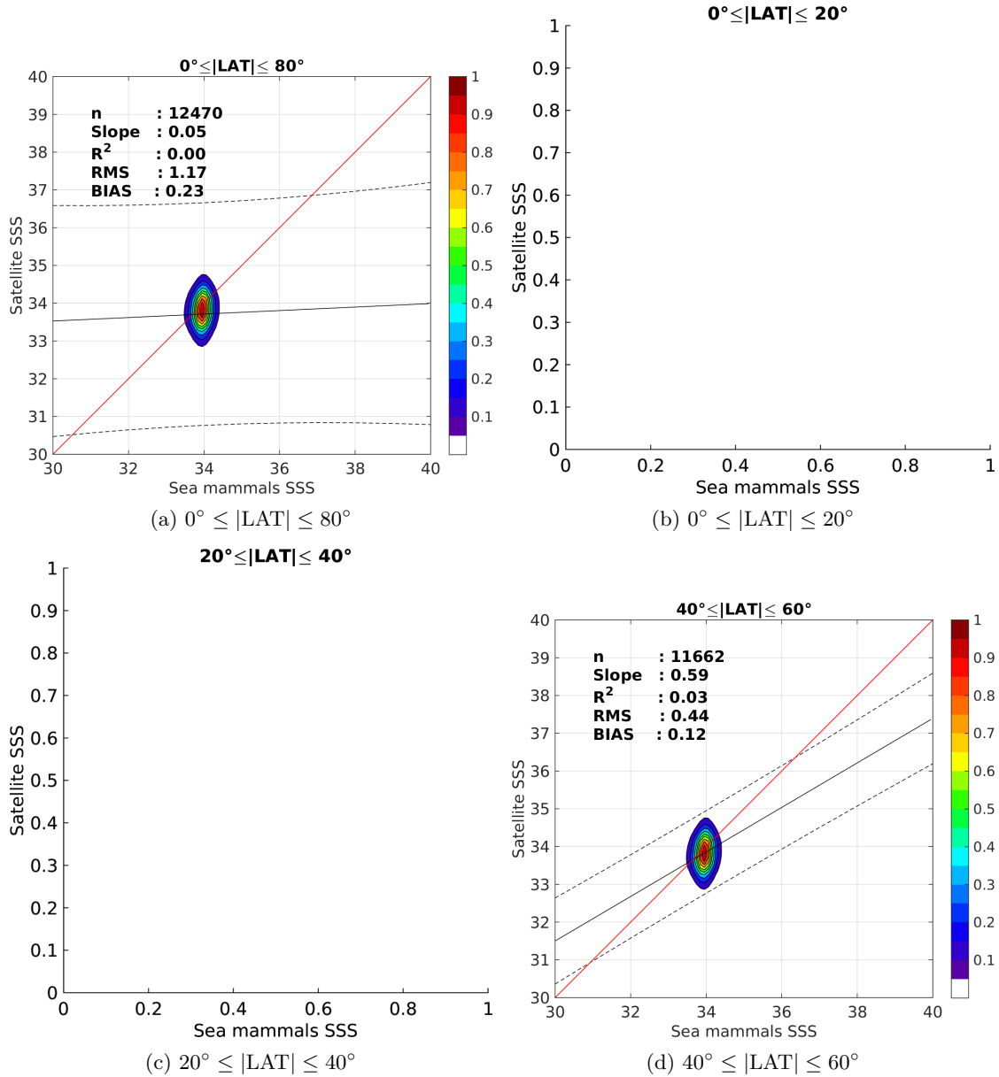
Figure 9: Contour maps of the concentration of SMAP-L3-RSS-V2-MONTHLY-0.25DEG-40KM SSS (y-axis) versus Sea mammals SSS (x-axis) at match-up pairs for different latitude bands. For each plot, the red line shows x=y . The black thin and dashed lines indicate a linear fit through the data cloud and the \pm 95\% confidence levels, respectively. The number match-up pairs n , the slope and R^2 coefficient of the linear fit, the root mean square (RMS) and the mean bias between satellite and in situ data are indicated for each latitude band in each plots.
