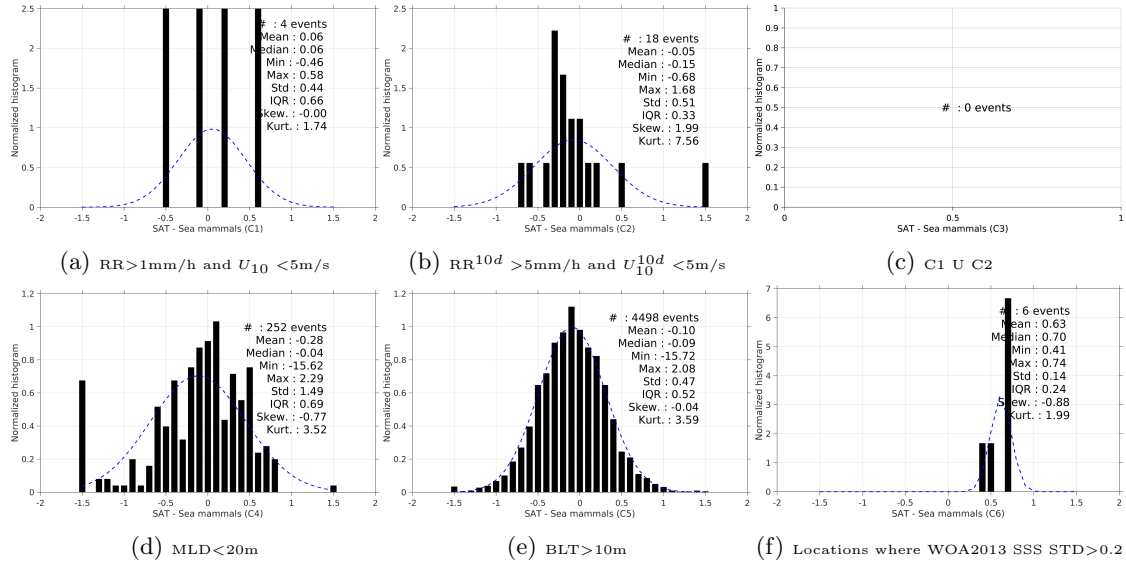
Figure 13: Normalized histogram of \Delta SSS (SMAP-L3-RSS-V2-MONTHLY-0.25DEG-40KM - Sea mammals) for 6 different subdatasets corresponding to: RR > 1\text{mm/h} and U_{10} < 5\text{m/s} (a), RR^{10d} > 5\text{mm/h} and U_{10}^{10d} < 5\text{m/s} (b), C1 \cup C2 (c), MLD < 20\text{m} (d), BLT > 10\text{m} (e), Locations where WOA2013 SSS STD > 0.2 (f).
