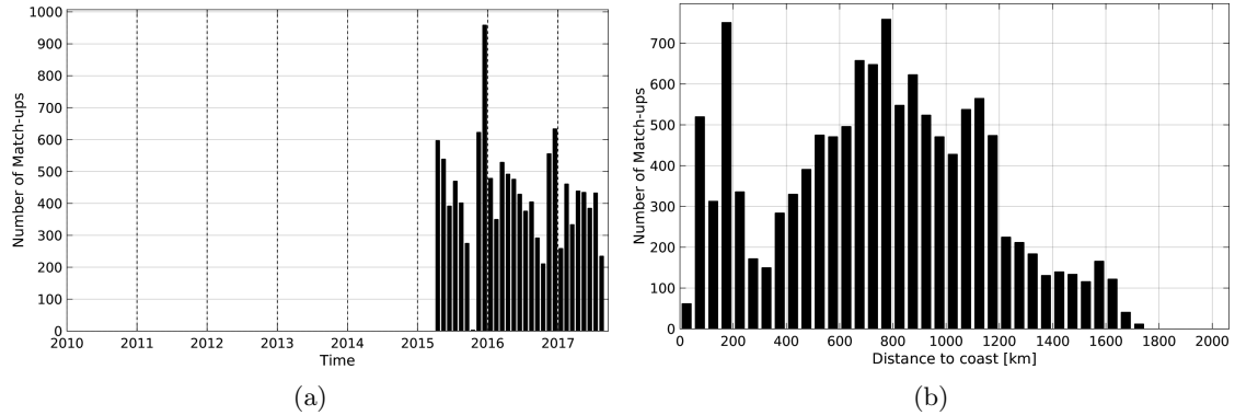
Figure 1: Number of match-ups between Sea mammals and SMAP-L3-RSS-V2-MONTHLY-0.25DEG-40KM SSS as a function of time (a) and as function of the distance to coast (b) over the Southern Ocean Pi-MEP region and for the full satellite product period.
