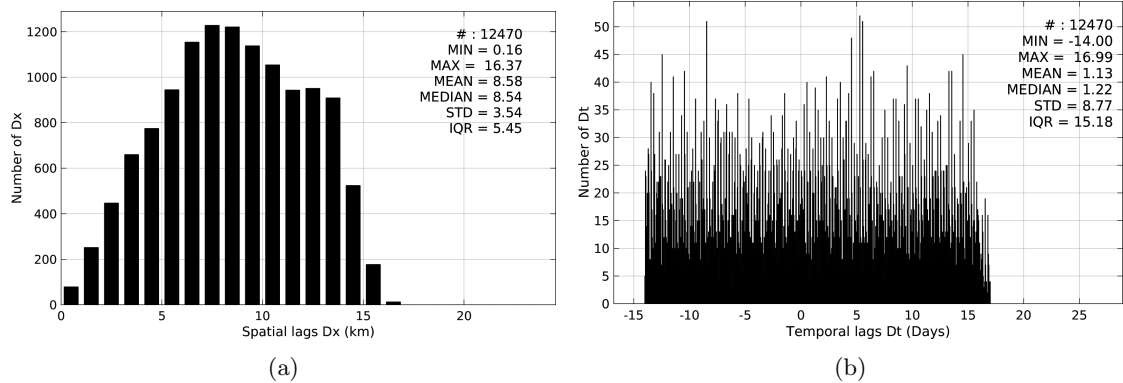
Figure 5: Histograms of the spatial (a) and temporal (b) lags between the time of the Sea mammals measurements and the date of the corresponding SMAP-L3-RSS-V2-MONTHLY-0.25DEG-40KM SSS product.
