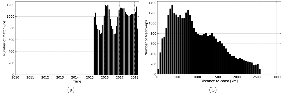
Figure 1: Number of match-ups between Argo and SMAP-L3-RSS-V2-MONTHLY-0.25DEG-40KM SSS as a function of time (a) and as function of the distance to coast (b) over the Southern Ocean Pi-MEP region and for the full satellite product period.
