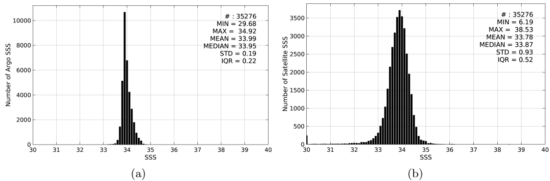
Figure 2: Histograms of SSS from Argo (a) and SMAP-L3-RSS-V2-MONTHLY-0.25DEG-40KM (b) considering all match-up pairs per bins of 0.1 over the Southern Ocean Pi-MEP region and for the full satellite product period.
