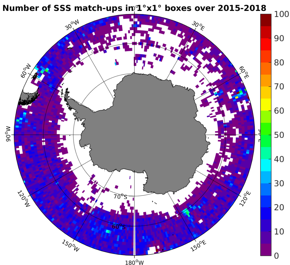
Figure 4: Number of SSS match-ups between Argo SSS and the SMAP-L3-RSS-V2-MONTHLY-0.25DEG-40KM SSS product for the Southern Ocean Pi-MEP region over 1^\circ \times 1^\circ boxes and for the full satellite product period.
