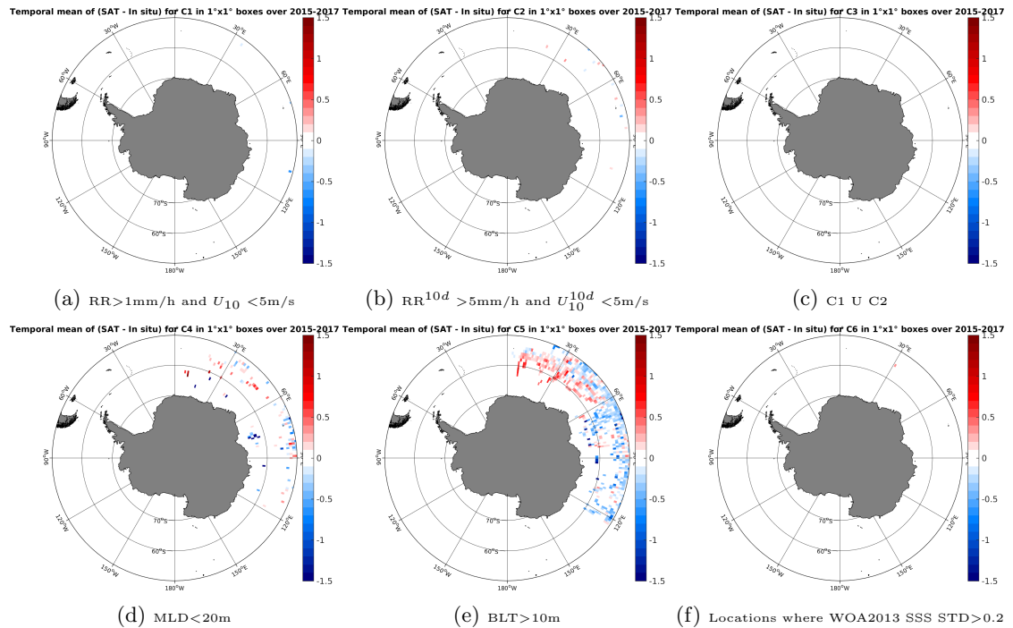
Figure 12: Temporal mean gridded over spatial boxes of size 1^\circ \times 1^\circ of \Delta SSS (SMAP-L3-RSS-V2-MONTHLY-70KM - Sea mammals) for 6 different subdatasets corresponding to: RR > 1\text{mm/h} and U_{10} < 5\text{m/s} (a), RR^{10d} > 5\text{mm/h} and U_{10}^{10d} < 5\text{m/s} (b), C1 U C2 (c), MLD < 20\text{m} (d), BLT > 10\text{m} (e), Locations where WOA2013 SSS STD > 0.2 (f).
