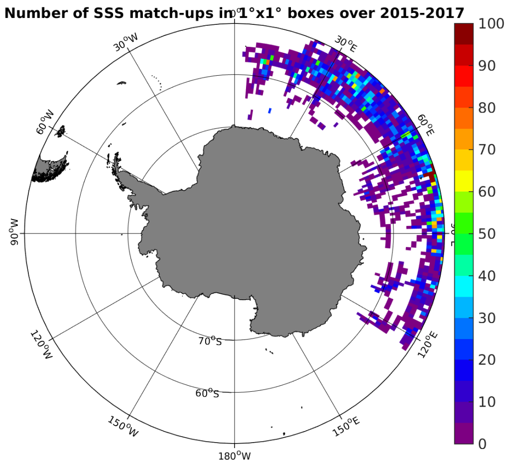
Figure 4: Number of SSS match-ups between Sea mammals SSS and the SMAP-L3-RSS-V2-MONTHLY-70KM SSS product for the Southern Ocean Pi-MEP region over 1^\circ \times 1^\circ boxes and for the full satellite product period.
