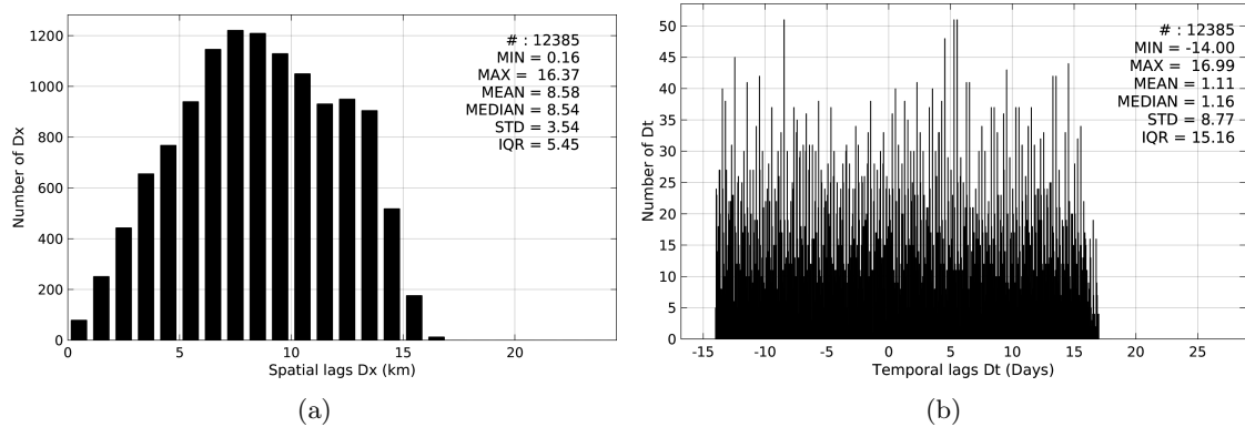
Figure 5: Histograms of the spatial (a) and temporal (b) lags between the time of the Sea mammals measurements and the date of the corresponding SMAP-L3-RSS-V2-MONTHLY-70KM SSS product.
