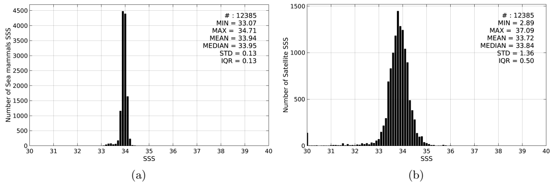
Figure 2: Histograms of SSS from Sea mammals (a) and SMAP-L3-RSS-V2-MONTHLY-70KM (b) considering all match-up pairs per bins of 0.1 over the Southern Ocean Pi-MEP region and for the full satellite product period.
