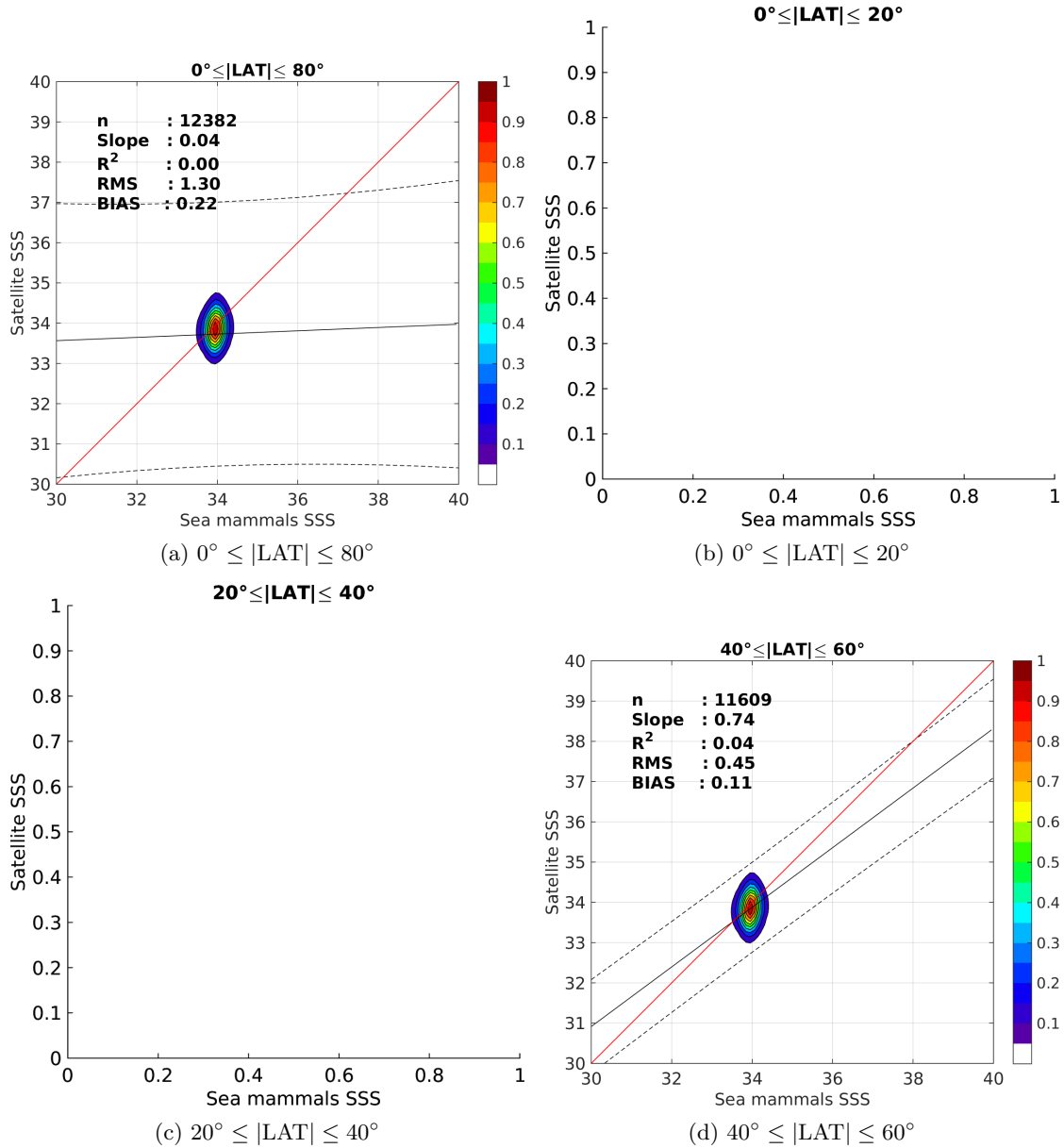
Figure 9: Contour maps of the concentration of SMAP-L3-RSS-V2-MONTHLY-70KM SSS (y-axis) versus Sea mammals SSS (x-axis) at match-up pairs for different latitude bands. For each plot, the red line shows x=y . The black thin and dashed lines indicate a linear fit through the data cloud and the \pm 95\% confidence levels, respectively. The number match-up pairs n , the slope and R^2 coefficient of the linear fit, the root mean square (RMS) and the mean bias between satellite and in situ data are indicated for each latitude band in each plots.
