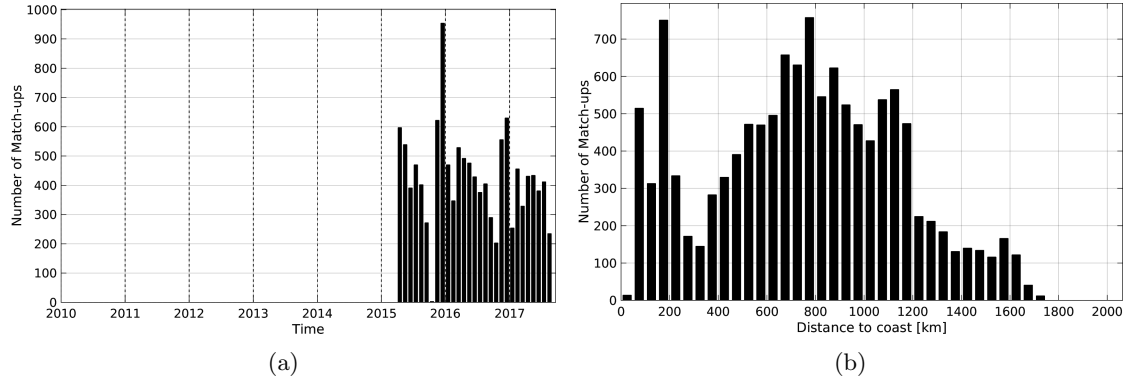
Figure 1: Number of match-ups between Sea mammals and SMAP-L3-RSS-V2-MONTHLY-70KM SSS as a function of time (a) and as function of the distance to coast (b) over the Southern Ocean Pi-MEP region and for the full satellite product period.
