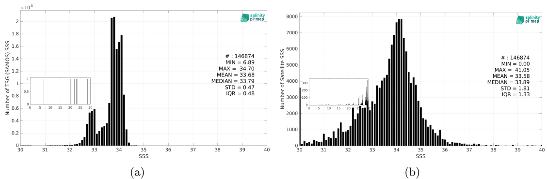
Figure 3: Histograms of SSS from TSG (SAMOS) (a) and SMAP SSS L3 v5.0 - 8-Day running (JPL) (b) considering all match-up pairs per bins of 0.1 over the Southern Ocean Pi-MEP region and for the full satellite product period.
