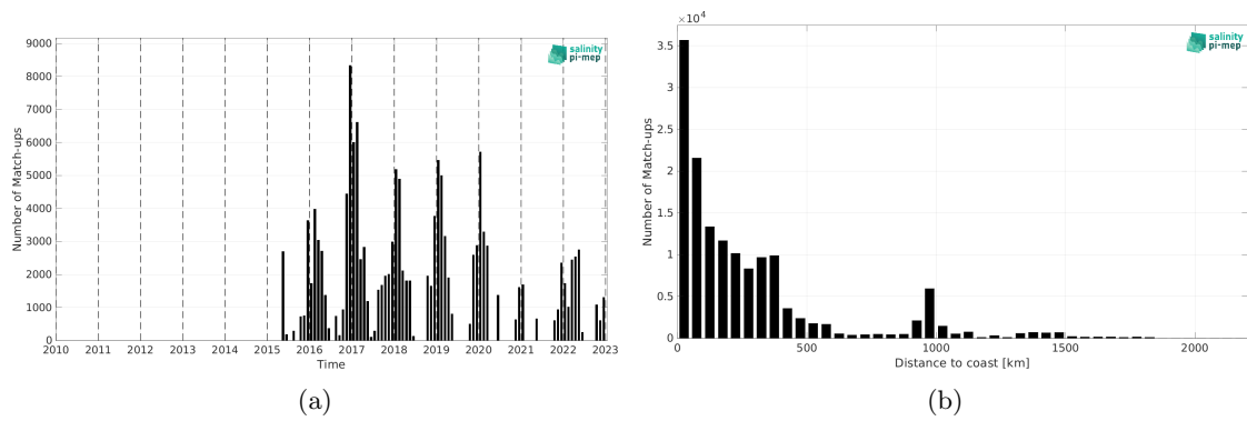
Figure 2: Number of match-ups between TSG (SAMOS) and SMAP SSS L3 v5.0 - 8-Day running (JPL) SSS as a function of time (a) and as function of the distance to coast (b) over the Southern Ocean Pi-MEP region and for the full satellite product period.
