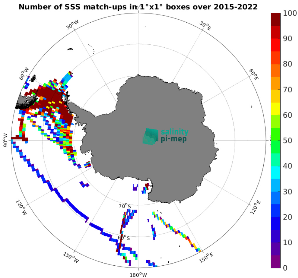
Figure 5: Number of SSS match-ups between TSG (SAMOS) SSS and the SMAP SSS L3 v5.0 - 8-Day running (JPL) SSS product for the Southern Ocean Pi-MEP region over 1^\circ \times 1^\circ boxes and for the full satellite product period.
