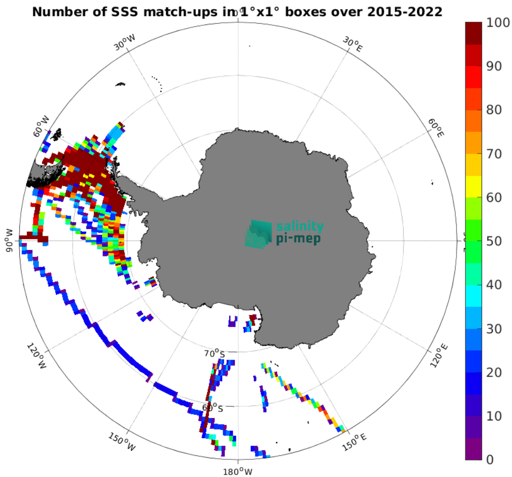
Figure 4: Number of SSS match-ups between TSG (SAMOS) SSS and the SMAP SSS L3 v5.0 - 8-Day running (JPL) SSS product for the Southern Ocean Pi-MEP region over 1^{\circ} \times 1^{\circ} boxes and for the full satellite product period.
