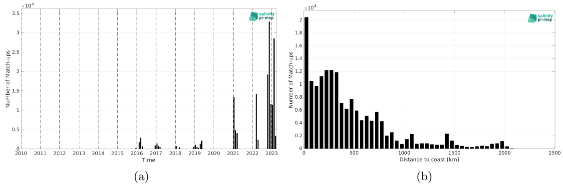
Figure 2: Number of match-ups between TSG (Polarstern) and SMAP SSS L3 v5.0 - 8-Day running (JPL) SSS as a function of time (a) and as function of the distance to coast (b) over the Southern Ocean Pi-MEP region and for the full satellite product period.
