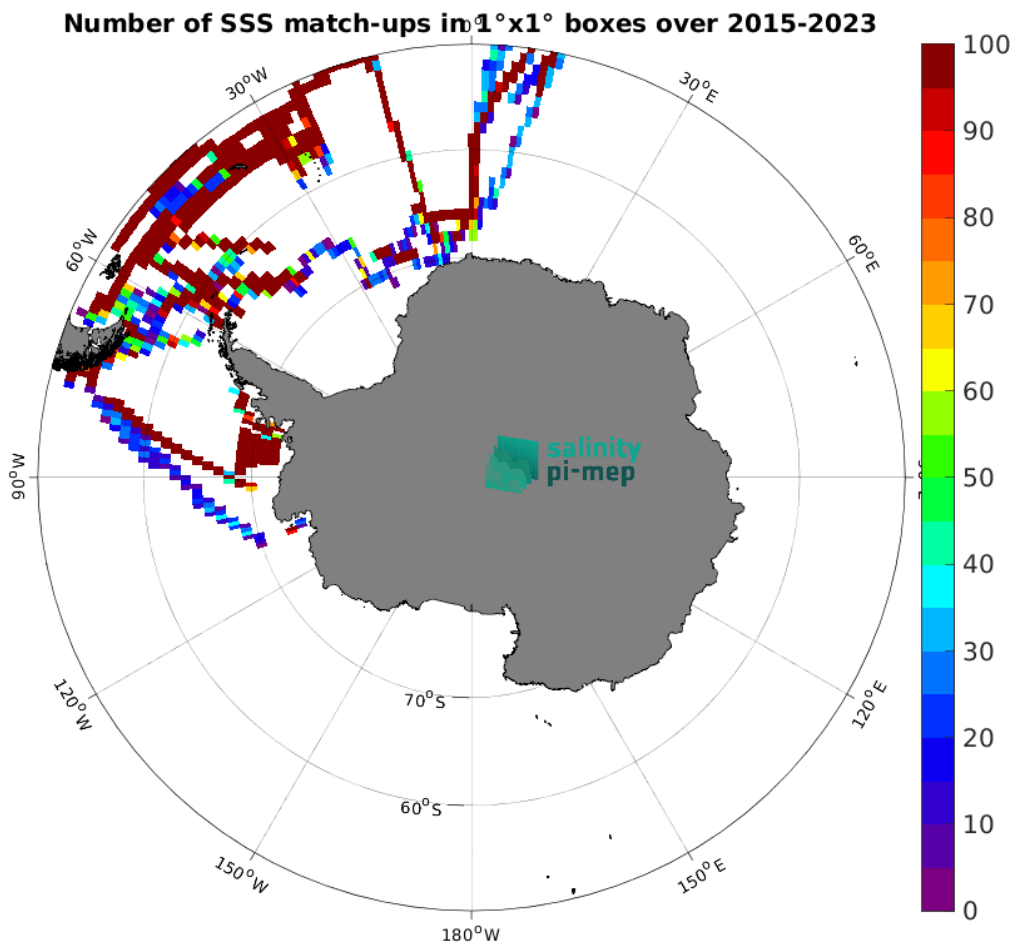
Figure 5: Number of SSS match-ups between TSG (Polarstern) SSS and the SMAP SSS L3 v5.0 - 8-Day running (JPL) SSS product for the Southern Ocean Pi-MEP region over 1^{\circ} \times 1^{\circ} boxes and for the full satellite product period.
