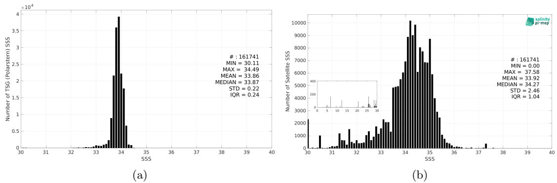
Figure 3: Histograms of SSS from TSG (Polarstern) (a) and SMAP SSS L3 v5.0 - 8-Day running (JPL) (b) considering all match-up pairs per bins of 0.1 over the Southern Ocean Pi-MEP region and for the full satellite product period.
