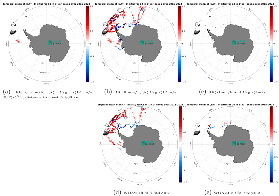
Figure 14: Temporal mean gridded over spatial boxes of size 1^\circ \times 1^\circ of \Delta\text{SSS} (SMAP SSS L3 v5.0 - 8-Day running (JPL) - TSG (Polarstern)) for 5 different subdatasets corresponding to:RR=0 mm/h, 3 < U_{10} < 12 m/s, SST>5°C, distance to coast > 800 km (a), RR=0 mm/h, 3 < U_{10} < 12 m/s (b), RR>1mm/h and U_{10} < 4 m/s (c), WOA2013 SSS Std<0.2 (d), WOA2013 SSS Std>0.2 (e).
