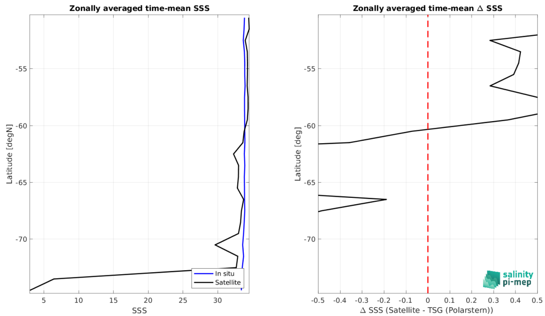
Figure 9: Left panel: Zonal mean SSS from SMAP SSS L3 v5.0 - 8-Day running (JPL) satellite product (black) and from TSG (Polarstern) (blue). Right panel: Zonal mean of \Delta SSS (Satellite - TSG (Polarstern)) for all the collected Pi-MEP match-up pairs estimated over the full satellite product period.
