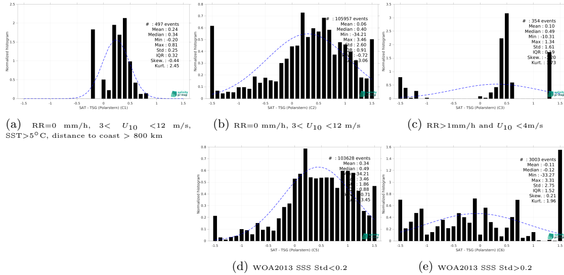
Figure 15: Normalized histogram of \Delta SSS (SMAP SSS L3 v5.0 - 8-Day running (JPL) - TSG (Polarstern)) for 5 different subdatasets corresponding to: RR=0 mm/h, 3 < U_{10} < 12 m/s, SST>5°C, distance to coast > 800 km (a), RR=0 mm/h, 3 < U_{10} < 12 m/s (b), RR>1mm/h and U_{10} < 4 m/s (c), WOA2013 SSS Std<0.2 (d), WOA2013 SSS Std>0.2 (e).
