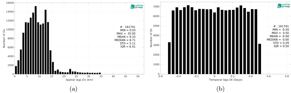
Figure 6: Histograms of the spatial (a) and temporal (b) lags between the location/time of the TSG (Polarstern) measurement and the date of the corresponding SMAP SSS L3 v5.0 - 8-Day running (JPL) SSS pixel.
