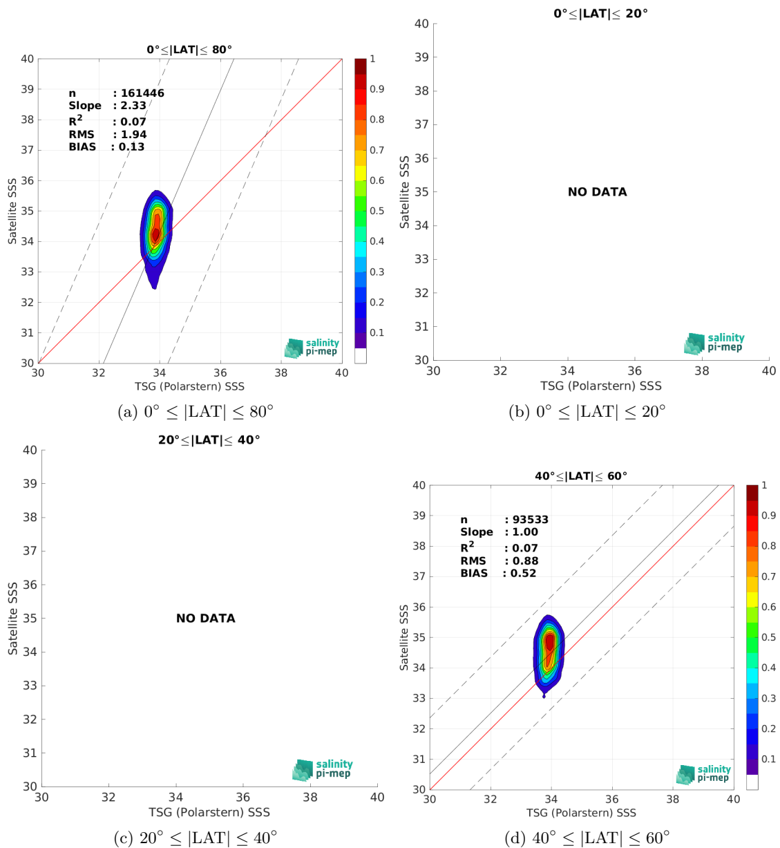
Figure 10: Contour maps of the concentration of SMAP SSS L3 v5.0 - 8-Day running (JPL) SSS (y-axis) versus TSG (Polarstern) SSS (x-axis) at match-up pairs for different latitude bands. For each plot, the red line shows x=y . The black thin and dashed lines indicate a linear fit through the data cloud and the \pm 95\% confidence levels, respectively. The number match-up pairs n , the slope and R^2 coefficient of the linear fit, the root mean square (RMS) and the mean bias between satellite and in situ data are indicated for each latitude band in each plots.
