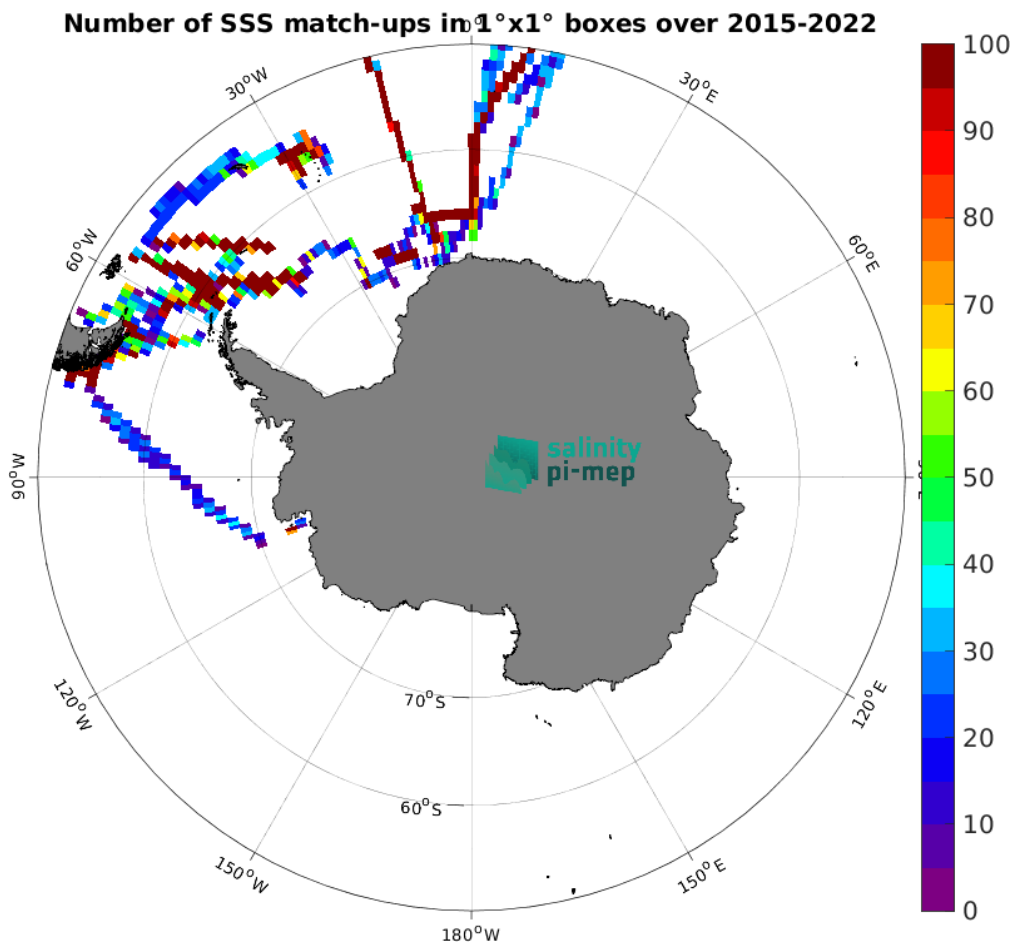
Figure 4: Number of SSS match-ups between TSG (Polarstern) SSS and the SMAP SSS L3 v5.0 - 8-Day running (JPL) SSS product for the Southern Ocean Pi-MEP region over 1^{\circ} \times 1^{\circ} boxes and for the full satellite product period.
