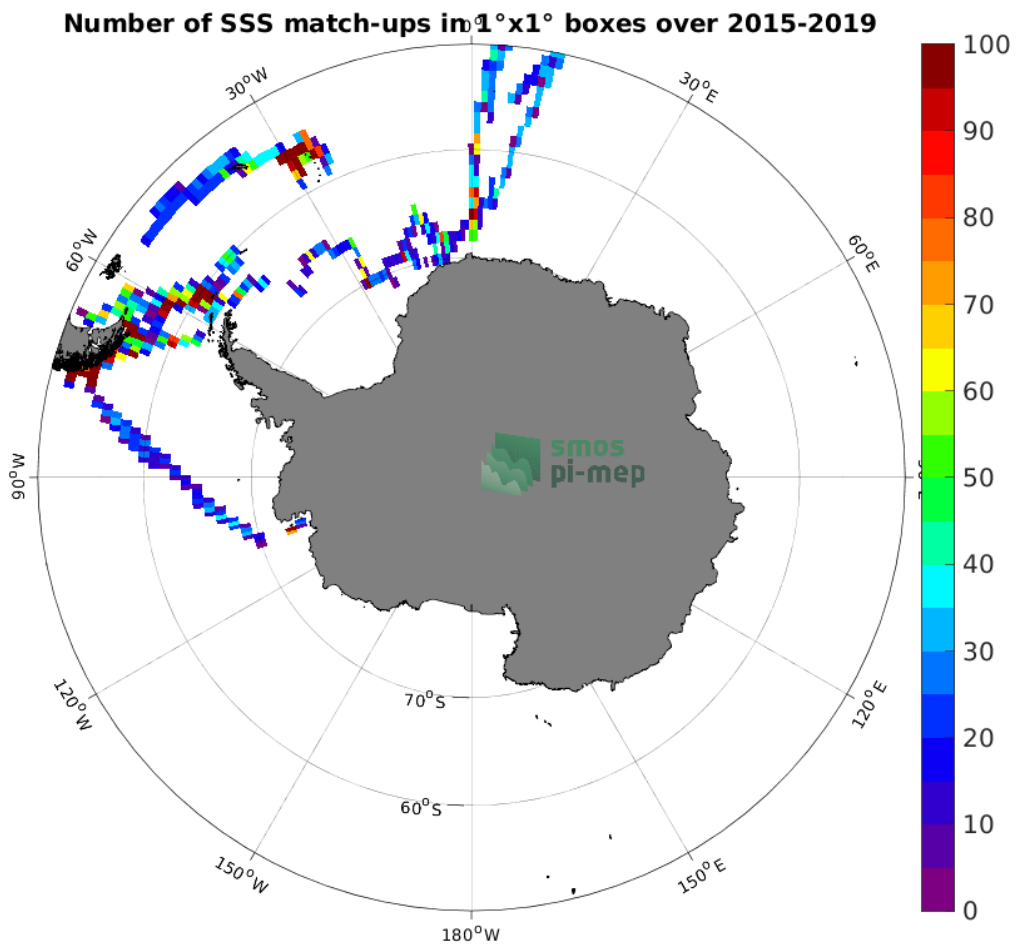
Figure 4: Number of SSS match-ups between TSG (Polarstern) SSS and the SMAP SSS L3 v5.0 - 8-Day running (JPL) SSS product for the Southern Ocean Pi-MEP region over 1^\circ \times 1^\circ boxes and for the full satellite product period.
