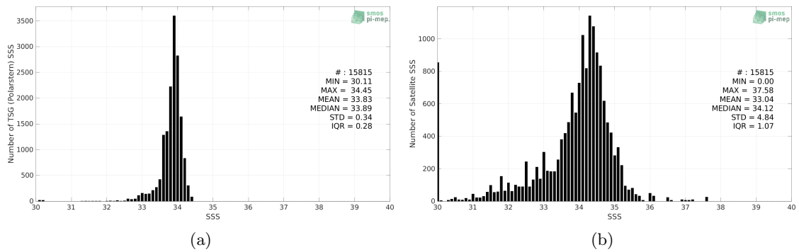
Figure 2: Histograms of SSS from TSG (Polarstern) (a) and SMAP SSS L3 v5.0 - 8-Day running (JPL) (b) considering all match-up pairs per bins of 0.1 over the Southern Ocean Pi-MEP region and for the full satellite product period.
