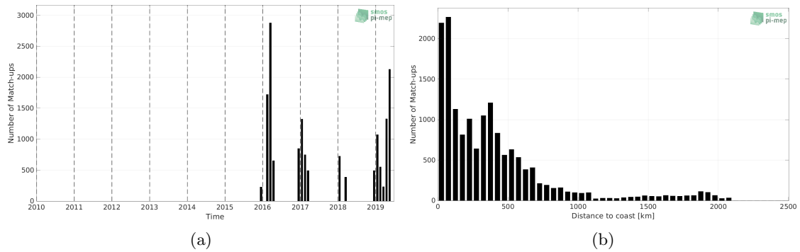
Figure 1: Number of match-ups between TSG (Polarstern) and SMAP SSS L3 v5.0 - 8-Day running (JPL) SSS as a function of time (a) and as function of the distance to coast (b) over the Southern Ocean Pi-MEP region and for the full satellite product period.
