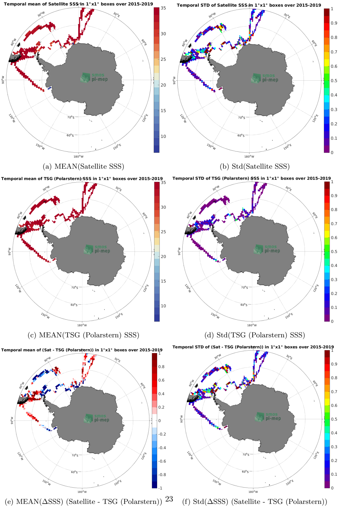
Figure 6: Temporal mean (left) and Std (right) of SSS from SMAP SSS L3 v5.0 - 8-Day running (JPL) (top), TSG (Polarstern) (middle), and of \Delta SSS (Satellite - TSG (Polarstern)). Only match-up pairs are used to generate these maps.
