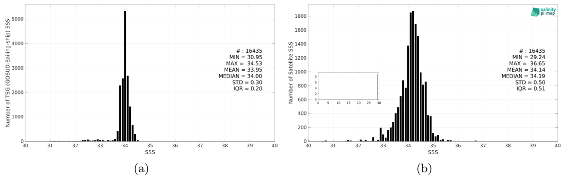
Figure 3: Histograms of SSS from TSG (GOSUD-Sailing-ship) (a) and SMAP SSS L3 v5.0 - 8-Day running (JPL) (b) considering all match-up pairs per bins of 0.1 over the Southern Ocean Pi-MEP region and for the full satellite product period.
