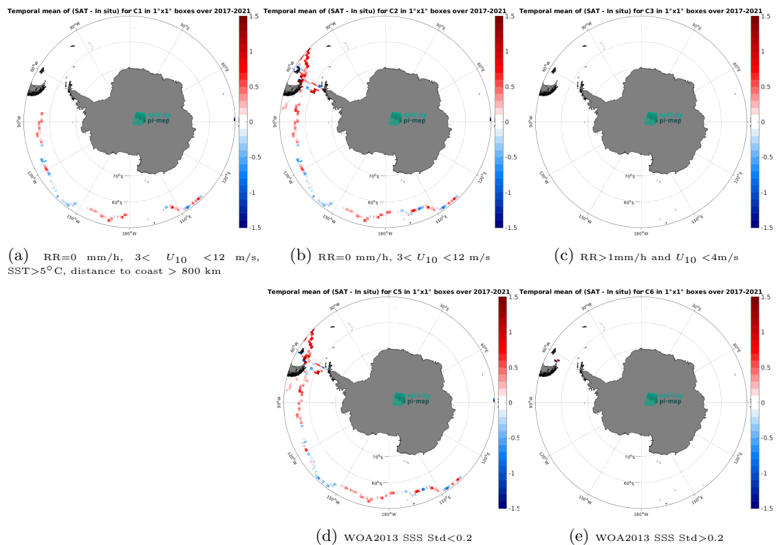
Figure 14: Temporal mean gridded over spatial boxes of size 1^\circ \times 1^\circ of \Delta SSS (SMAP SSS L3 v5.0 - 8-Day running (JPL) - TSG (GOSUD-Sailing-ship)) for 5 different subdatasets corresponding to:RR=0 mm/h, 3 < U_{10} < 12 m/s, SST>5°C, distance to coast > 800 km (a), RR=0 mm/h, 3 < U_{10} < 12 m/s (b), RR>1mm/h and U_{10} < 4 m/s (c), WOA2013 SSS Std<0.2 (d), WOA2013 SSS Std>0.2 (e).
