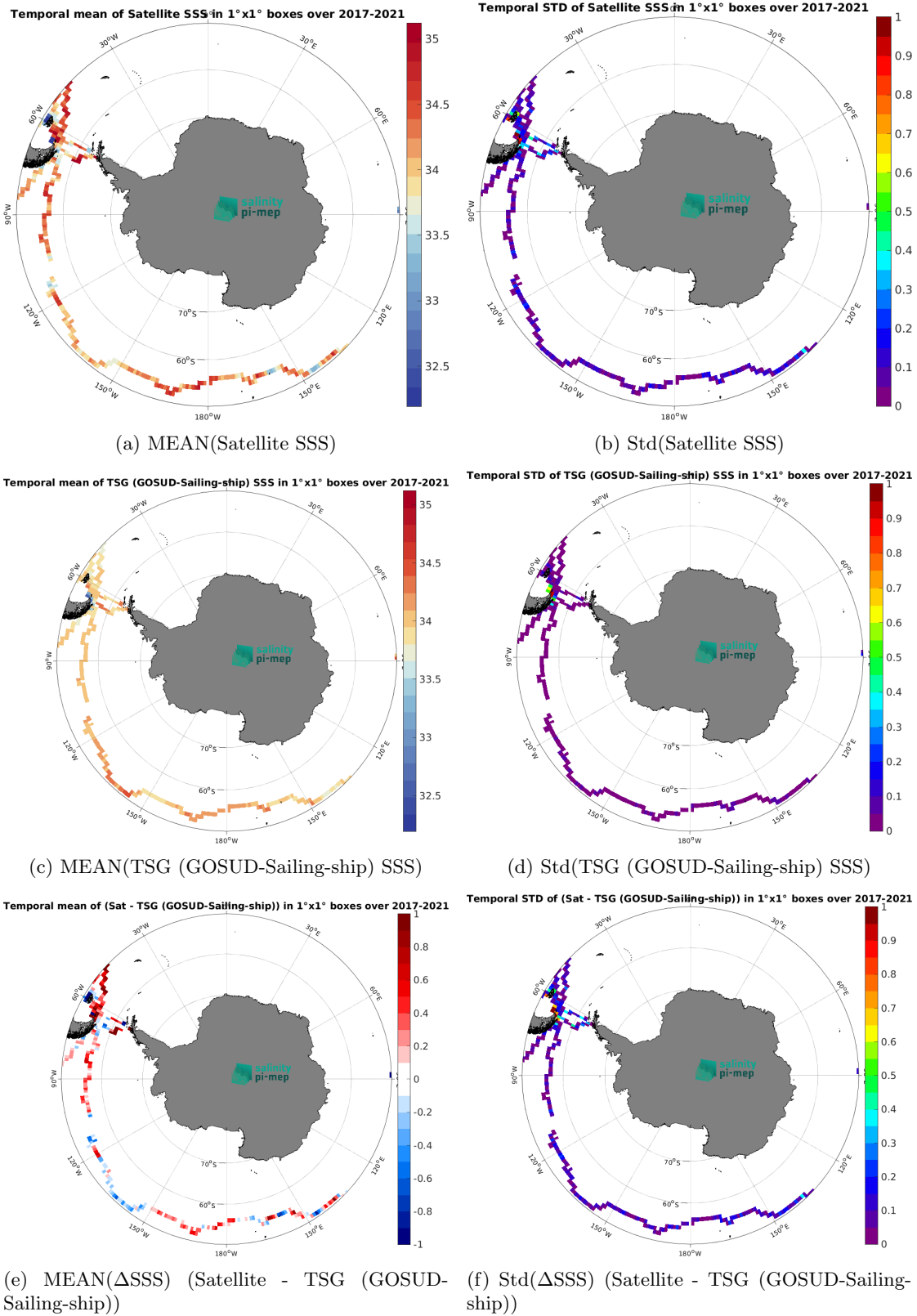
Figure 7: Temporal mean (left) and Std (right), of SSS from SMAP SSS L3 v5.0 - 8-Day running (JPL) (top), TSG (GOSUD-Sailing-ship) (middle), and of \Delta SSS (Satellite - TSG (GOSUD-Sailing-ship)). Only match-up pairs are used to generate these maps.
