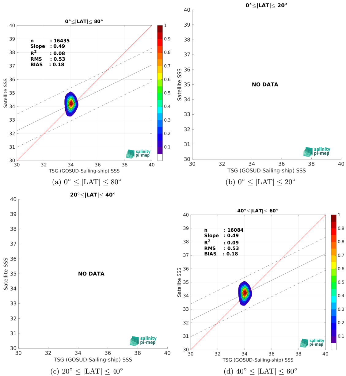
Figure 10: Contour maps of the concentration of SMAP SSS L3 v5.0 - 8-Day running (JPL) SSS (y-axis) versus TSG (GOSUD-Sailing-ship) SSS (x-axis) at match-up pairs for different latitude bands. For each plot, the red line shows x=y . The black thin and dashed lines indicate a linear fit through the data cloud and the \pm 95\% confidence levels, respectively. The number match-up pairs n , the slope and R^2 coefficient of the linear fit, the root mean square (RMS) and the mean bias between satellite and in situ data are indicated for each latitude band in each plots.
