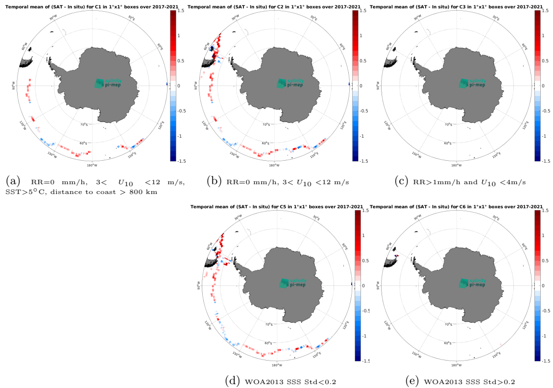
Figure 12: Temporal mean gridded over spatial boxes of size 1^\circ \times 1^\circ of \Delta\text{SSS} (SMAP SSS L3 v5.0 - 8-Day running (JPL) - TSG (GOSUD-Sailing-ship)) for 5 different subdatasets corresponding to: RR=0 mm/h, 3 < U_{10} < 12 m/s, SST > 5^\circ\text{C} , distance to coast > 800 km (a), RR=0 mm/h, 3 < U_{10} < 12 m/s (b), RR > 1 mm/h and U_{10} < 4 m/s (c), WOA2013 SSS Std <0.2 (d), WOA2013 SSS Std >0.2 (e).
