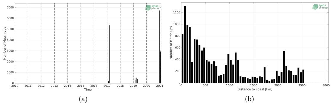
Figure 1: Number of match-ups between TSG (GOSUD-Sailing-ship) and SMAP SSS L3 v5.0 - 8-Day running (JPL) SSS as a function of time (a) and as function of the distance to coast (b) over the Southern Ocean Pi-MEP region and for the full satellite product period.
