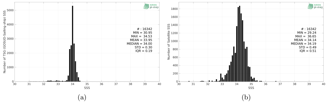
Figure 2: Histograms of SSS from TSG (GOSUD-Sailing-ship) (a) and SMAP SSS L3 v5.0 - 8-Day running (JPL) (b) considering all match-up pairs per bins of 0.1 over the Southern Ocean Pi-MEP region and for the full satellite product period.
