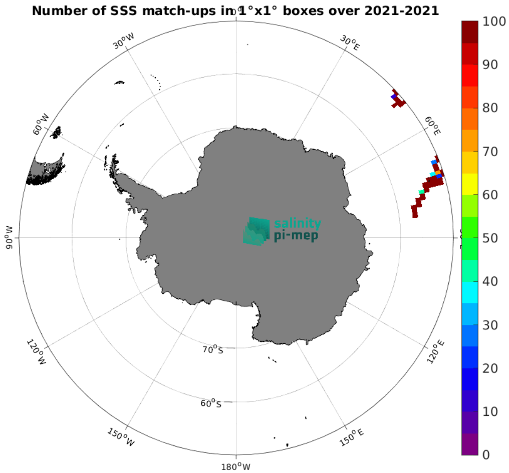
Figure 5: Number of SSS match-ups between TSG (GOSUD-Research-vessel) SSS and the SMAP SSS L3 v5.0 - 8-Day running (JPL) SSS product for the Southern Ocean Pi-MEP region over 1^\circ \times 1^\circ boxes and for the full satellite product period.
