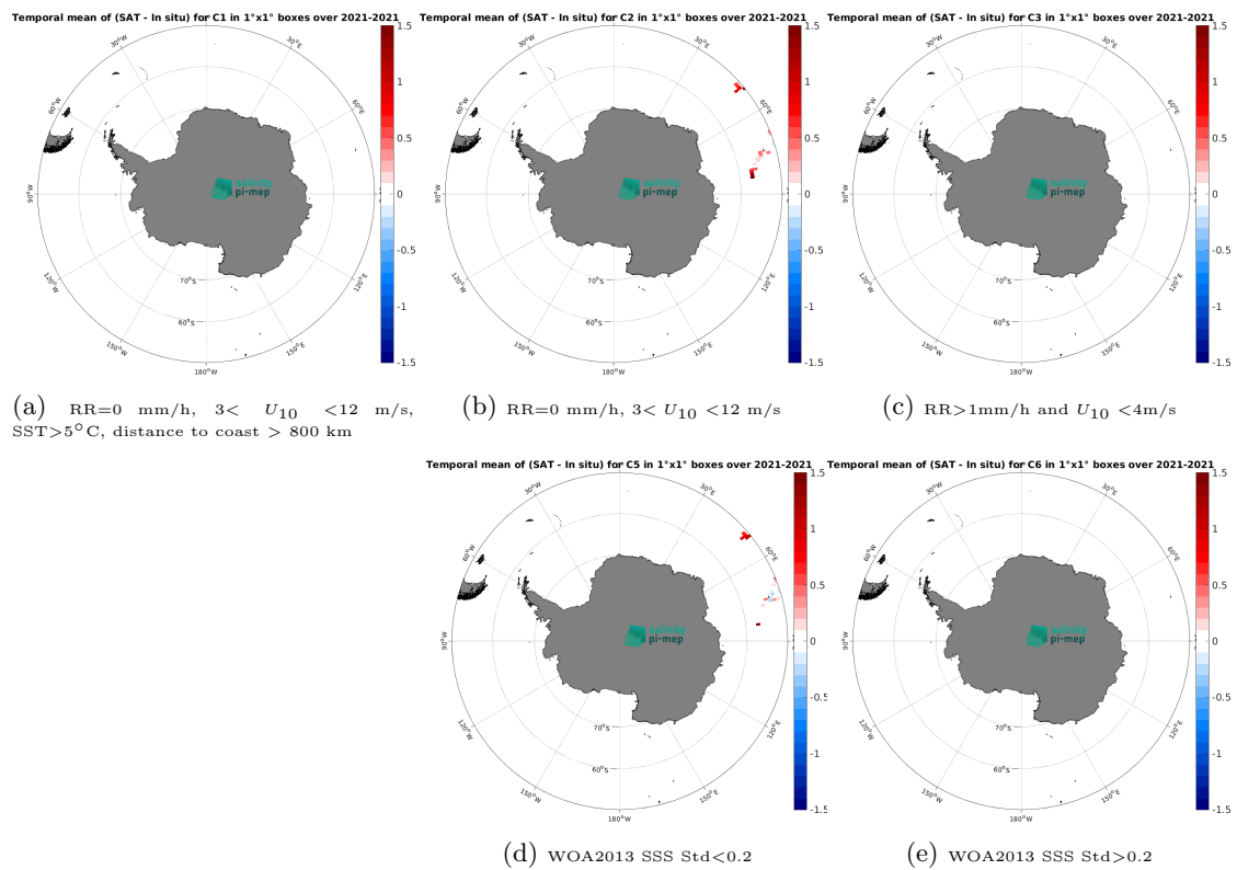
Figure 14: Temporal mean gridded over spatial boxes of size 1^\circ \times 1^\circ of \Delta\text{SSS} (SMAP SSS L3 v5.0 - 8-Day running (JPL) - TSG (GOSUD-Research-vessel)) for 5 different subdatasets corresponding to:RR=0 mm/h, 3 < U_{10} < 12 m/s, SST>5°C, distance to coast > 800 km (a), RR=0 mm/h, 3 < U_{10} < 12 m/s (b), RR>1mm/h and U_{10} < 4 m/s (c), WOA2013 SSS Std<0.2 (d), WOA2013 SSS Std>0.2 (e).
