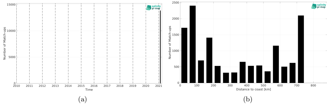
Figure 2: Number of match-ups between TSG (GOSUD-Research-vessel) and SMAP SSS L3 v5.0 - 8-Day running (JPL) SSS as a function of time (a) and as function of the distance to coast (b) over the Southern Ocean Pi-MEP region and for the full satellite product period.
