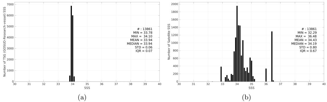
Figure 3: Histograms of SSS from TSG (GOSUD-Research-vessel) (a) and SMAP SSS L3 v5.0 - 8-Day running (JPL) (b) considering all match-up pairs per bins of 0.1 over the Southern Ocean Pi-MEP region and for the full satellite product period.
