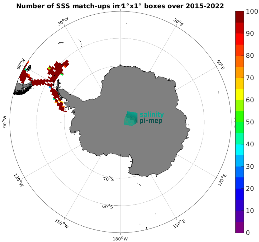
Figure 5: Number of SSS match-ups between TSG (CSIC-UTM) SSS and the SMAP SSS L3 v5.0 - 8-Day running (JPL) SSS product for the Southern Ocean Pi-MEP region over 1^\circ \times 1^\circ boxes and for the full satellite product period.
