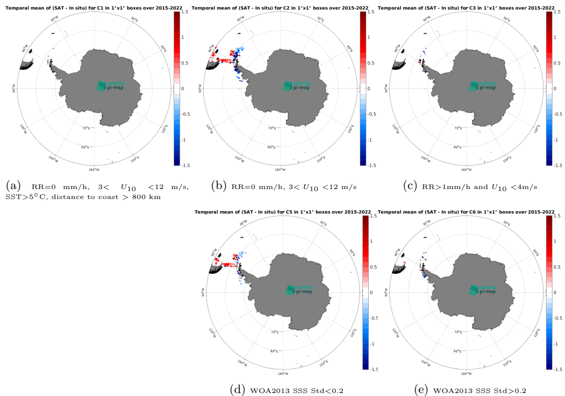
Figure 14: Temporal mean gridded over spatial boxes of size 1^\circ \times 1^\circ of \Delta\text{SSS} (SMAP SSS L3 v5.0 - 8-Day running (JPL) - TSG (CSIC-UTM)) for 5 different subdatasets corresponding to:RR=0 mm/h, 3 < U_{10} < 12 m/s, SST>5°C, distance to coast > 800 km (a), RR=0 mm/h, 3 < U_{10} < 12 m/s (b), RR>1mm/h and U_{10} < 4 m/s (c), WOA2013 SSS Std<0.2 (d), WOA2013 SSS Std>0.2 (e).
