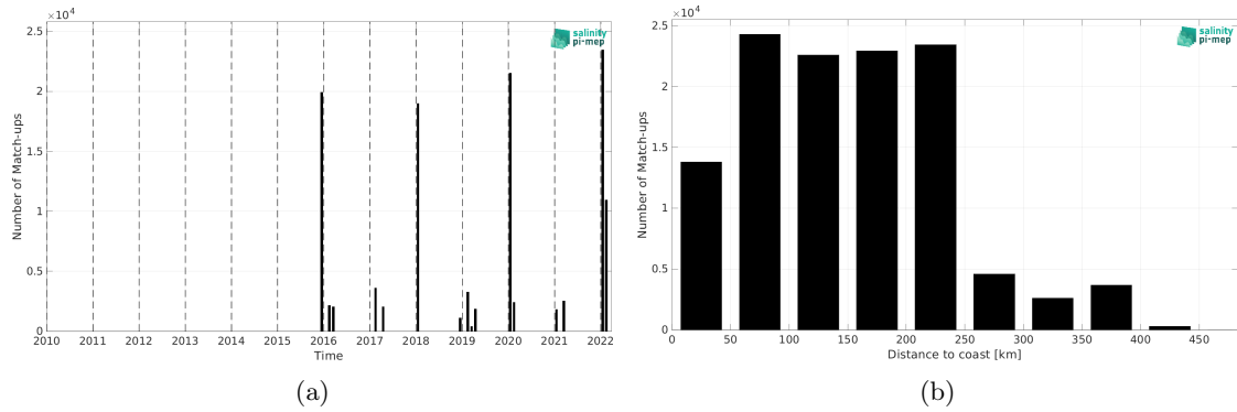
Figure 1: Number of match-ups between TSG (CSIC-UTM) and SMAP SSS L3 v5.0 - 8-Day running (JPL) SSS as a function of time (a) and as function of the distance to coast (b) over the Southern Ocean Pi-MEP region and for the full satellite product period.
