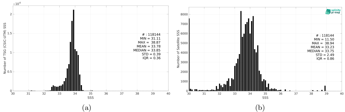
Figure 2: Histograms of SSS from TSG (CSIC-UTM) (a) and SMAP SSS L3 v5.0 - 8-Day running (JPL) (b) considering all match-up pairs per bins of 0.1 over the Southern Ocean Pi-MEP region and for the full satellite product period.
