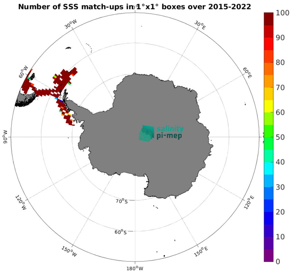
Figure 4: Number of SSS match-ups between TSG (CSIC-UTM) SSS and the SMAP SSS L3 v5.0 - 8-Day running (JPL) SSS product for the Southern Ocean Pi-MEP region over 1^\circ \times 1^\circ boxes and for the full satellite product period.
