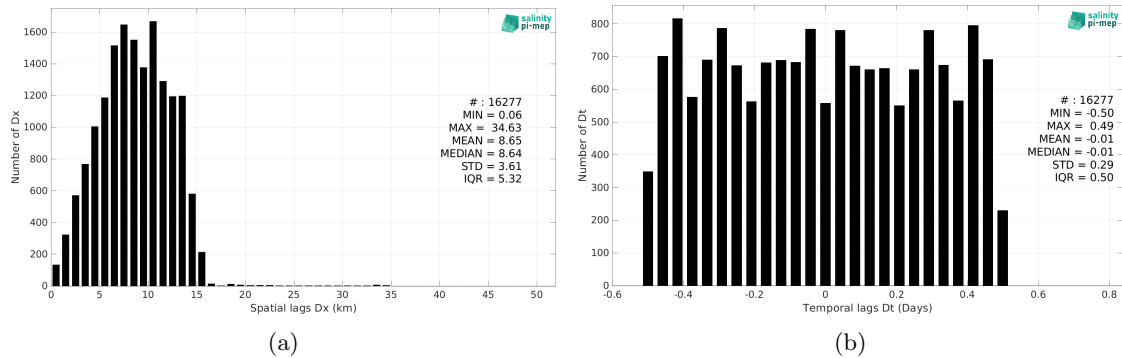
Figure 6: Histograms of the spatial (a) and temporal (b) lags between the location/time of the Saildrone measurement and the date of the corresponding SMAP SSS L3 v5.0 - 8-Day running (JPL) SSS pixel.
