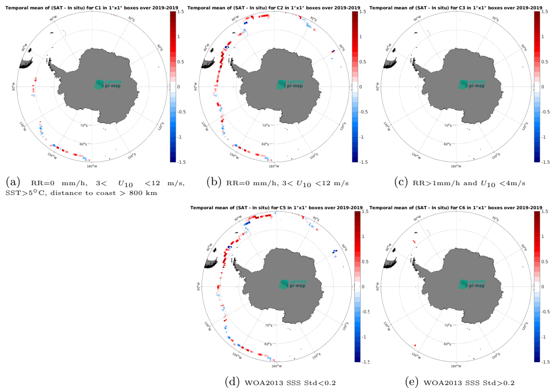
Figure 14: Temporal mean gridded over spatial boxes of size 1^\circ \times 1^\circ of \Delta SSS (SMAP SSS L3 v5.0 - 8-Day running (JPL) - Saikrone) for 5 different subdatasets corresponding to:RR=0 mm/h, 3 < U_{10} < 12 m/s, SST > 5^\circ\text{C} , distance to coast > 800 km (a), RR=0 mm/h, 3 < U_{10} < 12 m/s (b), RR > 1 mm/h and U_{10} < 4 m/s (c), WOA2013 SSS Std < 0.2 (d), WOA2013 SSS Std > 0.2 (e).
