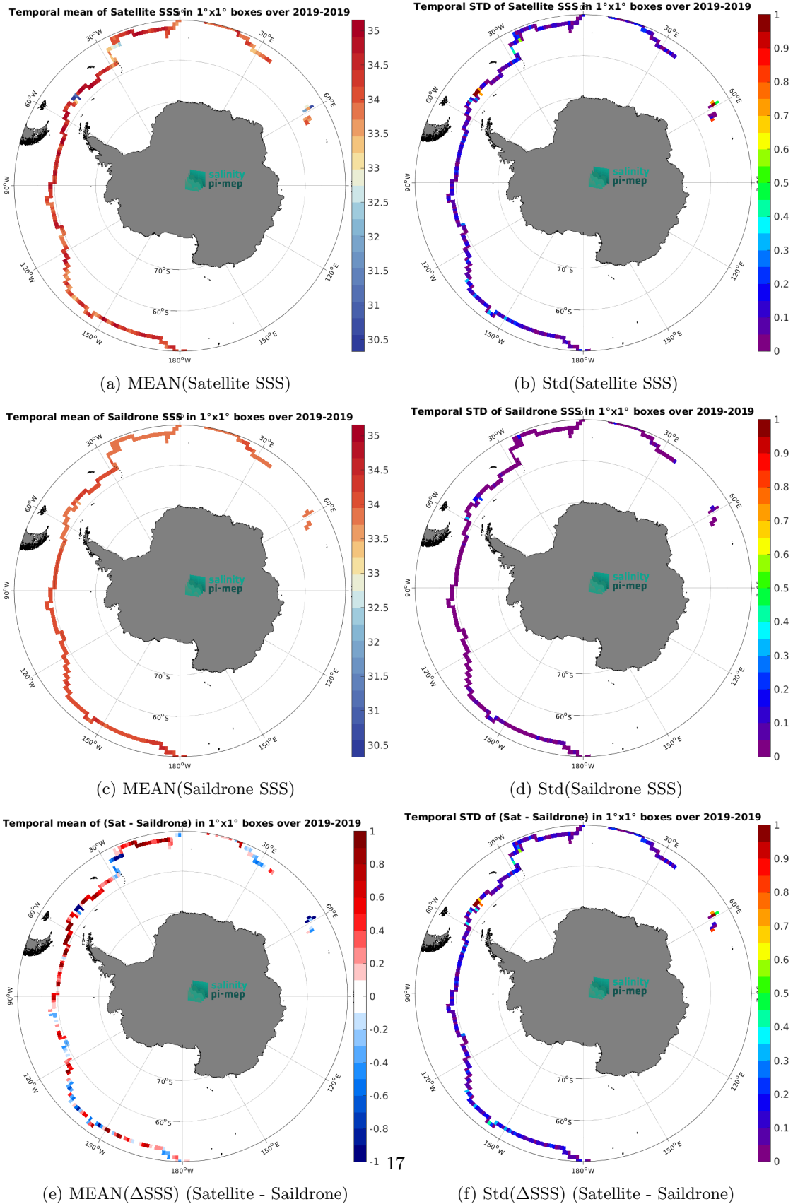
Figure 7: Temporal mean (left) and Std (right) of SSS from SMAP SSS L3 v5.0 - 8-Day running (JPL) (top), Saildrone (middle), and of \Delta SSS (Satellite - Saildrone). Only match-up pairs are used to generate these maps.
