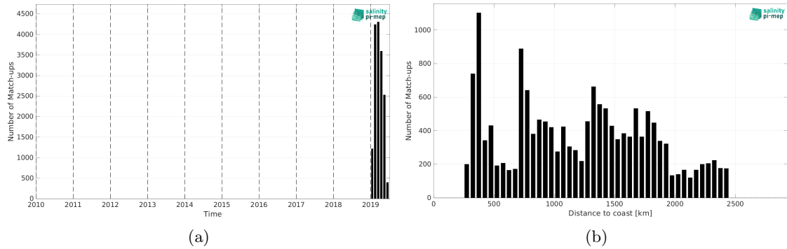
Figure 2: Number of match-ups between Saildrone and SMAP SSS L3 v5.0 - 8-Day running (JPL) SSS as a function of time (a) and as function of the distance to coast (b) over the Southern Ocean Pi-MEP region and for the full satellite product period.
