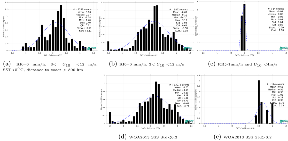
Figure 15: Normalized histogram of \Delta SSS (SMAP SSS L3 v5.0 - 8-Day running (JPL) - Saldrone) for 5 different subdatasets corresponding to: RR=0 mm/h, 3 < U_{10} < 12 m/s, SST > 5°C, distance to coast > 800 km (a), RR=0 mm/h, 3 < U_{10} < 12 m/s (b), RR > 1mm/h and U_{10} < 4 m/s (c), WOA2013 SSS Std < 0.2 (d), WOA2013 SSS Std > 0.2 (e).
