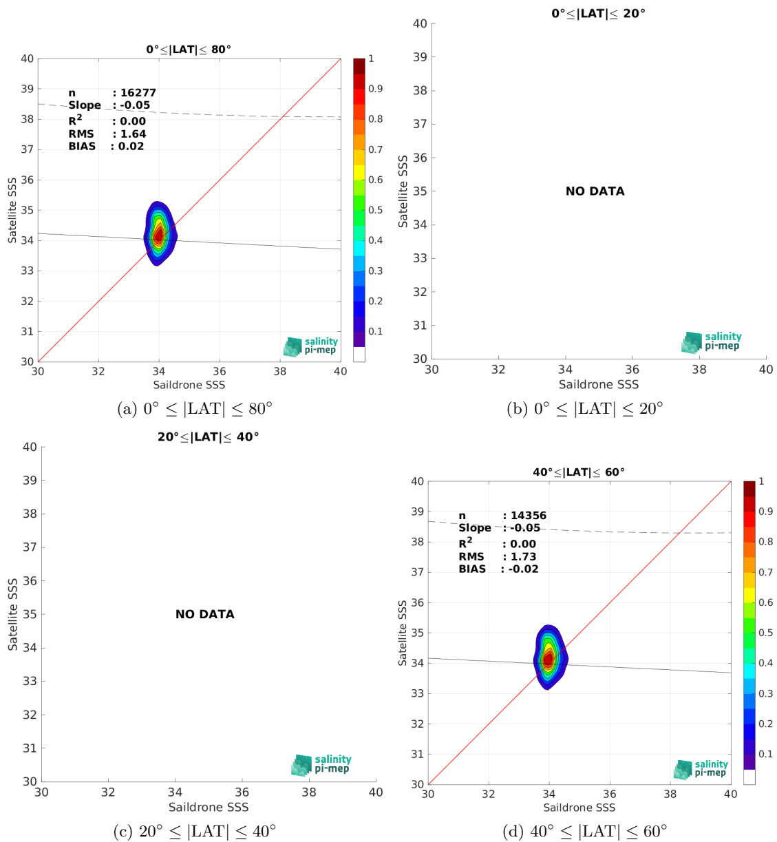
Figure 10: Contour maps of the concentration of SMAP SSS L3 v5.0 - 8-Day running (JPL) SSS (y-axis) versus Saildrone SSS (x-axis) at match-up pairs for different latitude bands. For each plot, the red line shows x=y . The black thin and dashed lines indicate a linear fit through the data cloud and the \pm 95\% confidence levels, respectively. The number match-up pairs n , the slope and R^2 coefficient of the linear fit, the root mean square (RMS) and the mean bias between satellite and in situ data are indicated for each latitude band in each plots.
