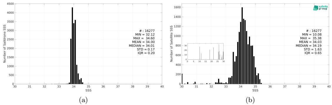
Figure 3: Histograms of SSS from Saildrone (a) and SMAP SSS L3 v5.0 - 8-Day running (JPL) (b) considering all match-up pairs per bins of 0.1 over the Southern Ocean Pi-MEP region and for the full satellite product period.
