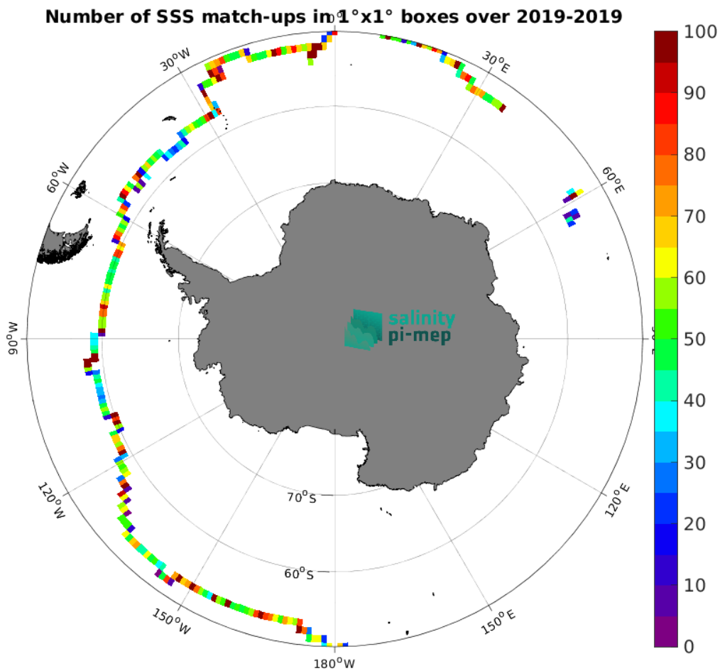
Figure 5: Number of SSS match-ups between Sairdrone SSS and the SMAP SSS L3 v5.0 - 8-Day running (JPL) SSS product for the Southern Ocean Pi-MEP region over 1^\circ \times 1^\circ boxes and for the full satellite product period.
