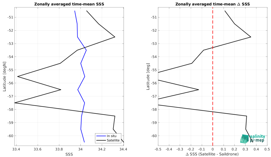
Figure 9: Left panel: Zonal mean SSS from SMAP SSS L3 v5.0 - 8-Day running (JPL) satellite product (black) and from Sairdrone (blue). Right panel: Zonal mean of \Delta SSS (Satellite - Sairdrone) for all the collected Pi-MEP match-up pairs estimated over the full satellite product period.
