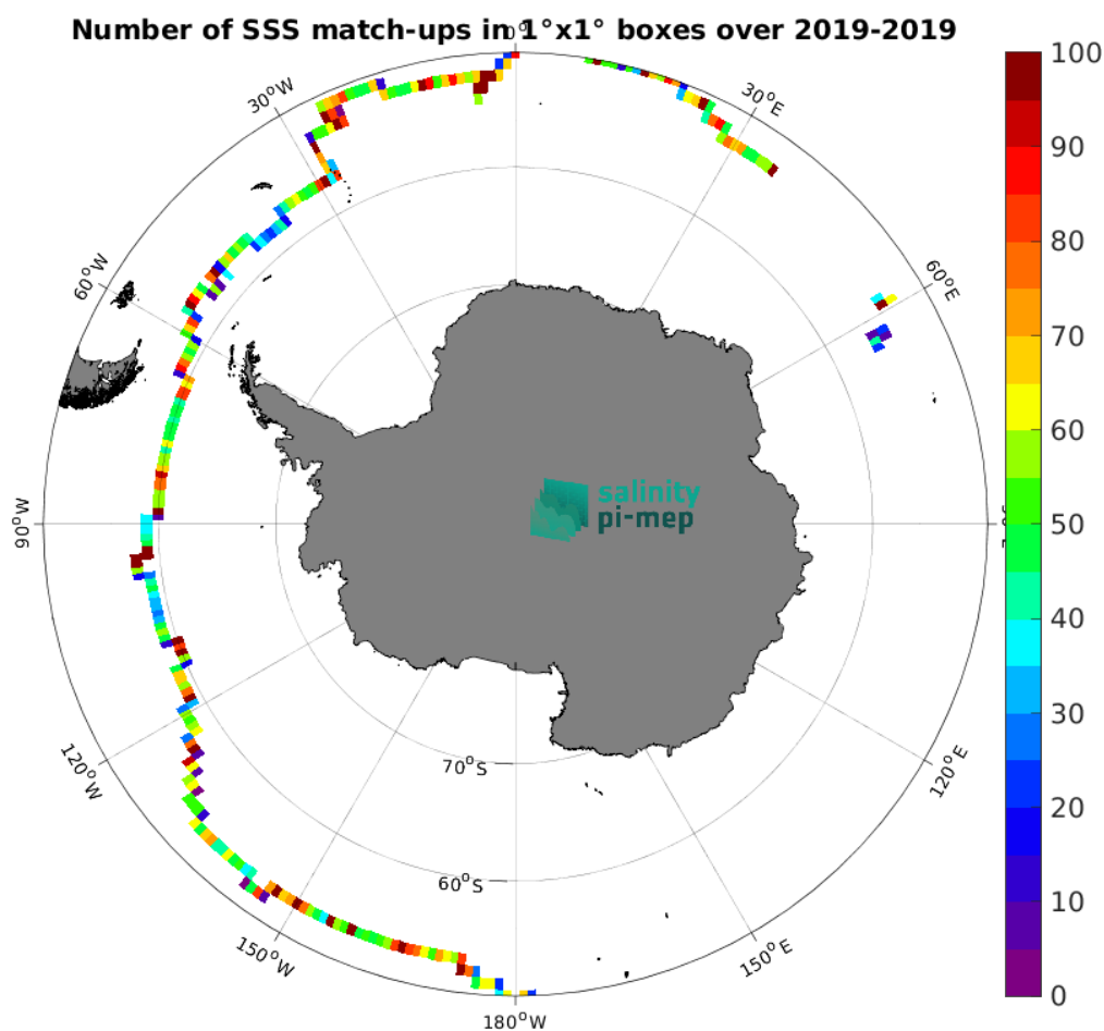
Figure 4: Number of SSS match-ups between Saildrone SSS and the SMAP SSS L3 v5.0 - 8-Day running (JPL) SSS product for the Southern Ocean Pi-MEP region over 1^\circ \times 1^\circ boxes and for the full satellite product period.
