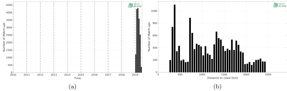
Figure 1: Number of match-ups between Saildrone and SMAP SSS L3 v5.0 - 8-Day running (JPL) SSS as a function of time (a) and as function of the distance to coast (b) over the Southern Ocean Pi-MEP region and for the full satellite product period.
