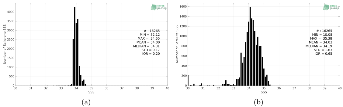
Figure 2: Histograms of SSS from Saildrone (a) and SMAP SSS L3 v5.0 - 8-Day running (JPL) (b) considering all match-up pairs per bins of 0.1 over the Southern Ocean Pi-MEP region and for the full satellite product period.
