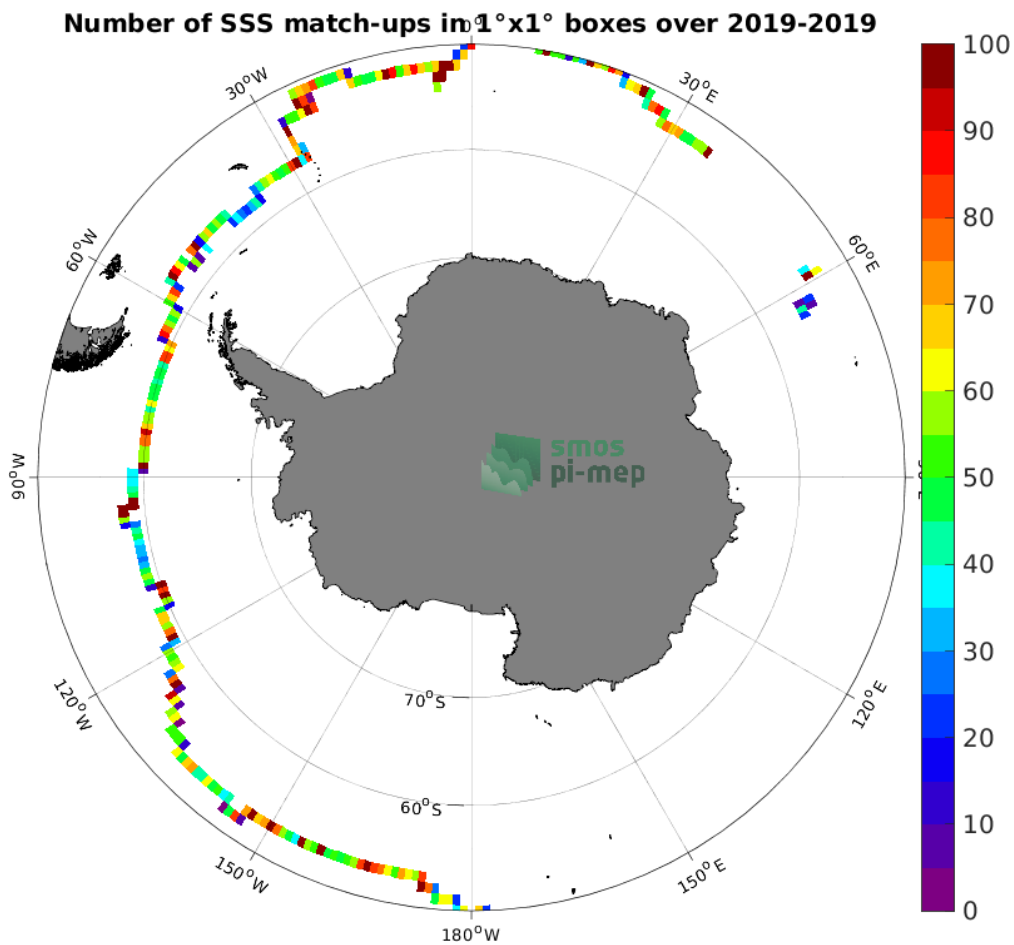
Figure 4: Number of SSS match-ups between Sairdrone SSS and the SMAP SSS L3 v5.0 - 8-Day running (JPL) SSS product for the Southern Ocean Pi-MEP region over 1^\circ \times 1^\circ boxes and for the full satellite product period.
