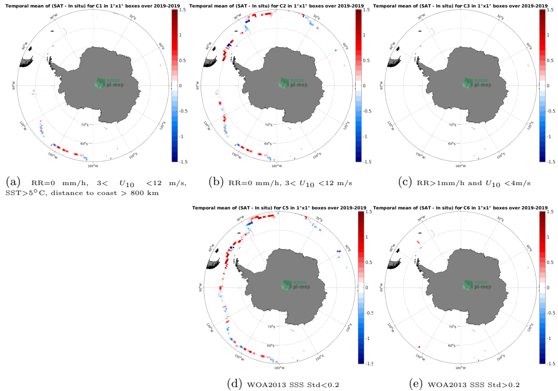
Figure 12: Temporal mean gridded over spatial boxes of size 1^{\circ}\times 1^{\circ} of \Delta\text{SSS} (SMAP SSS L3 v5.0 - 8-Day running (JPL) - Sairdrone) for 5 different subdatasets corresponding to:RR=0 mm/h, 3 < U_{10} < 12 m/s, SST >5^{\circ}\text{C} , distance to coast > 800 km (a), RR=0 mm/h, 3 < U_{10} < 12 m/s (b), RR >1 mm/h and U_{10} < 4 m/s (c), WOA2013 SSS Std <0.2 (d), WOA2013 SSS Std >0.2 (e).
