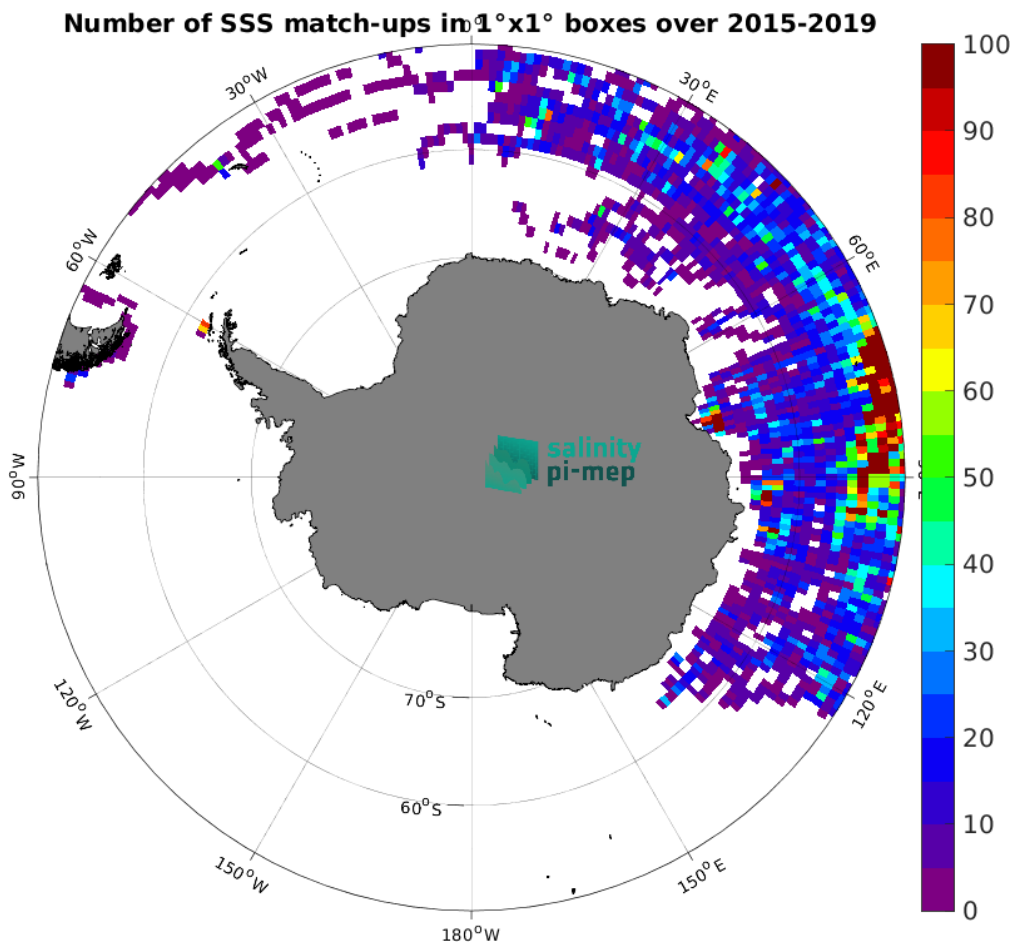
Figure 4: Number of SSS match-ups between Marine mammals SSS and the SMAP SSS L3 v5.0 - 8-Day running (JPL) SSS product for the Southern Ocean Pi-MEP region over 1^{\circ} \times 1^{\circ} boxes and for the full satellite product period.
