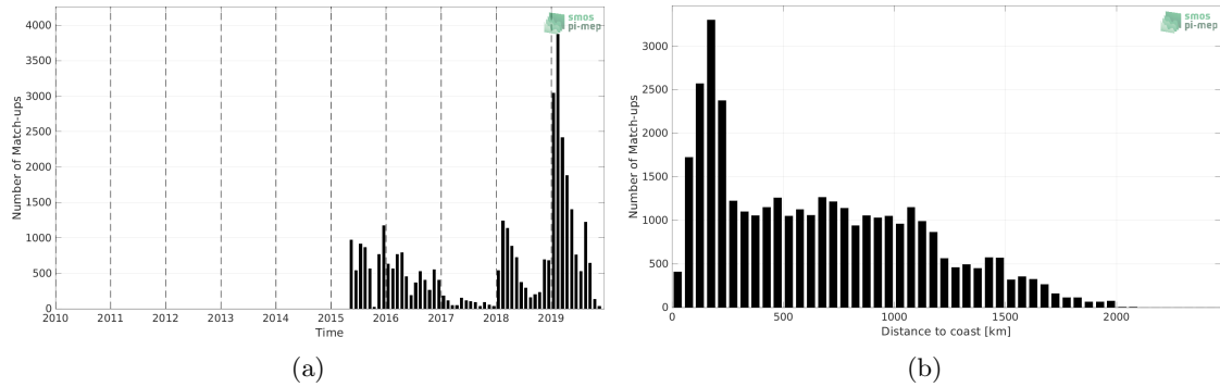
Figure 1: Number of match-ups between Marine mammals and SMAP SSS L3 v5.0 - 8-Day running (JPL) SSS as a function of time (a) and as function of the distance to coast (b) over the Southern Ocean Pi-MEP region and for the full satellite product period.
