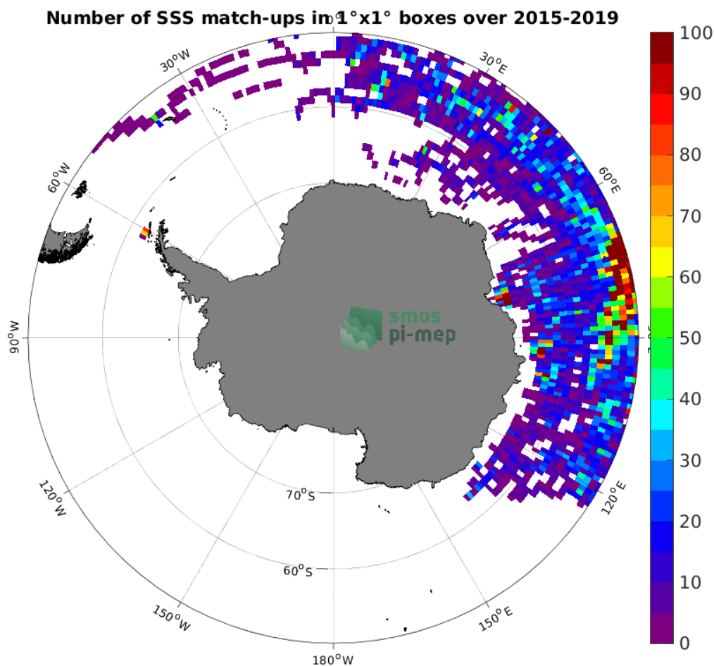
Figure 4: Number of SSS match-ups between Marine mammals SSS and the SMAP SSS L3 v5.0 - 8-Day running (JPL) SSS product for the Southern Ocean Pi-MEP region over 1^\circ \times 1^\circ boxes and for the full satellite product period.
