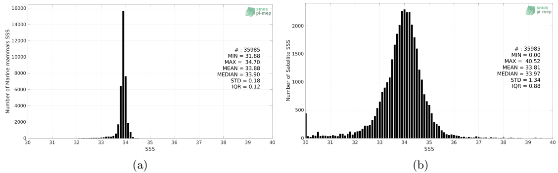
Figure 2: Histograms of SSS from Marine mammals (a) and SMAP SSS L3 v5.0 - 8-Day running (JPL) (b) considering all match-up pairs per bins of 0.1 over the Southern Ocean Pi-MEP region and for the full satellite product period.
