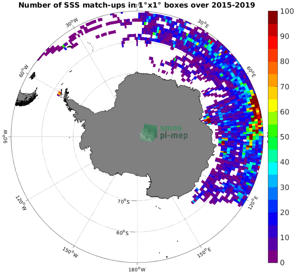
Figure 4: Number of SSS match-ups between Marine mammals SSS and the SMAP SSS L3 v5.0 - 8-Day running (JPL) SSS product for the Southern Ocean Pi-MEP region over 1^\circ \times 1^\circ boxes and for the full satellite product period.
