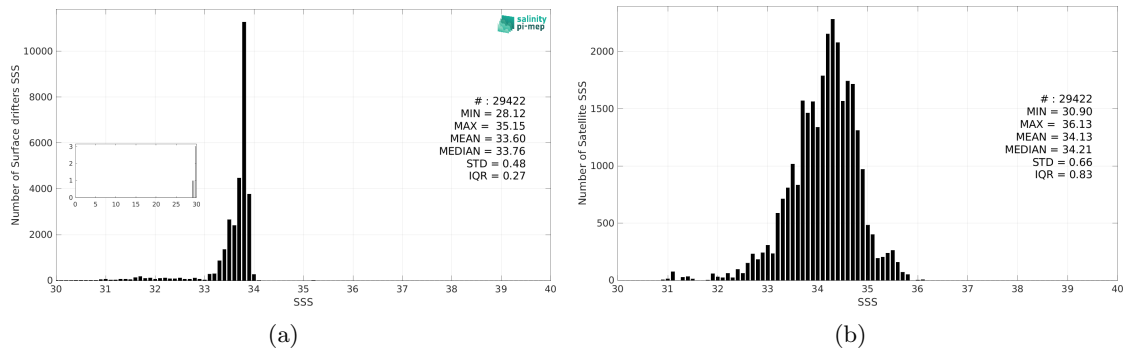
Figure 3: Histograms of SSS from Surface drifters (a) and SMAP SSS L3 v5.0 - 8-Day running (JPL) (b) considering all match-up pairs per bins of 0.1 over the Southern Ocean Pi-MEP region and for the full satellite product period.
