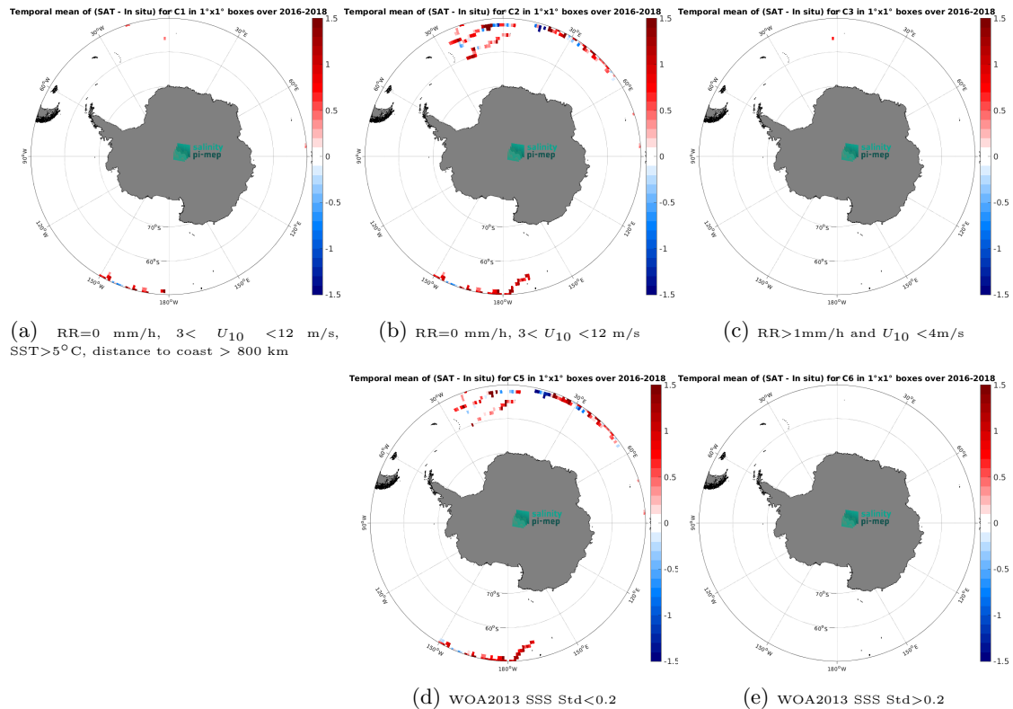
Figure 13: Temporal mean gridded over spatial boxes of size 1^\circ \times 1^\circ of \Delta SSS (SMAP SSS L3 v5.0 - 8-Day running (JPL) - Surface drifters) for 5 different subdatasets corresponding to:RR=0 mm/h, 3 < U_{10} < 12 m/s, SST >5^\circ\text{C} , distance to coast > 800 km (a), RR=0 mm/h, 3 < U_{10} < 12 m/s (b), RR >1 mm/h and U_{10} < 4 m/s (c), WOA2013 SSS Std <0.2 (d), WOA2013 SSS Std >0.2 (e).
