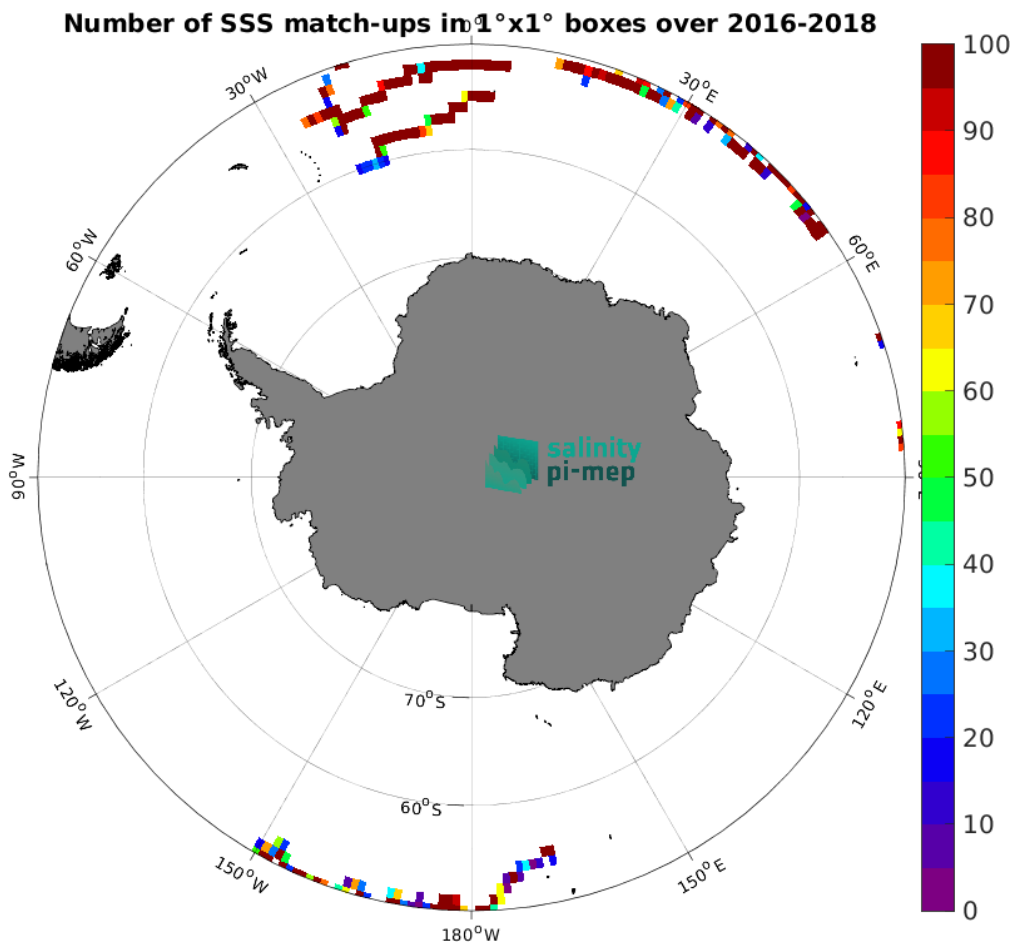
Figure 4: Number of SSS match-ups between Surface drifters SSS and the SMAP SSS L3 v5.0 - 8-Day running (JPL) SSS product for the Southern Ocean Pi-MEP region over 1^\circ \times 1^\circ boxes and for the full satellite product period.
