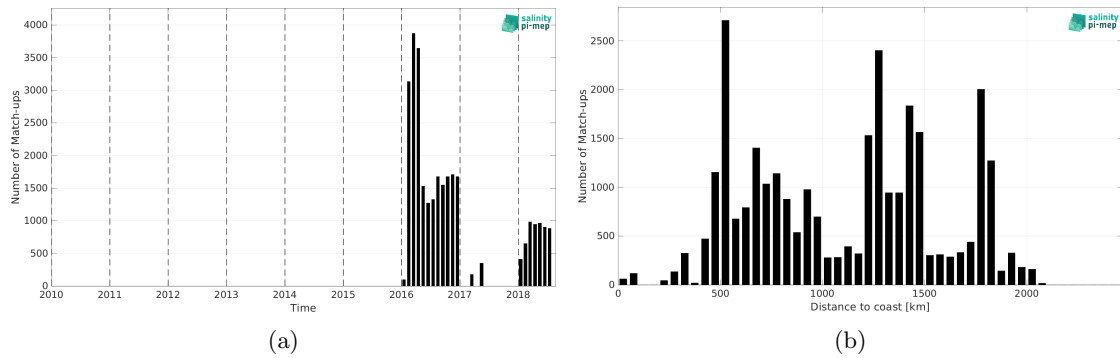
Figure 2: Number of match-ups between Surface drifters and SMAP SSS L3 v5.0 - 8-Day running (JPL) SSS as a function of time (a) and as function of the distance to coast (b) over the Southern Ocean Pi-MEP region and for the full satellite product period.
