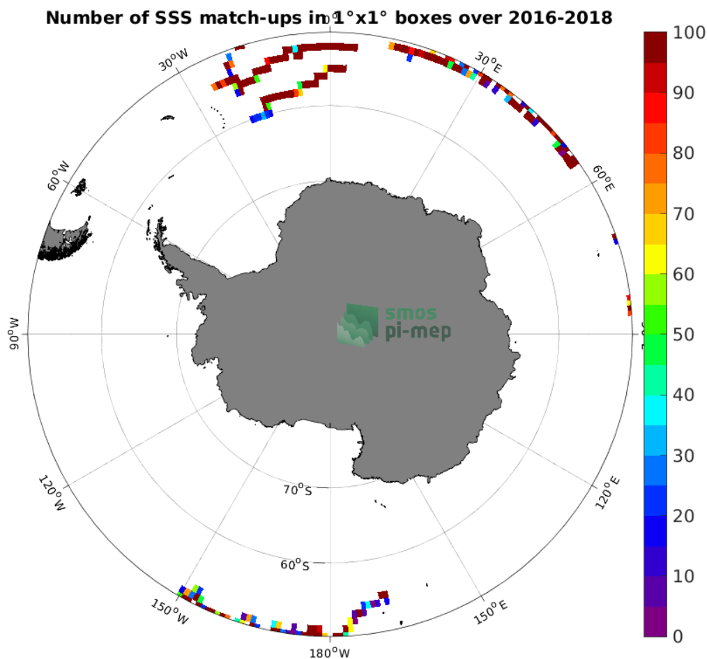
Figure 3: Number of SSS match-ups between Surface drifters SSS and the SMAP SSS L3 v5.0 - 8-Day running (JPL) SSS product for the Southern Ocean Pi-MEP region over 1^\circ \times 1^\circ boxes and for the full satellite product period.
