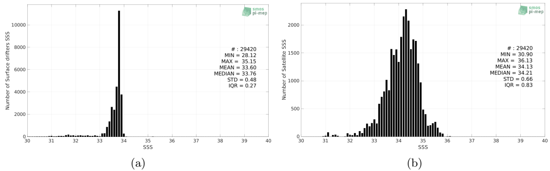
Figure 2: Histograms of SSS from Surface drifters (a) and SMAP SSS L3 v5.0 - 8-Day running (JPL) (b) considering all match-up pairs per bins of 0.1 over the Southern Ocean Pi-MEP region and for the full satellite product period.
