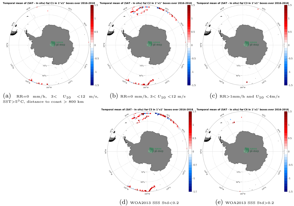
Figure 11: Temporal mean gridded over spatial boxes of size 1^{\circ}\times 1^{\circ} of \Delta\text{SSS} (SMAP SSS L3 v5.0 - 8-Day running (JPL) - Surface drifters) for 5 different subdatasets corresponding to:RR=0 mm/h, 3 < U_{10} < 12 m/s, SST >5^{\circ}\text{C} , distance to coast > 800 km (a), RR=0 mm/h, 3 < U_{10} < 12 m/s (b), RR >1 mm/h and U_{10} < 4 m/s (c), WOA2013 SSS Std <0.2 (d), WOA2013 SSS Std >0.2 (e).
