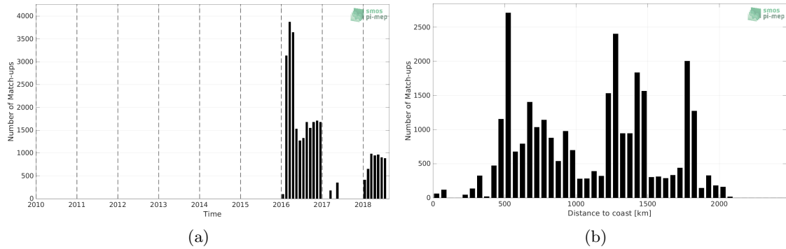
Figure 1: Number of match-ups between Surface drifters and SMAP SSS L3 v5.0 - 8-Day running (JPL) SSS as a function of time (a) and as function of the distance to coast (b) over the Southern Ocean Pi-MEP region and for the full satellite product period.
