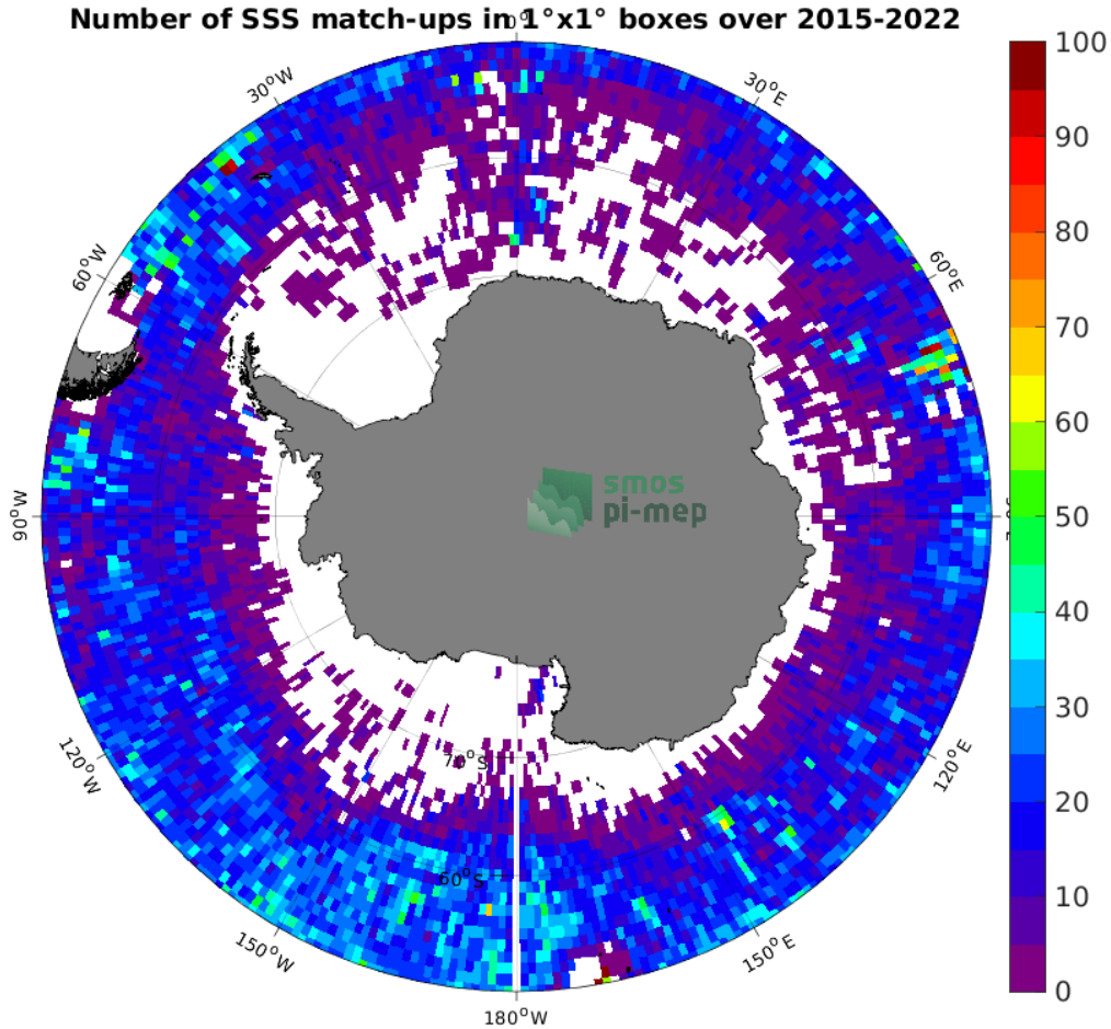
Figure 4: Number of SSS match-ups between Argo SSS and the SMAP SSS L3 v5.0 - 8-Day running (JPL) SSS product for the Southern Ocean Pi-MEP region over 1^\circ \times 1^\circ boxes and for the full satellite product period.
