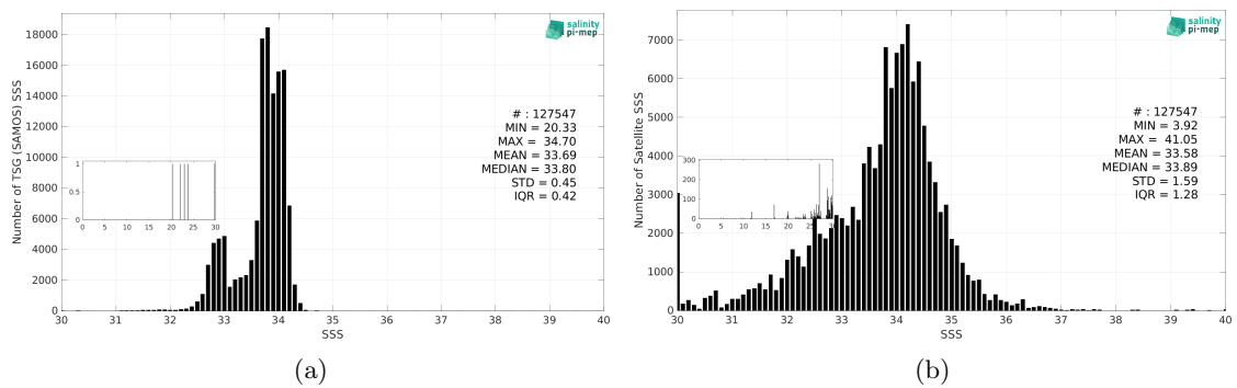
Figure 3: Histograms of SSS from TSG (SAMOS) (a) and SMAP SSS L3 v5.0 - Monthly (JPL) (b) considering all match-up pairs per bins of 0.1 over the Southern Ocean Pi-MEP region and for the full satellite product period.
