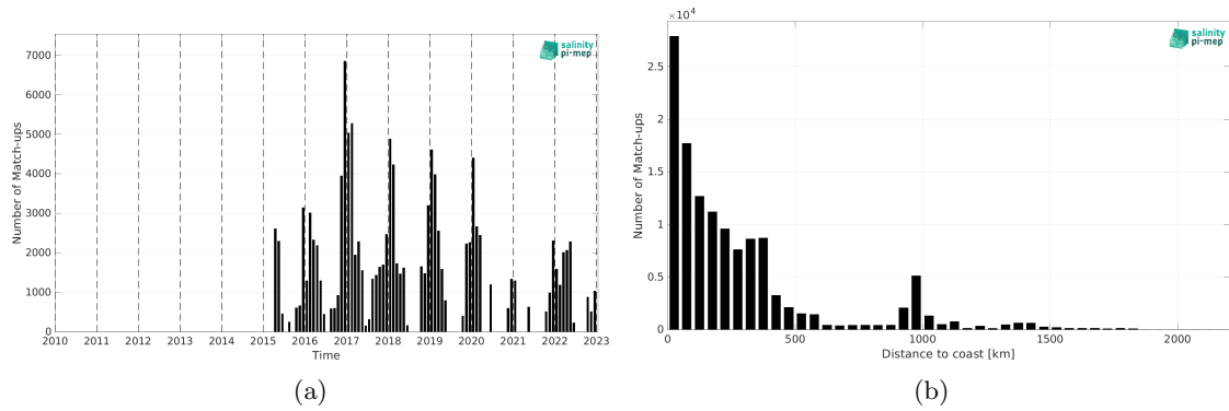
Figure 2: Number of match-ups between TSG (SAMOS) and SMAP SSS L3 v5.0 - Monthly (JPL) SSS as a function of time (a) and as function of the distance to coast (b) over the Southern Ocean Pi-MEP region and for the full satellite product period.
