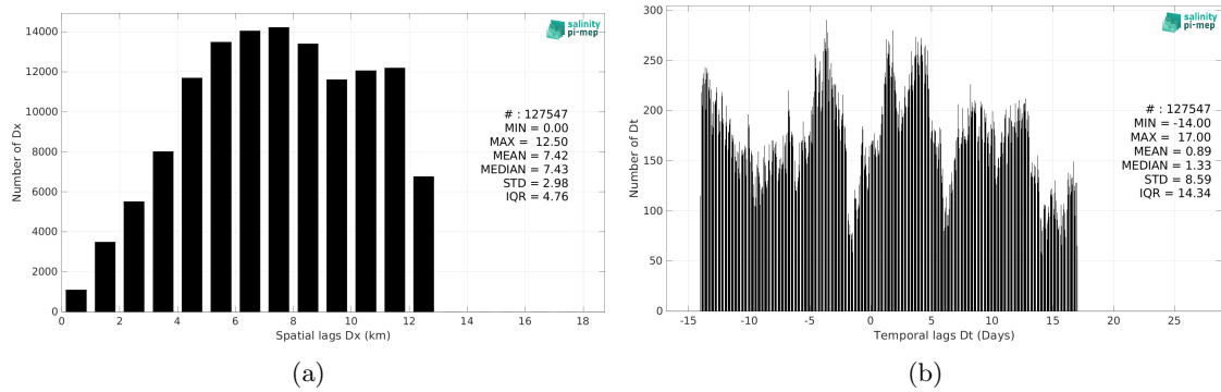
Figure 6: Histograms of the spatial (a) and temporal (b) lags between the location/time of the TSG (SAMOS) measurement and the date of the corresponding SMAP SSS L3 v5.0 - Monthly (JPL) SSS pixel.
