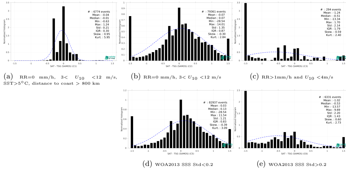
Figure 15: Normalized histogram of \Delta SSS (SMAP SSS L3 v5.0 - Monthly (JPL) - TSG (SAMOS)) for 5 different subdatasets corresponding to: RR=0 mm/h, 3 < U_{10} < 12 m/s, SST > 5°C, distance to coast > 800 km (a), RR=0 mm/h, 3 < U_{10} < 12 m/s (b), RR > 1mm/h and U_{10} < 4 m/s (c), WOA2013 SSS Std < 0.2 (d), WOA2013 SSS Std > 0.2 (e).
