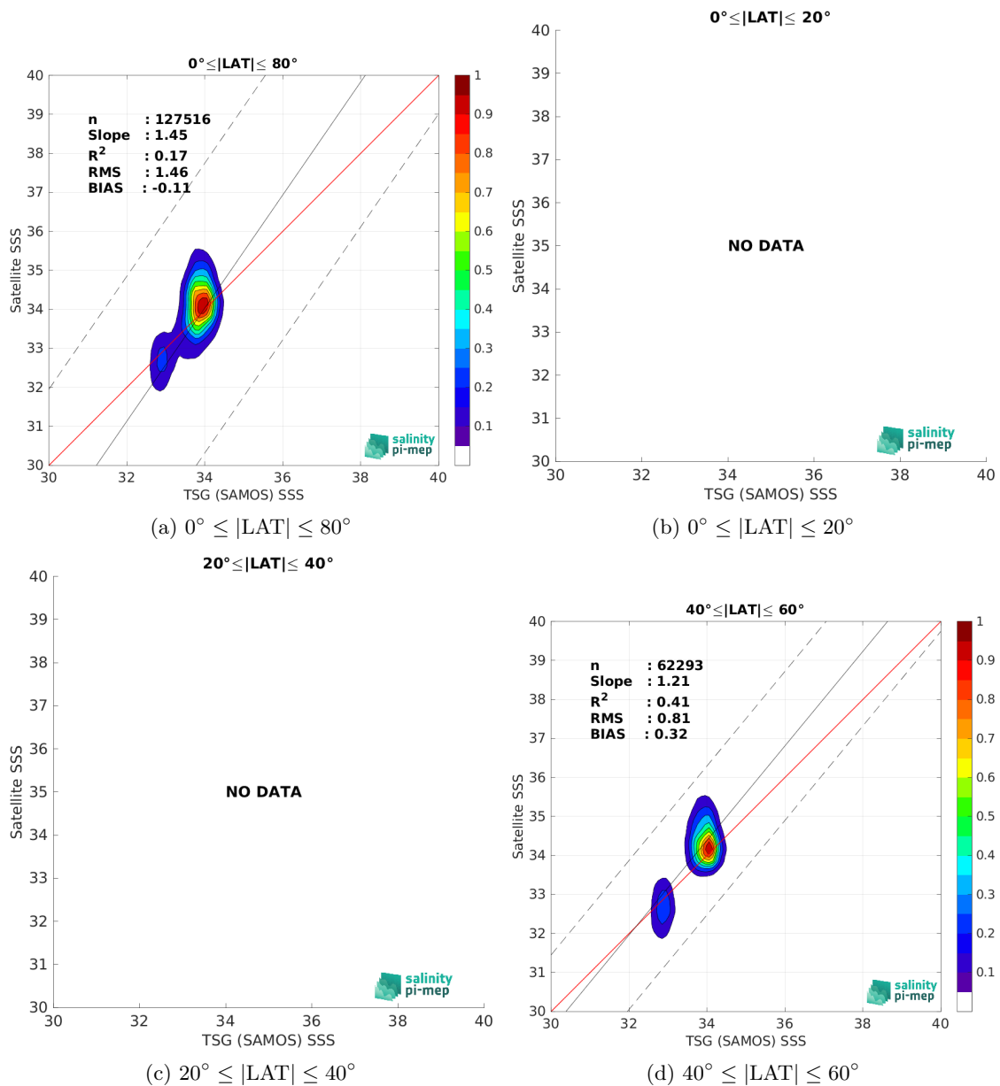
Figure 10: Contour maps of the concentration of SMAP SSS L3 v5.0 - Monthly (JPL) SSS (y-axis) versus TSG (SAMOS) SSS (x-axis) at match-up pairs for different latitude bands. For each plot, the red line shows x=y . The black thin and dashed lines indicate a linear fit through the data cloud and the \pm 95\% confidence levels, respectively. The number match-up pairs n , the slope and R^2 coefficient of the linear fit, the root mean square (RMS) and the mean bias between satellite and in situ data are indicated for each latitude band in each plots.
