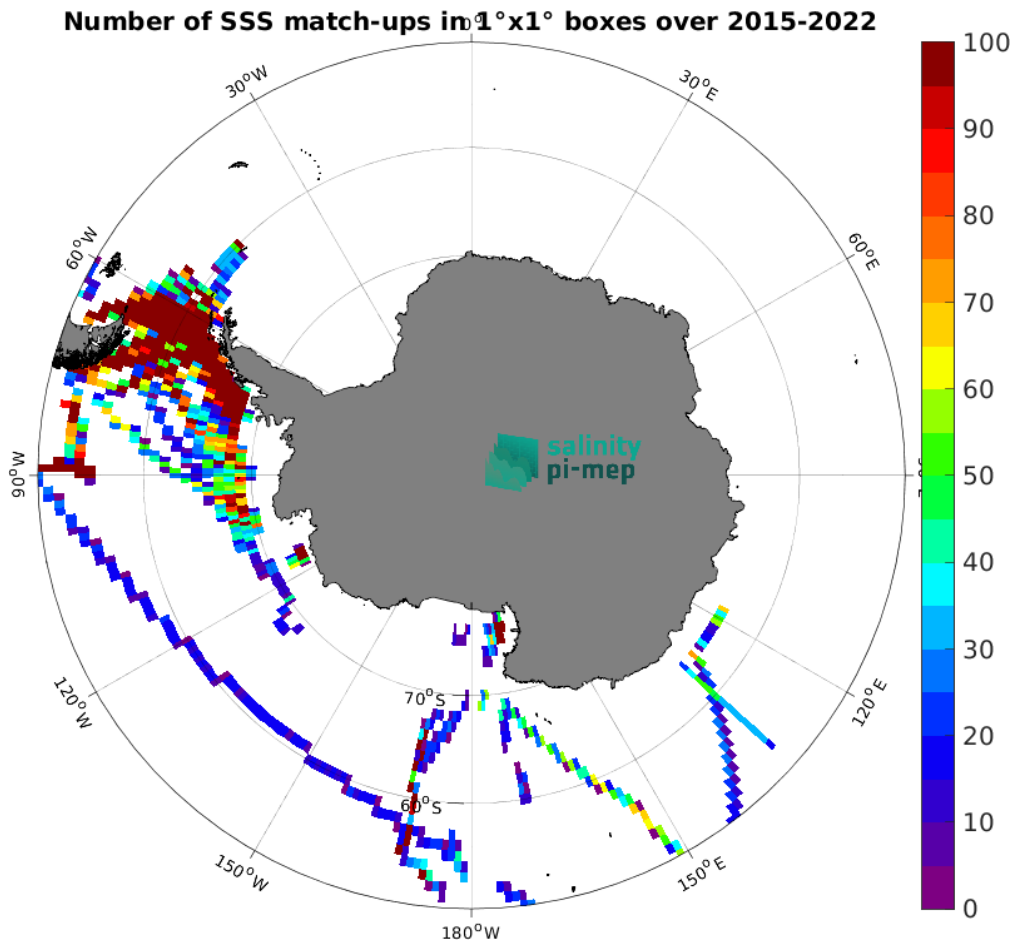
Figure 5: Number of SSS match-ups between TSG (SAMOS) SSS and the SMAP SSS L3 v5.0 - Monthly (JPL) SSS product for the Southern Ocean Pi-MEP region over 1^\circ \times 1^\circ boxes and for the full satellite product period.
