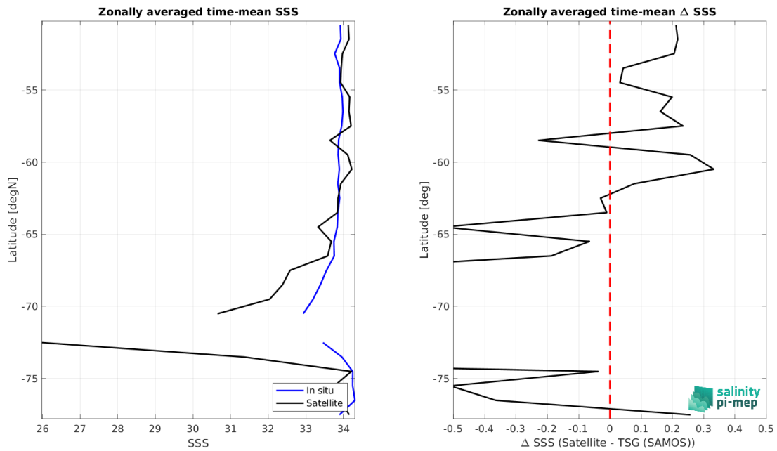
Figure 9: Left panel: Zonal mean SSS from SMAP SSS L3 v5.0 - Monthly (JPL) satellite product (black) and from TSG (SAMOS) (blue). Right panel: Zonal mean of \Delta SSS (Satellite - TSG (SAMOS)) for all the collected Pi-MEP match-up pairs estimated over the full satellite product period.
