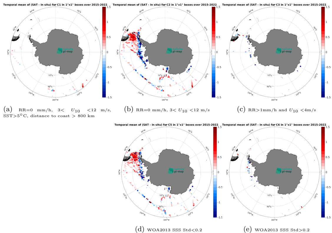
Figure 14: Temporal mean gridded over spatial boxes of size 1^\circ \times 1^\circ of \Delta SSS (SMAP SSS L3 v5.0 - Monthly (JPL) - TSG (SAMOS)) for 5 different subdatasets corresponding to:RR=0 mm/h, 3 < U_{10} < 12 m/s, SST>5°C, distance to coast > 800 km (a), RR=0 mm/h, 3 < U_{10} < 12 m/s (b), RR>1mm/h and U_{10} < 4 m/s (c), WOA2013 SSS Std<0.2 (d), WOA2013 SSS Std>0.2 (e).
