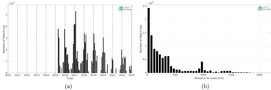
Figure 1: Number of match-ups between TSG (SAMOS) and SMAP SSS L3 v5.0 - Monthly (JPL) SSS as a function of time (a) and as function of the distance to coast (b) over the Southern Ocean Pi-MEP region and for the full satellite product period.
