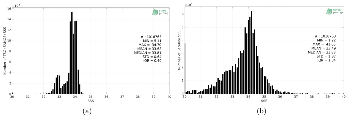
Figure 2: Histograms of SSS from TSG (SAMOS) (a) and SMAP SSS L3 v5.0 - Monthly (JPL) (b) considering all match-up pairs per bins of 0.1 over the Southern Ocean Pi-MEP region and for the full satellite product period.
