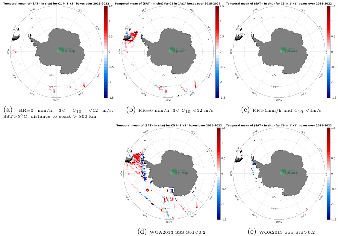
Figure 12: Temporal mean gridded over spatial boxes of size 1^{\circ}\times 1^{\circ} of \Delta\text{SSS} (SMAP SSS L3 v5.0 - Monthly (JPL) - TSG (SAMOS)) for 5 different subdatasets corresponding to:RR=0 mm/h, 3 < U_{10} < 12 m/s, SST >5^{\circ}\text{C} , distance to coast > 800 km (a), RR=0 mm/h, 3 < U_{10} < 12 m/s (b), RR >1 mm/h and U_{10} < 4 m/s (c), WOA2013 SSS Std <0.2 (d), WOA2013 SSS Std >0.2 (e).
