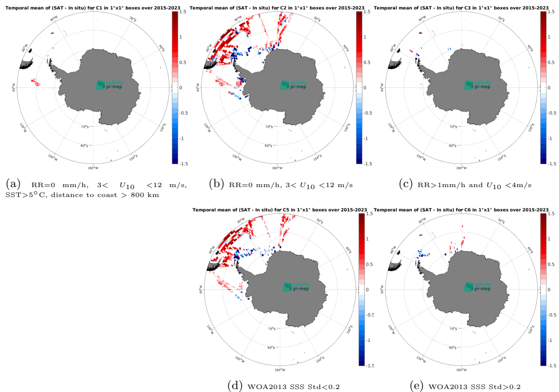
Figure 14: Temporal mean gridded over spatial boxes of size 1^\circ \times 1^\circ of \Delta\text{SSS} (SMAP SSS L3 v5.0 - Monthly (JPL) - TSG (Polarstern)) for 5 different subdatasets corresponding to: RR=0 mm/h, 3 < U_{10} < 12 m/s, \text{SST} > 5^\circ\text{C} , distance to coast > 800 km (a), RR=0 mm/h, 3 < U_{10} < 12 m/s (b), RR>1mm/h and U_{10} < 4\text{m/s} (c), WOA2013 SSS Std<0.2 (d), WOA2013 SSS Std>0.2 (e).
