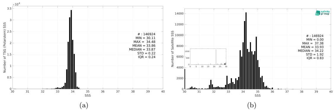
Figure 3: Histograms of SSS from TSG (Polarstern) (a) and SMAP SSS L3 v5.0 - Monthly (JPL) (b) considering all match-up pairs per bins of 0.1 over the Southern Ocean Pi-MEP region and for the full satellite product period.
