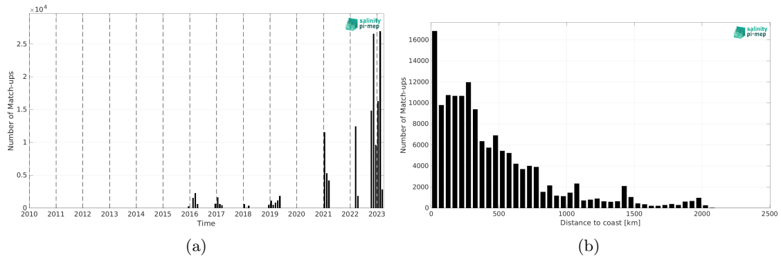
Figure 2: Number of match-ups between TSG (Polarstern) and SMAP SSS L3 v5.0 - Monthly (JPL) SSS as a function of time (a) and as function of the distance to coast (b) over the Southern Ocean Pi-MEP region and for the full satellite product period.
