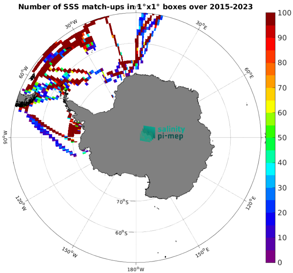
Figure 5: Number of SSS match-ups between TSG (Polarstern) SSS and the SMAP SSS L3 v5.0 - Monthly (JPL) SSS product for the Southern Ocean Pi-MEP region over 1^\circ \times 1^\circ boxes and for the full satellite product period.
