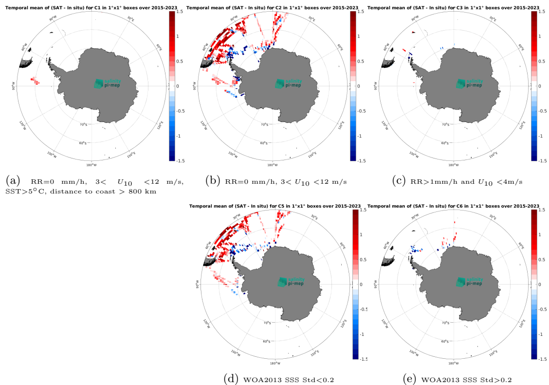
Figure 14: Temporal mean gridded over spatial boxes of size 1^\circ \times 1^\circ of \Delta SSS (SMAP SSS L3 v5.0 - Monthly (JPL) - TSG (Polarstern)) for 5 different subdatasets corresponding to: RR=0 mm/h, 3 < U_{10} < 12 m/s, SST > 5^\circ\text{C} , distance to coast > 800 km (a), RR=0 mm/h, 3 < U_{10} < 12 m/s (b), RR > 1 mm/h and U_{10} < 4 m/s (c), WOA2013 SSS Std < 0.2 (d), WOA2013 SSS Std > 0.2 (e).
