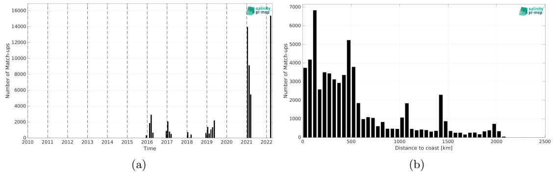
Figure 1: Number of match-ups between TSG (Polarstern) and SMAP SSS L3 v5.0 - Monthly (JPL) SSS as a function of match-up time (a) and as function of the distance to coast (b) over the Southern Ocean Pi-MEP region and for the full satellite product period.
