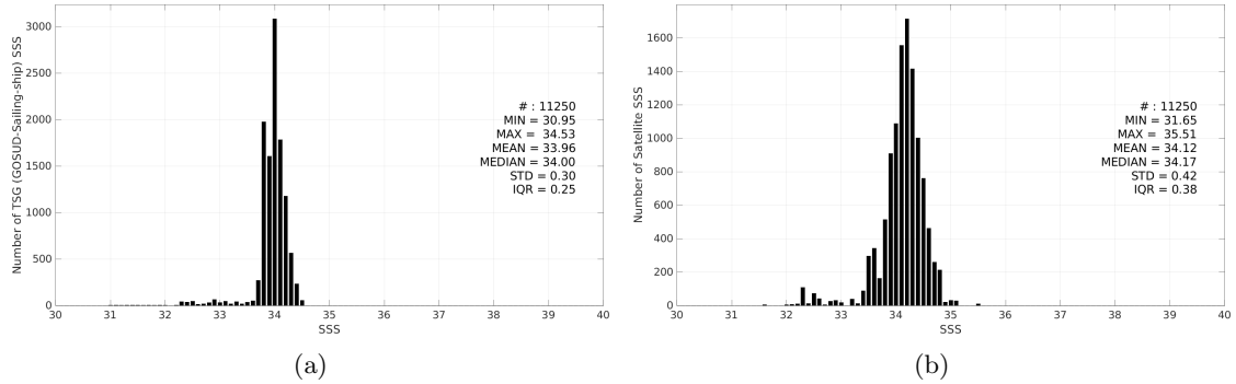
Figure 3: Histograms of SSS from TSG (GOSUD-Sailing-ship) (a) and SMAP SSS L3 v5.0 - Monthly (JPL) (b) considering all match-up pairs per bins of 0.1 over the Southern Ocean Pi-MEP region and for the full satellite product period.
