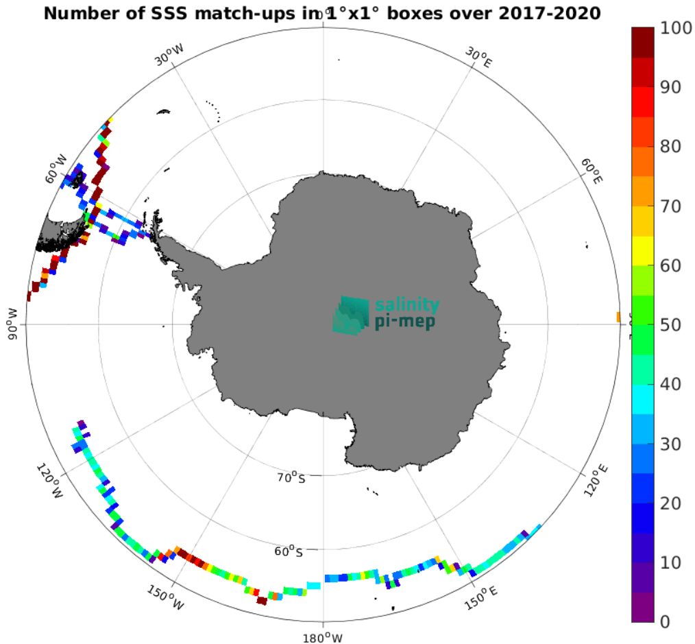
Figure 5: Number of SSS match-ups between TSG (GOSUD-Sailing-ship) SSS and the SMAP SSS L3 v5.0 - Monthly (JPL) SSS product for the Southern Ocean Pi-MEP region over 1^\circ \times 1^\circ boxes and for the full satellite product period.
