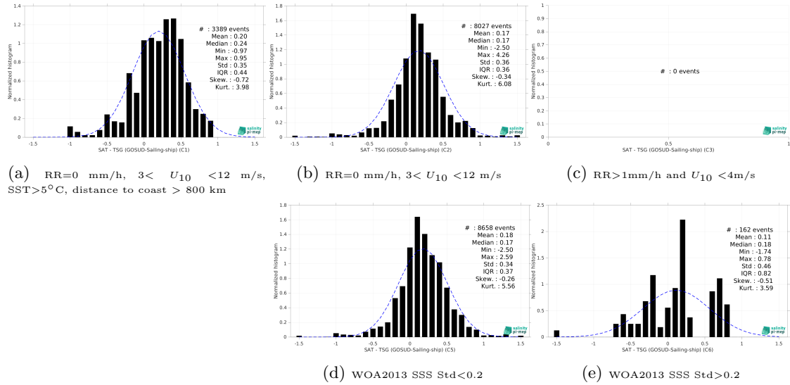
Figure 15: Normalized histogram of \Delta SSS (SMAP SSS L3 v5.0 - Monthly (JPL) - TSG (GOSUD-Sailing-ship)) for 5 different subdatasets corresponding to: RR=0 mm/h, 3 < U_{10} < 12 m/s, SST >5^{\circ}\text{C} , distance to coast > 800 km (a), RR=0 mm/h, 3 < U_{10} < 12 m/s (b), RR >1 mm/h and U_{10} < 4 m/s (c), WOA2013 SSS Std <0.2 (d), WOA2013 SSS Std >0.2 (e).
