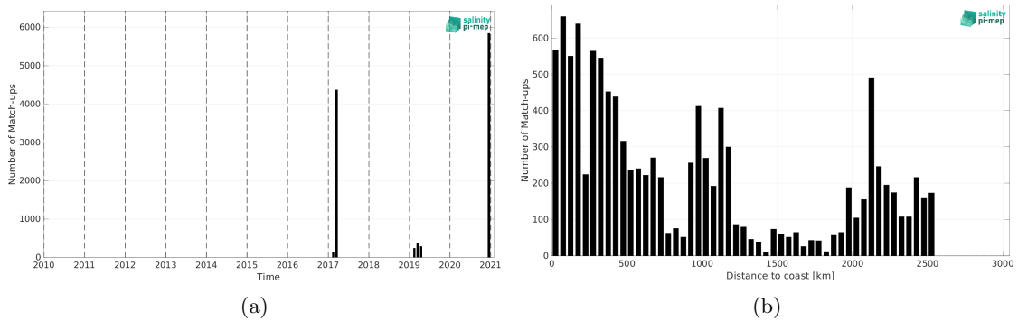
Figure 2: Number of match-ups between TSG (GOSUD-Sailing-ship) and SMAP SSS L3 v5.0 - Monthly (JPL) SSS as a function of time (a) and as function of the distance to coast (b) over the Southern Ocean Pi-MEP region and for the full satellite product period.
