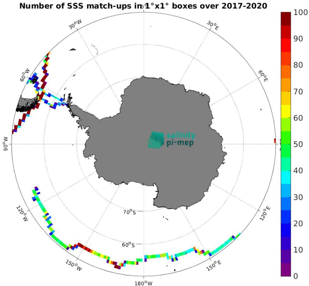
Figure 4: Number of SSS match-ups between TSG (GOSUD-Sailing-ship) SSS and the SMAP SSS L3 v5.0 - Monthly (JPL) SSS product for the Southern Ocean Pi-MEP region over 1^\circ \times 1^\circ boxes and for the full satellite product period.
