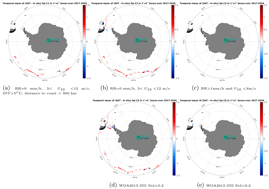
Figure 12: Temporal mean gridded over spatial boxes of size 1^\circ \times 1^\circ of \Delta\text{SSS} (SMAP SSS L3 v5.0 - Monthly (JPL) - TSG (GOSUD-Sailing-ship)) for 5 different subdatasets corresponding to: RR=0 mm/h, 3 < U_{10} < 12 m/s, SST > 5^\circ\text{C} , distance to coast > 800 km (a), RR=0 mm/h, 3 < U_{10} < 12 m/s (b), RR > 1 mm/h and U_{10} < 4 m/s (c), WOA2013 SSS Std < 0.2 (d), WOA2013 SSS Std > 0.2 (e).
