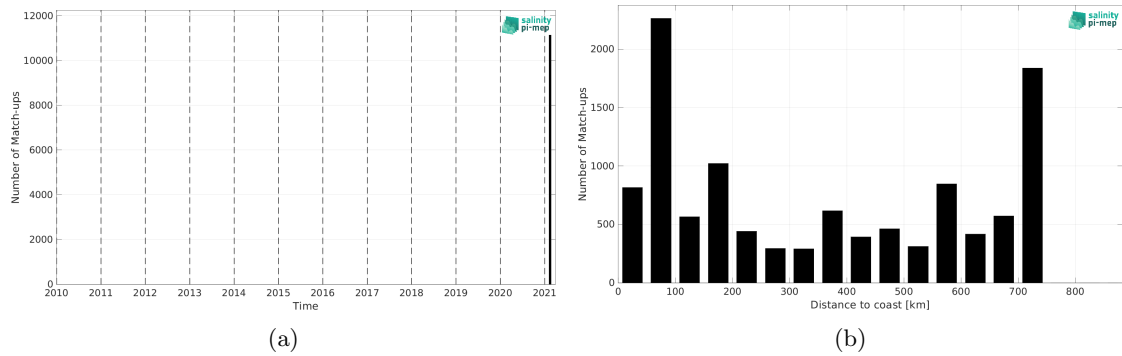
Figure 2: Number of match-ups between TSG (GOSUD-Research-vessel) and SMAP SSS L3 v5.0 - Monthly (JPL) SSS as a function of time (a) and as function of the distance to coast (b) over the Southern Ocean Pi-MEP region and for the full satellite product period.
