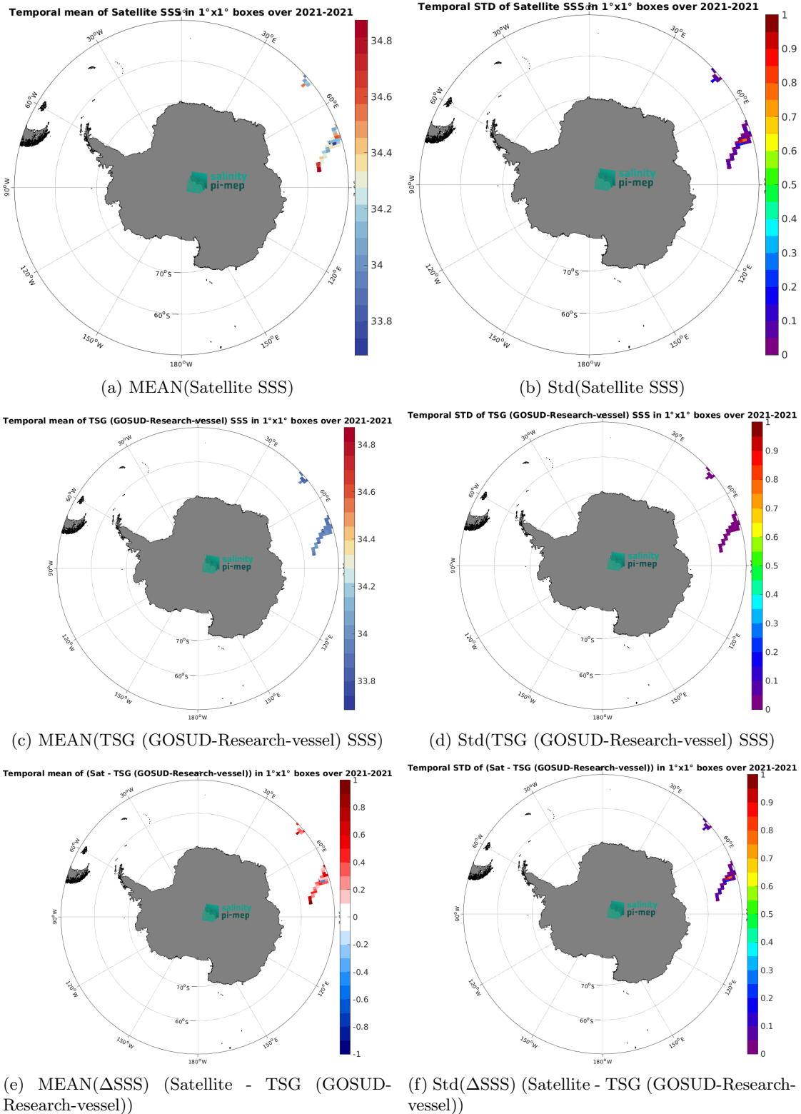
Figure 7: Temporal mean (left) and Std (right) of SSS from SMAP SSS L3 v5.0 - Monthly (JPL) (top), TSG (GOSUD-Research-vessel) (middle), and of \Delta SSS (Satellite - TSG (GOSUD-Research-vessel)). Only match-up pairs are used to generate these maps.
