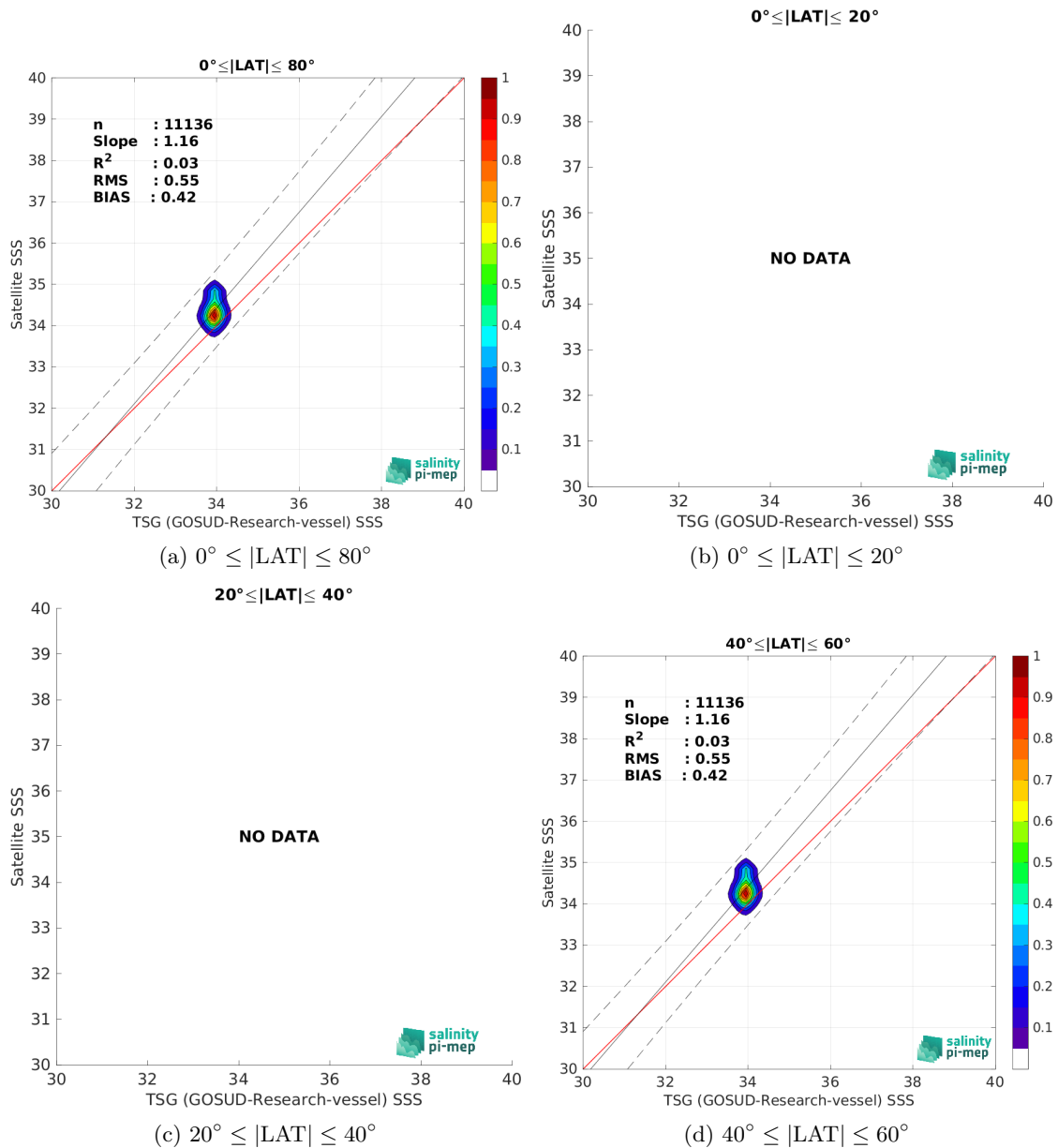
Figure 10: Contour maps of the concentration of SMAP SSS L3 v5.0 - Monthly (JPL) SSS (y-axis) versus TSG (GOSUD-Research-vessel) SSS (x-axis) at match-up pairs for different latitude bands. For each plot, the red line shows x=y . The black thin and dashed lines indicate a linear fit through the data cloud and the \pm 95\% confidence levels, respectively. The number match-up pairs n , the slope and R^2 coefficient of the linear fit, the root mean square (RMS) and the mean bias between satellite and in situ data are indicated for each latitude band in each plots.
