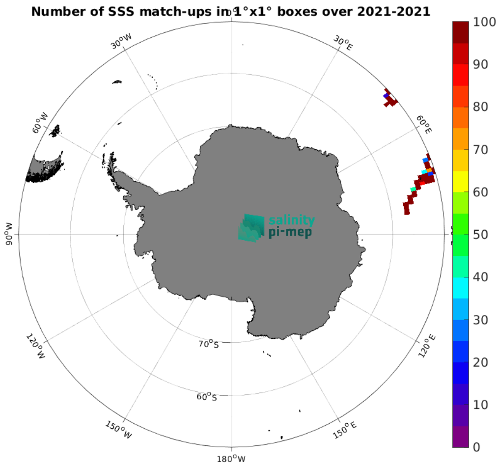
Figure 4: Number of SSS match-ups between TSG (GOSUD-Research-vessel) SSS and the SMAP SSS L3 v5.0 - Monthly (JPL) SSS product for the Southern Ocean Pi-MEP region over 1^\circ \times 1^\circ boxes and for the full satellite product period.
