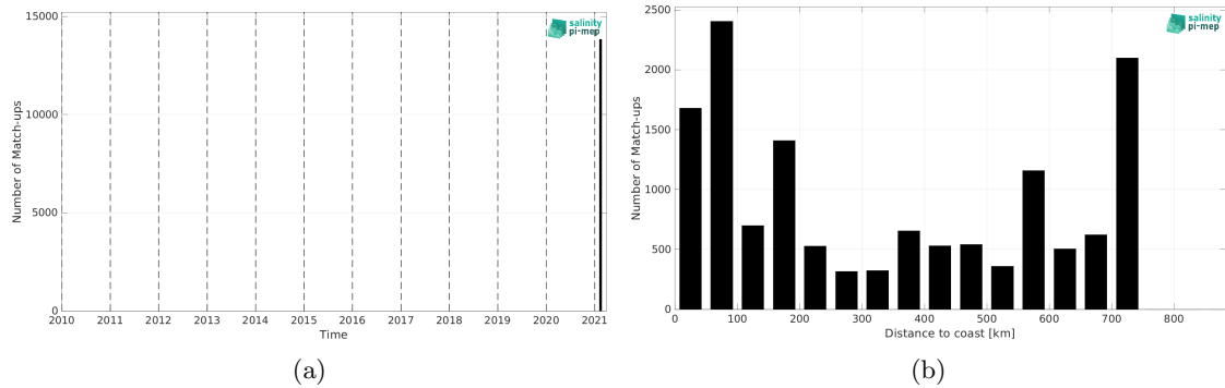
Figure 1: Number of match-ups between TSG (GOSUD-Research-vessel) and SMAP SSS L3 v5.0 - Monthly (JPL) SSS as a function of time (a) and as function of the distance to coast (b) over the Southern Ocean Pi-MEP region and for the full satellite product period.
