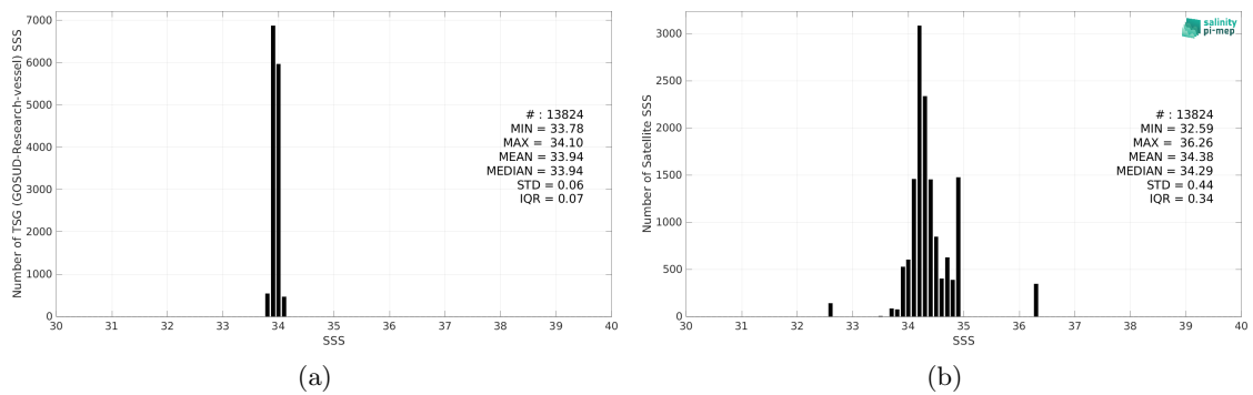
Figure 2: Histograms of SSS from TSG (GOSUD-Research-vessel) (a) and SMAP SSS L3 v5.0 - Monthly (JPL) (b) considering all match-up pairs per bins of 0.1 over the Southern Ocean Pi-MEP region and for the full satellite product period.
