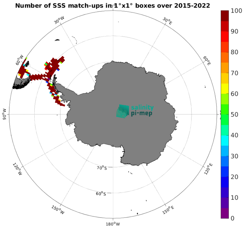
Figure 5: Number of SSS match-ups between TSG (CSIC-UTM) SSS and the SMAP SSS L3 v5.0 - Monthly (JPL) SSS product for the Southern Ocean Pi-MEP region over 1^{\circ} \times 1^{\circ} boxes and for the full satellite product period.
