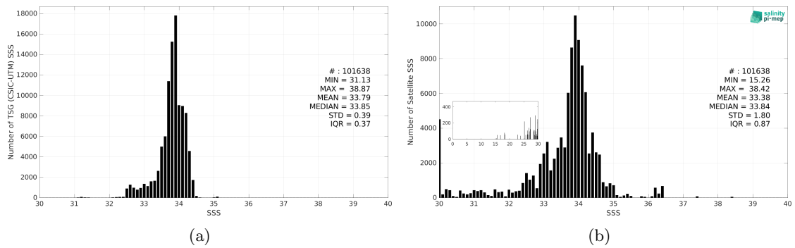
Figure 3: Histograms of SSS from TSG (CSIC-UTM) (a) and SMAP SSS L3 v5.0 - Monthly (JPL) (b) considering all match-up pairs per bins of 0.1 over the Southern Ocean Pi-MEP region and for the full satellite product period.
