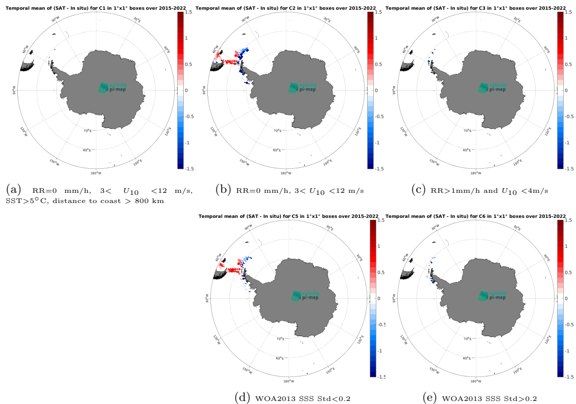
Figure 14: Temporal mean gridded over spatial boxes of size 1^\circ \times 1^\circ of \Delta SSS (SMAP SSS L3 v5.0 - Monthly (JPL) - TSG (CSIC-UTM)) for 5 different subdatasets corresponding to:RR=0 mm/h, 3 < U_{10} < 12 m/s, SST > 5^\circ\text{C} , distance to coast > 800 km (a), RR=0 mm/h, 3 < U_{10} < 12 m/s (b), RR > 1 mm/h and U_{10} < 4 m/s (c), WOA2013 SSS Std < 0.2 (d), WOA2013 SSS Std > 0.2 (e).
