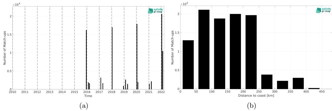
Figure 2: Number of match-ups between TSG (CSIC-UTM) and SMAP SSS L3 v5.0 - Monthly (JPL) SSS as a function of time (a) and as function of the distance to coast (b) over the Southern Ocean Pi-MEP region and for the full satellite product period.
