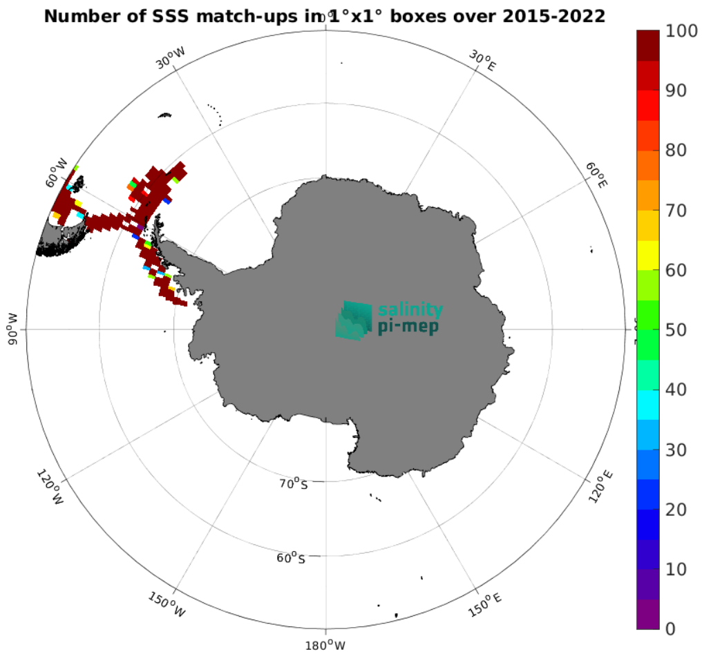
Figure 5: Number of SSS match-ups between TSG (CSIC-UTM) SSS and the SMAP SSS L3 v5.0 - Monthly (JPL) SSS product for the Southern Ocean Pi-MEP region over 1^\circ \times 1^\circ boxes and for the full satellite product period.
