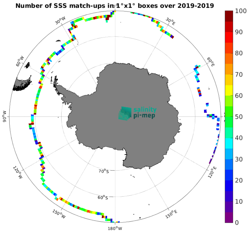
Figure 5: Number of SSS match-ups between Saildrone SSS and the SMAP SSS L3 v5.0 - Monthly (JPL) SSS product for the Southern Ocean Pi-MEP region over 1^\circ \times 1^\circ boxes and for the full satellite product period.
