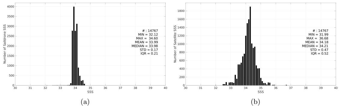
Figure 3: Histograms of SSS from Saildrone (a) and SMAP SSS L3 v5.0 - Monthly (JPL) (b) considering all match-up pairs per bins of 0.1 over the Southern Ocean Pi-MEP region and for the full satellite product period.
