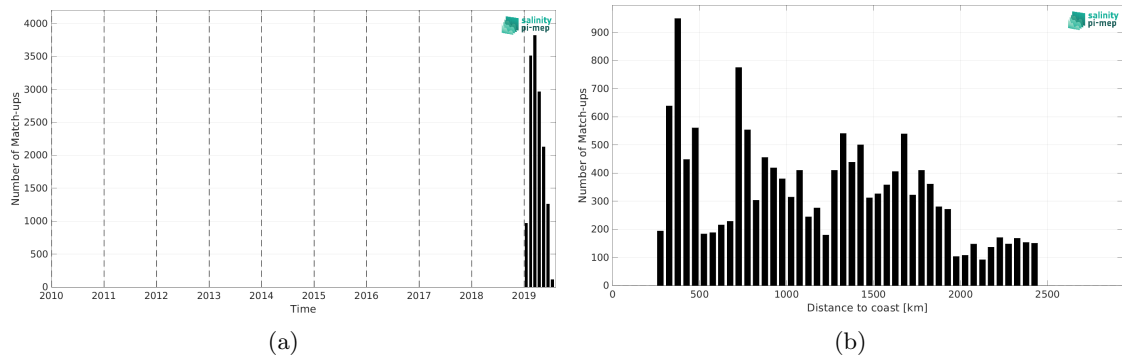
Figure 2: Number of match-ups between Saildrone and SMAP SSS L3 v5.0 - Monthly (JPL) SSS as a function of time (a) and as function of the distance to coast (b) over the Southern Ocean Pi-MEP region and for the full satellite product period.
