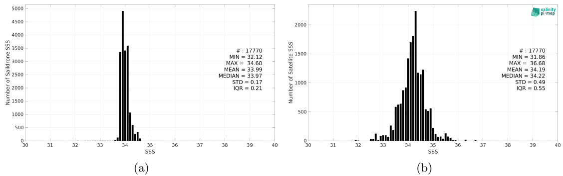
Figure 2: Histograms of SSS from Saildrone (a) and SMAP SSS L3 v5.0 - Monthly (JPL) (b) considering all match-up pairs per bins of 0.1 over the Southern Ocean Pi-MEP region and for the full satellite product period.
