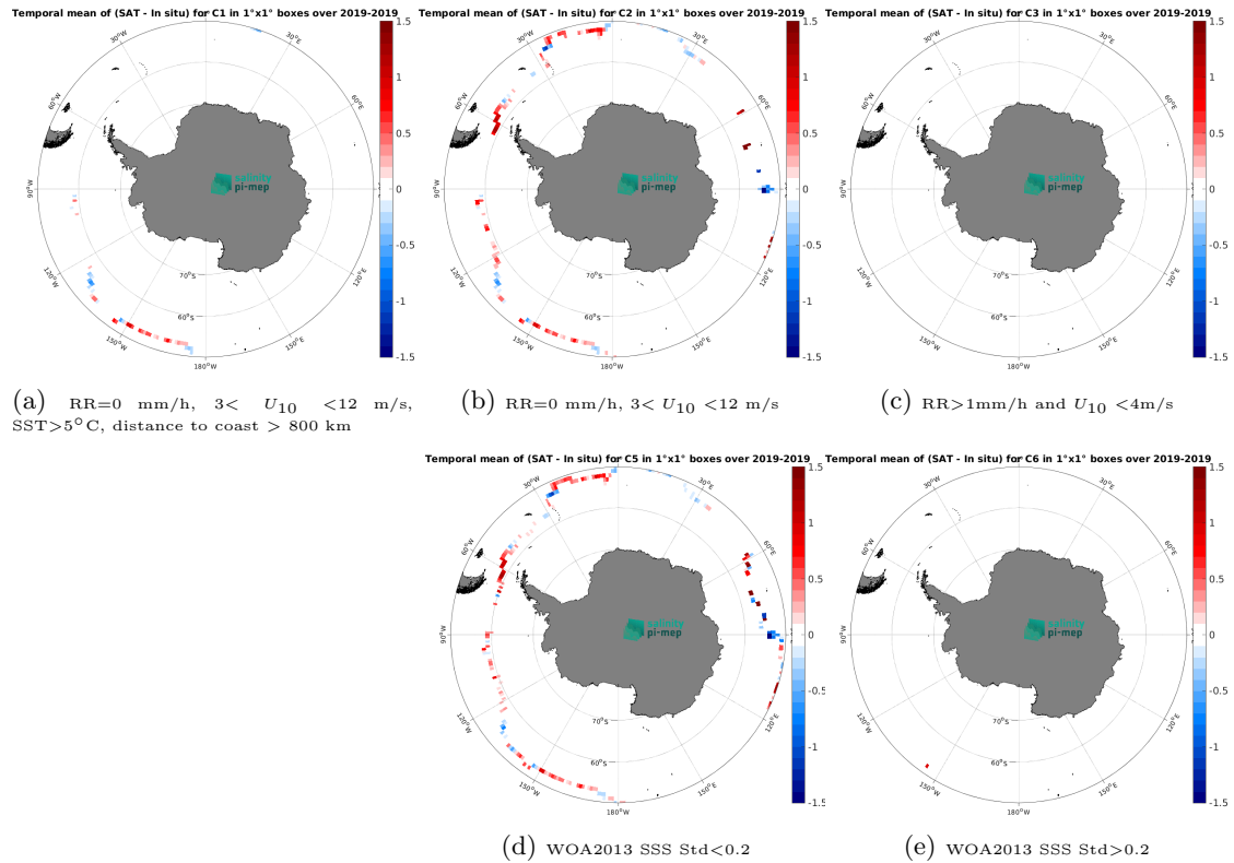
Figure 12: Temporal mean gridded over spatial boxes of size 1^{\circ}\times 1^{\circ} of \Delta\text{SSS} (SMAP SSS L3 v5.0 - Monthly (JPL) - Saildrone) for 5 different subdatasets corresponding to:RR=0 mm/h, 3 < U_{10} < 12 m/s, SST > 5^{\circ}\text{C} , distance to coast > 800 km (a), RR=0 mm/h, 3 < U_{10} < 12 m/s (b), RR > 1 mm/h and U_{10} < 4 m/s (c), WOA2013 SSS Std < 0.2 (d), WOA2013 SSS Std > 0.2 (e).
