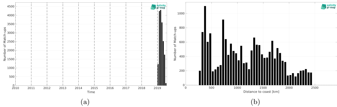
Figure 1: Number of match-ups between Saildrone and SMAP SSS L3 v5.0 - Monthly (JPL) SSS as a function of time (a) and as function of the distance to coast (b) over the Southern Ocean Pi-MEP region and for the full satellite product period.
