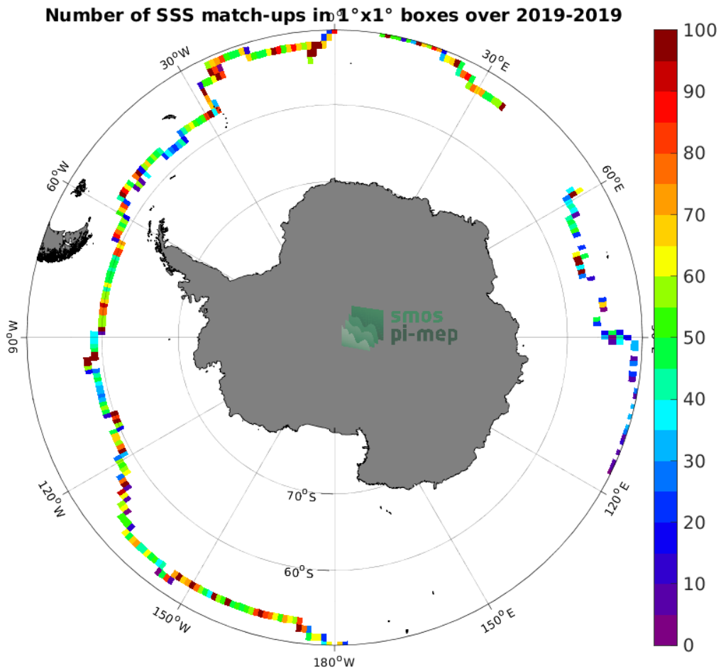
Figure 4: Number of SSS match-ups between Saildrone SSS and the SMAP SSS L3 v5.0 - Monthly (JPL) SSS product for the Southern Ocean Pi-MEP region over 1^\circ \times 1^\circ boxes and for the full satellite product period.
