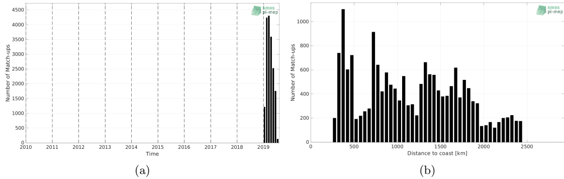
Figure 1: Number of match-ups between Sairdrone and SMAP SSS L3 v5.0 - Monthly (JPL) SSS as a function of time (a) and as function of the distance to coast (b) over the Southern Ocean Pi-MEP region and for the full satellite product period.
