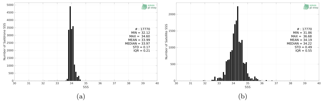
Figure 2: Histograms of SSS from Sairdrone (a) and SMAP SSS L3 v5.0 - Monthly (JPL) (b) considering all match-up pairs per bins of 0.1 over the Southern Ocean Pi-MEP region and for the full satellite product period.
