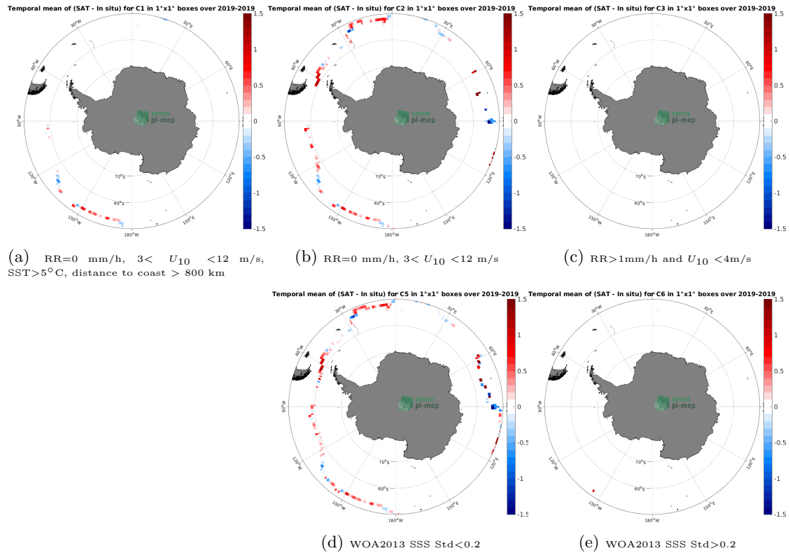
Figure 12: Temporal mean gridded over spatial boxes of size 1^{\circ}\times 1^{\circ} of \Delta\text{SSS} (SMAP SSS L3 v5.0 - Monthly (JPL) - Saikrone) for 5 different subdatasets corresponding to:RR=0 mm/h, 3 < U_{10} < 12 m/s, SST >5^{\circ}\text{C} , distance to coast > 800 km (a), RR=0 mm/h, 3 < U_{10} < 12 m/s (b), RR >1 mm/h and U_{10} < 4 m/s (c), WOA2013 SSS Std <0.2 (d), WOA2013 SSS Std >0.2 (e).
