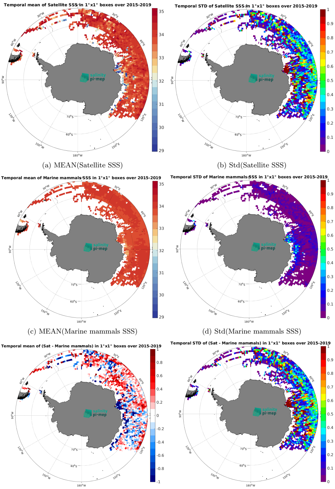
(e) MEAN( \Delta SSS) (Satellite - Marine mammals) 17 (f) Std( \Delta SSS) (Satellite - Marine mammals) Figure 6: Temporal mean (left) and Std (right) of SSS from SMAP SSS L3 v5.0 - Monthly (JPL) (top), Marine mammals (middle), and of \Delta SSS (Satellite - Marine mammals). Only match-up pairs are used to generate these maps.
