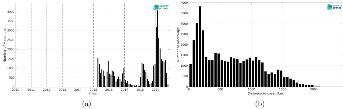
Figure 1: Number of match-ups between Marine mammals and SMAP SSS L3 v5.0 - Monthly (JPL) SSS as a function of time (a) and as function of the distance to coast (b) over the Southern Ocean Pi-MEP region and for the full satellite product period.
