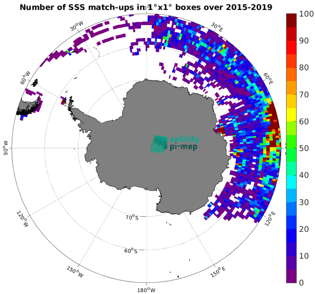
Figure 4: Number of SSS match-ups between Marine mammals SSS and the SMAP SSS L3 v5.0 - Monthly (JPL) SSS product for the Southern Ocean Pi-MEP region over 1^\circ \times 1^\circ boxes and for the full satellite product period.
