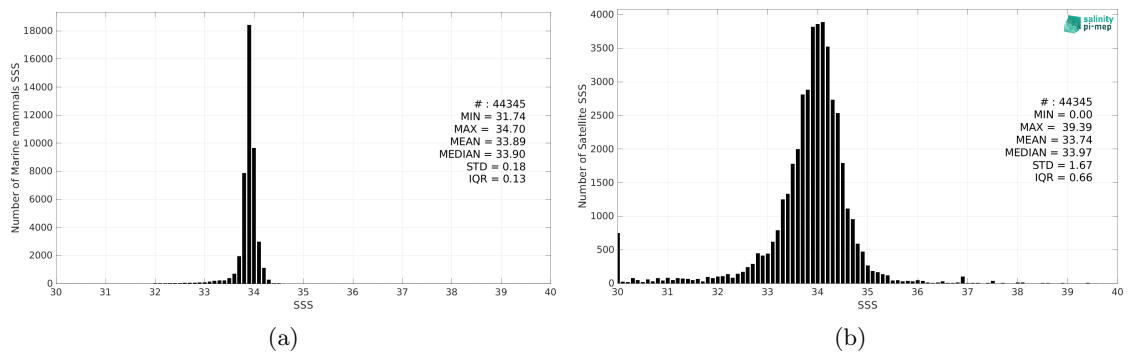
Figure 2: Histograms of SSS from Marine mammals (a) and SMAP SSS L3 v5.0 - Monthly (JPL) (b) considering all match-up pairs per bins of 0.1 over the Southern Ocean Pi-MEP region and for the full satellite product period.
